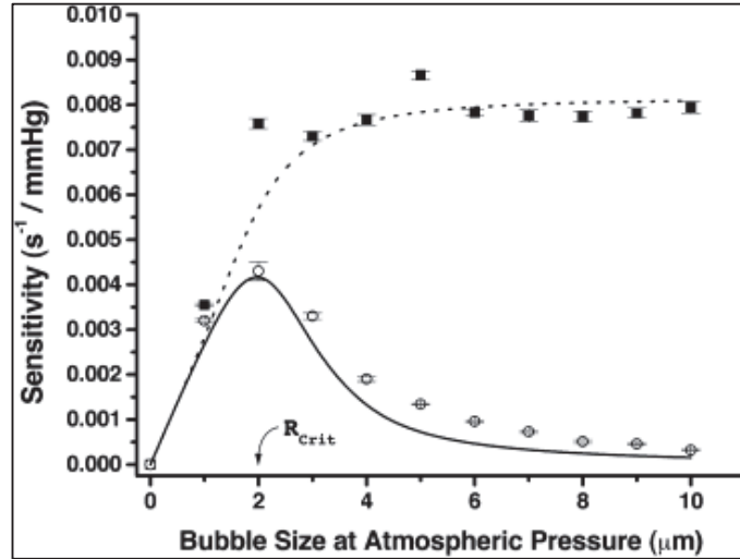
Figure 1.13 – Plot of the relation of the bubble size with the pressure sensitivity of both R_2^* and R_2^{\text{eff}} . The black square and the open circle, respectively, indicate R_2^* and R_2^{\text{eff}} simulations, while the dotted line and the solid line, respectively, represent R_2^* and R_2^{\text{eff}} theory (Dharmakumar, Plewes et al. 2002).
