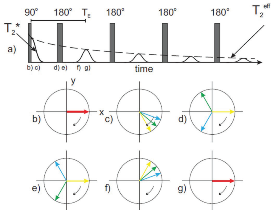
Figure 1.3 – Diagram showing the formation of a spin echo (SE). a) After the 90° RF pulse excitation, a subsequent 180° RF pulse is applied to refocus the spin and thus, the SE signal is formed after a delay of time, T_E . b) Magnetisation after tipping into transverse plane, c) Dephasing magnetisation, d) Dephased magnetisation, e) System after application of refocusing pulse along x, f) Magnetisation near beginning of echo envelope, g) Magnetisation at the echo time after the initial pulse. Red arrow is all magnetic moments in phase; yellow, green and blue arrows are, respectively, fast, medium and slowly dephasing magnetic moments. Diagram reproduced from Morris, 2009.
