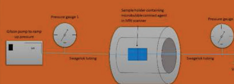
Figure 3 – An illustration showing the equipment set-up for the experiment. A sample holder containing a microbubble contrast agent was connected to a pump by Swagelok tubing. The pressure gauges were placed at both sides of the compartments to measure the pressure changes.
