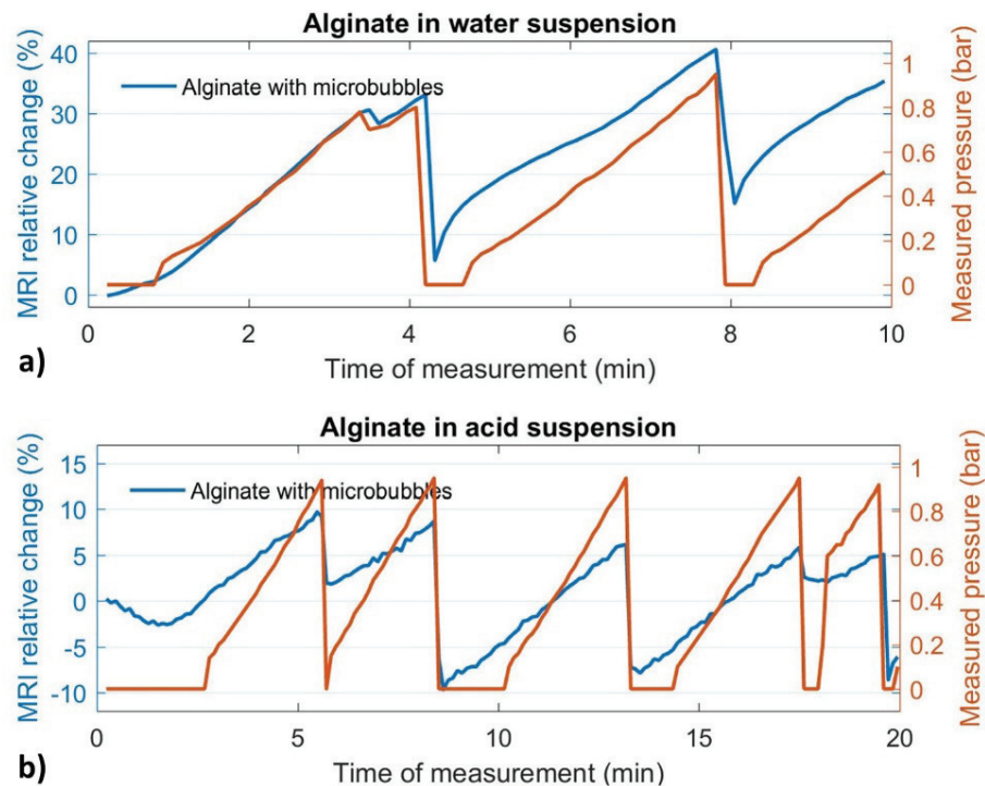
Figure 5.14 – Graphs showing two subsequent experiments measuring the sensitivity of alginate spheres with microbubbles in a) water and b) acid simulating gastric solution. The MRI relative change is calculated by comparing the signal intensity with the start of the image acquisition and the pressure cycling (pressure 0 bar). The red curve shows the measured pressure.
