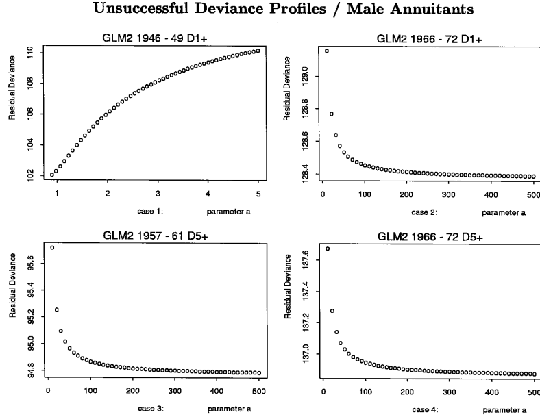
Figure 11: Difficulty with the non-linear parameter in (GLM2) fitting, either \min(a) < \max(\mu_x) or Dev \rightarrow \min only if a \rightarrow \infty .
