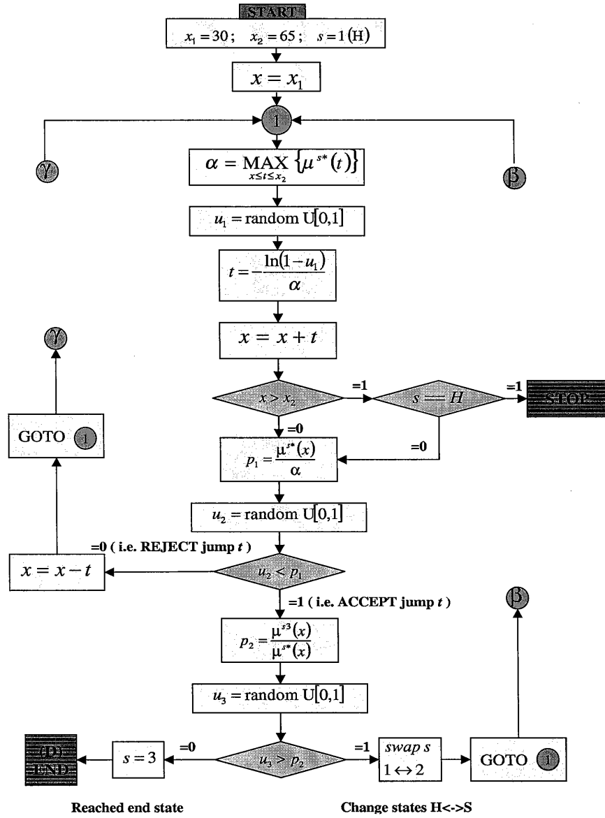
Figure 1: Logical Scheme of Simulation with Thinning.
