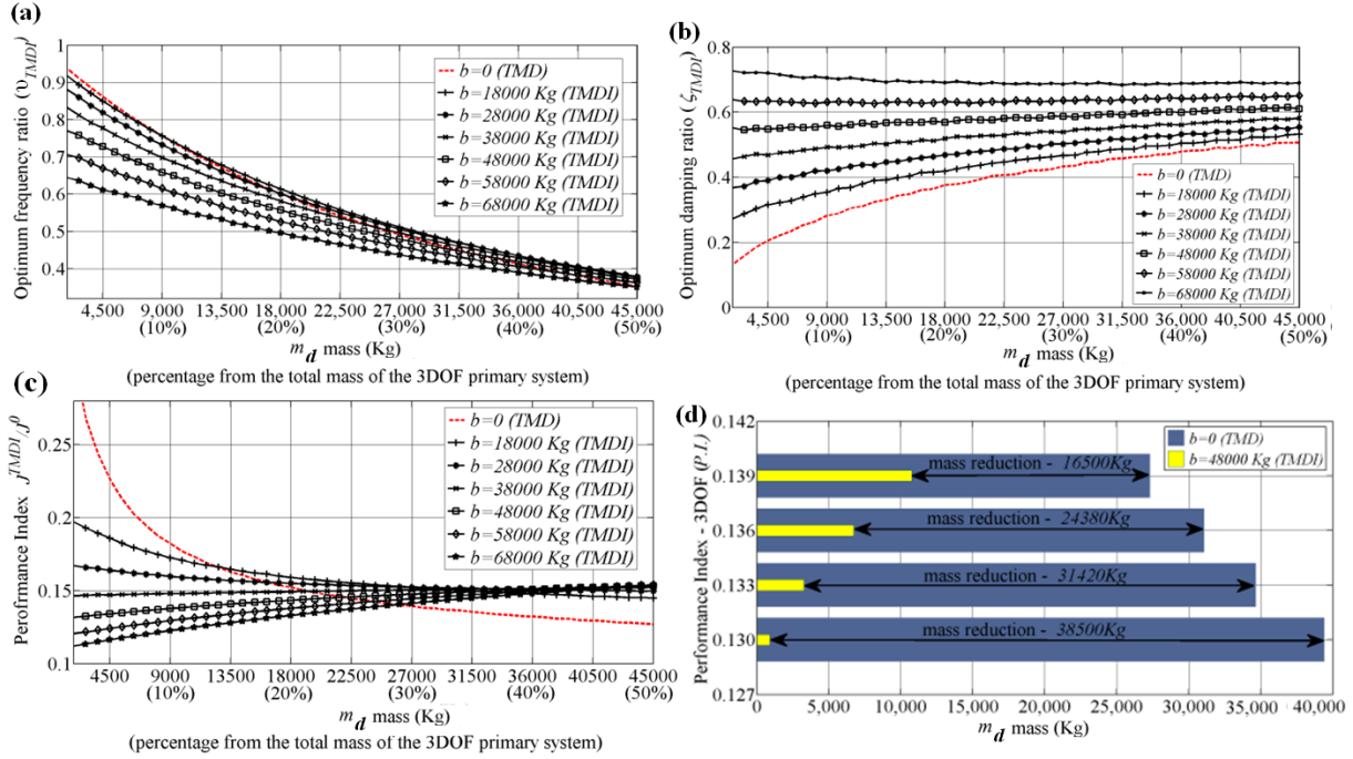
Figure 3: (a) Optimum frequency ratio; (b) Optimum damping ratio; (c) Performance index; (d) mass reduction for a given performance index, for various values of inerter b and attached mass m_d .
