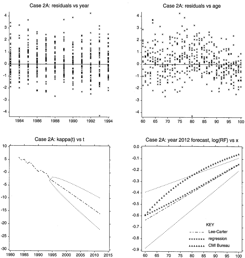
Fig. 7. RF for q_x , specific residuals, \kappa_t , forecasts
