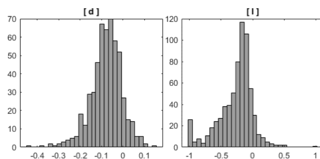
Figure 4: Example histograms of the asymmetry index I_{as} .
