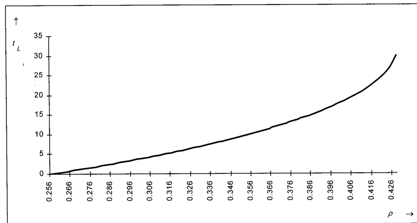
Figure 4: Optimal values of t_L as a function of \rho .
