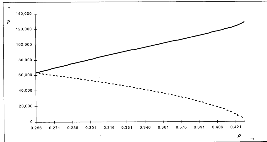
Figure 3: Optimal values for P_L (dotted) and P_H (solid) as a function of \rho .
