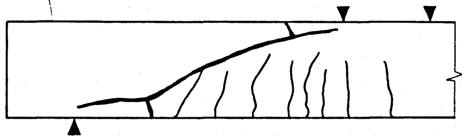
beam 17
