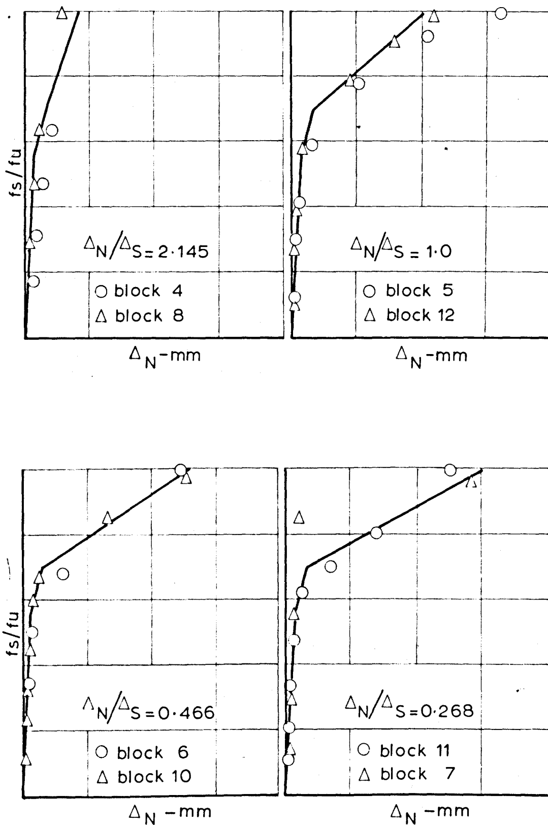
FIG. 6.13 TEST RESULTS, SERIES 3: SHEAR STRESS - DISPLACEMENT PLOTS
