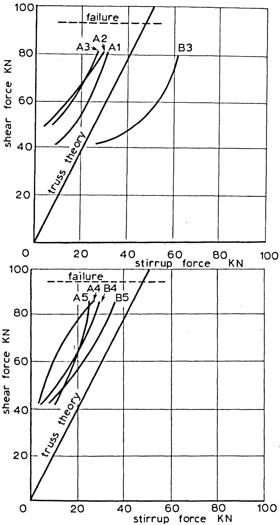
FIG.8.6 STIRRUP FORCE CARRIED IN BEAM 62/1
