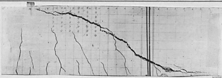
Fig. 4.8 Crack patterns at failure
