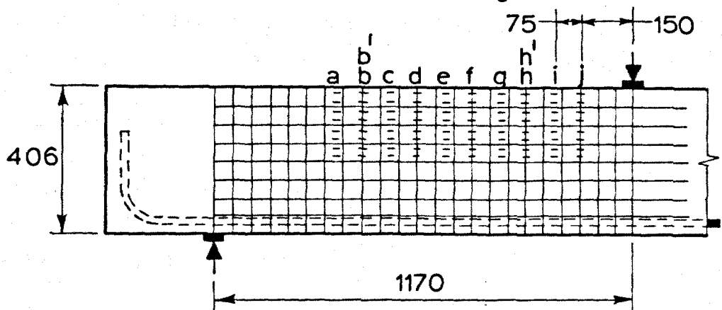
Beam 8
