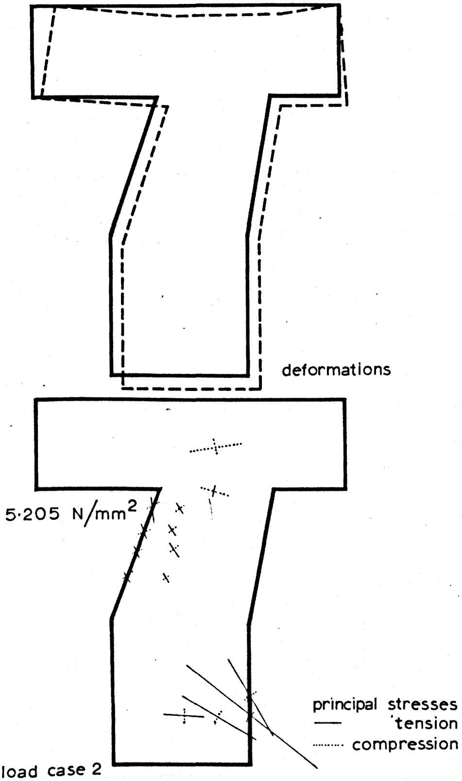
FIG.A.4 RESULTS OF SINGLE CANTILEVER ANALYSIS, LOAD CASE 2
