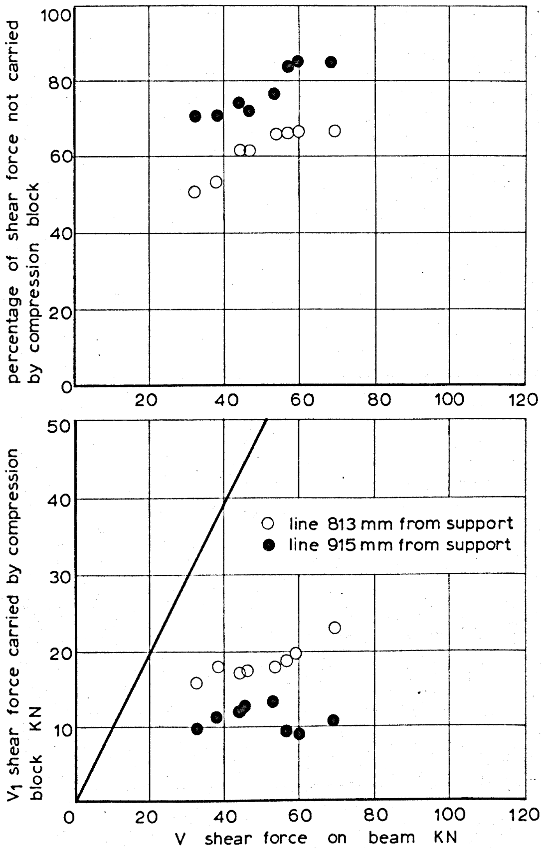
FIG 4.12 TEST RESULTS — BEAM I
