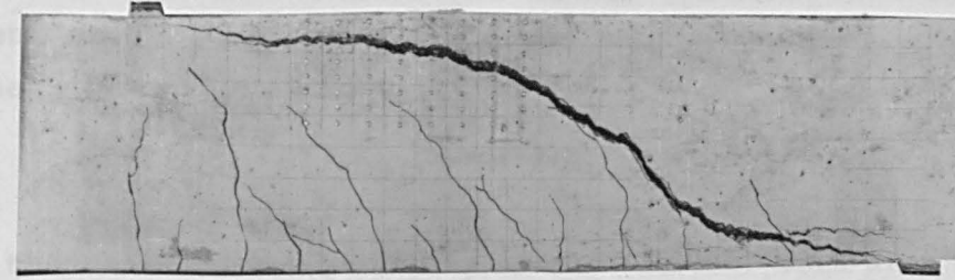
Fig 4.11 Crack patterns at failure Second test Beam 6
