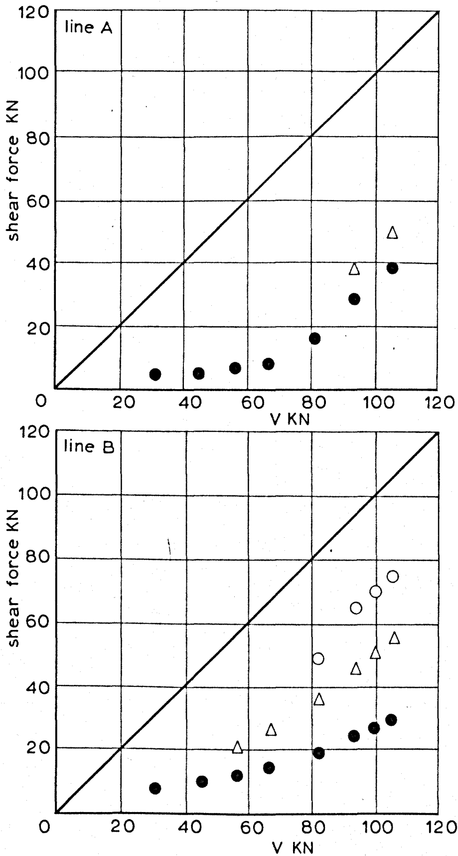
FIG.8.12 DISTRIBUTION OF SHEAR FORCE IN BEAM 12
