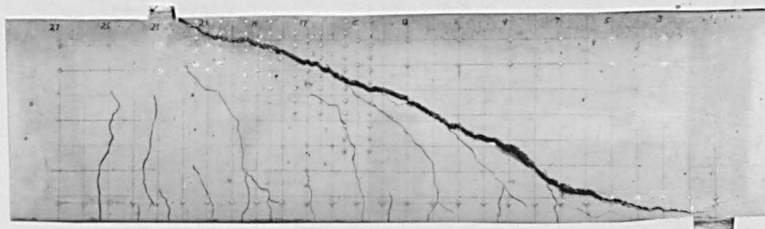
Fig 4.7 Crack patterns at failure Beam 2
