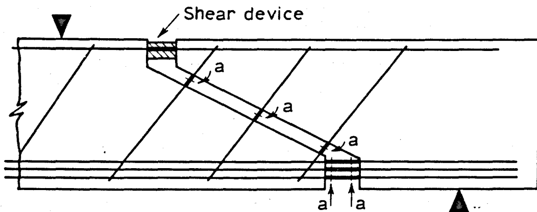
Test beam
