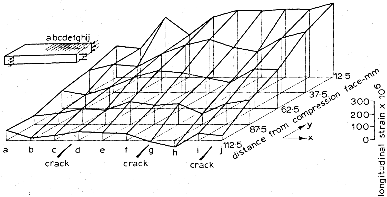
FIG 4.21 MEASURED STRAINS ON BEAM 9 AT LOAD STAGE 11
