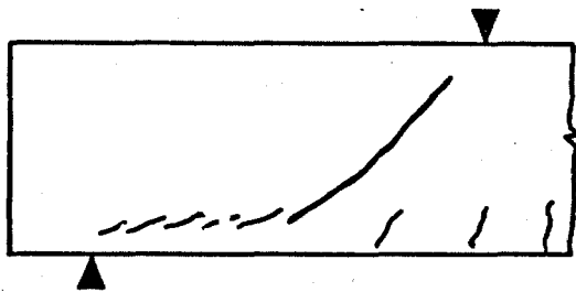
Shear bond
