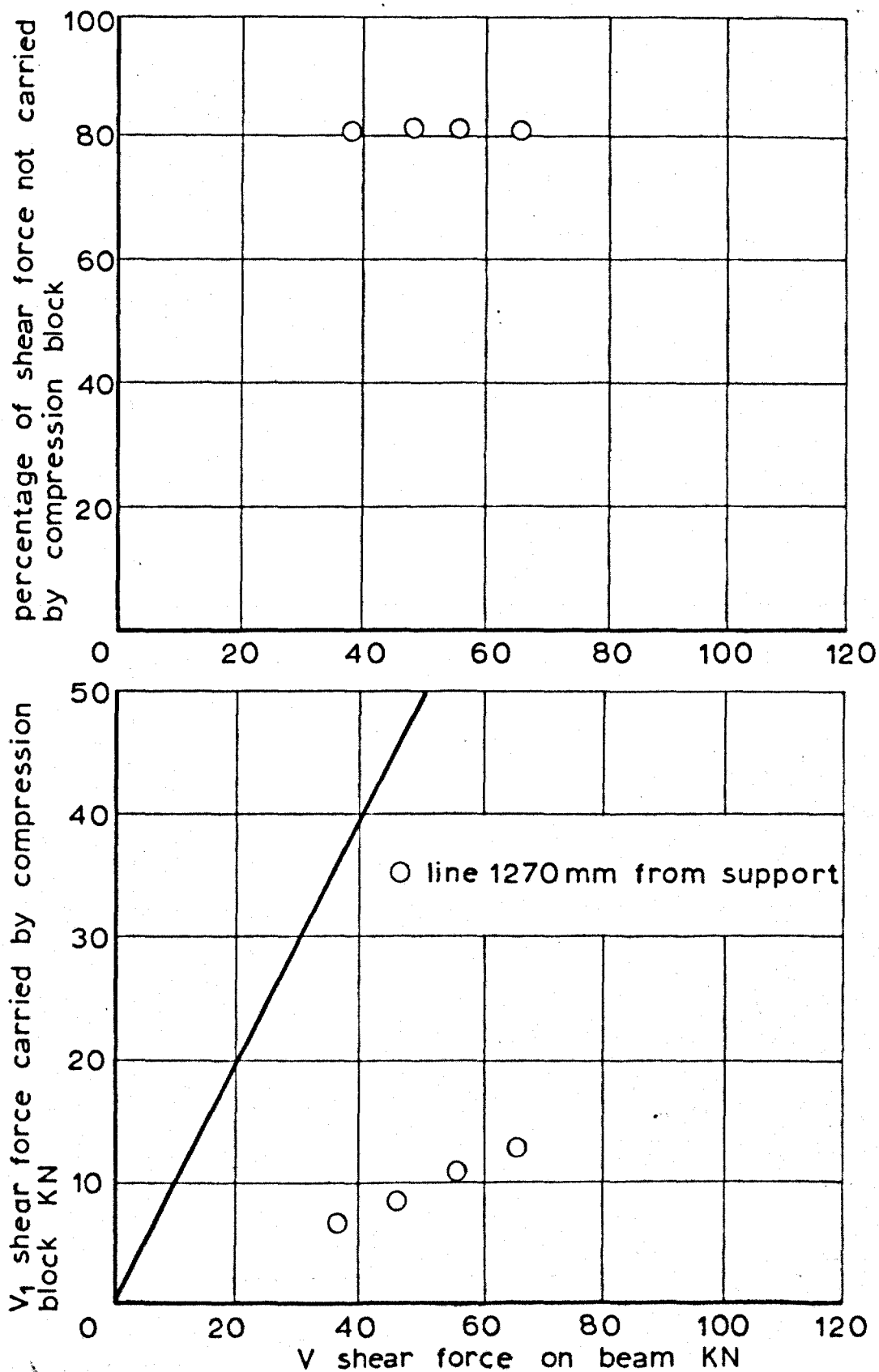
FIG. 4.15 TEST RESULTS BEAM 4
