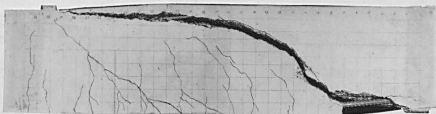
Beam 3
