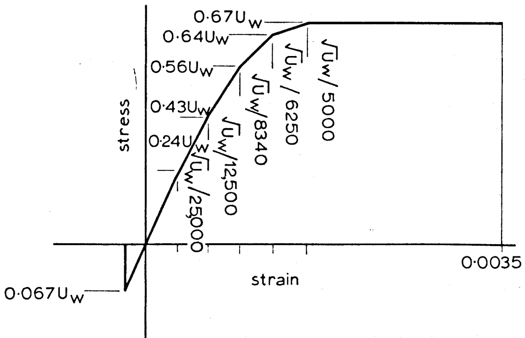
(a) concrete
