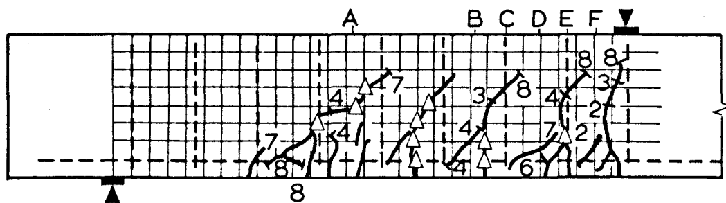
beam 11
