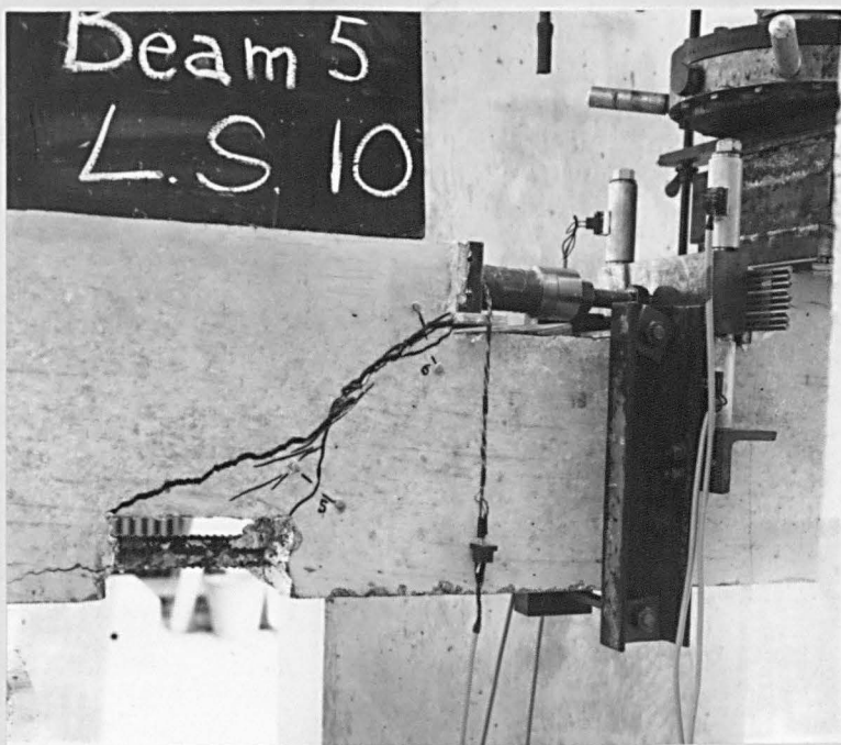
FIG. 6.24 Preformed crack on beam D5 at finish of test
