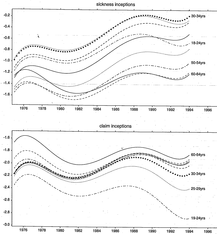
Log predicted inception intensities vs period, by age, DP1 Figure 5.1(a)
