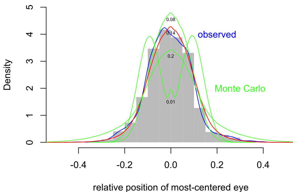
Fig 3. Densities of the simulated distributions of the most-centered-eye. Monte Carlo simulations in green and red (see text) plotted at four representative values of the standard deviation, \sigma (small numbers in black). The density (blue) of the observed distribution (histogram in grey) is plotted for comparison.
