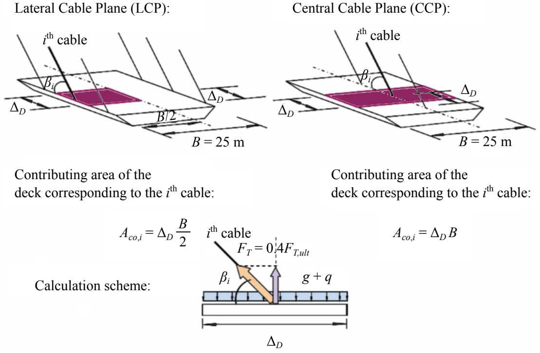
Figure 3.9: Contributing areas of the deck associated with each cable and calculation scheme to obtain their load, both in LCP and CCP models. Dimensions in [m] ( taken from Camara (2011) ).
