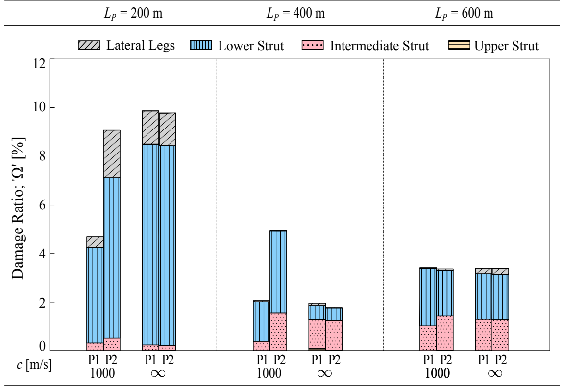
Figure 7.16: Average values for the damage factor \Omega (%) at the end of the records in the individual components of pylons P1 and P2 when c = 1000 and \infty m/s. H-LCP model; L_P = 200, 400 and 600 m, respectively. \theta = 0^\circ .
