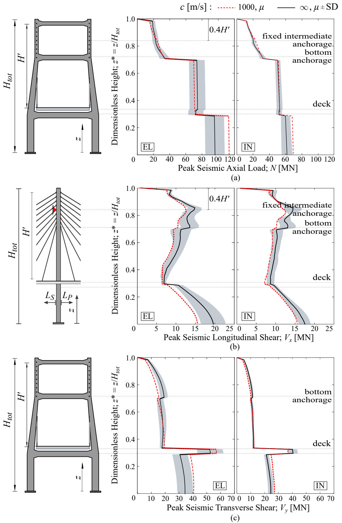
Figure 7.3: Peak elastic (left column) and inelastic (right column) seismic response in pylon P2. H-LCP bridge; L_P = 400 m; \theta = 0^\circ (i.e. FN // bridge axis).
