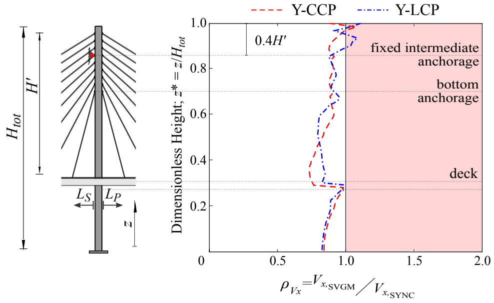
Figure 6.13: Longitudinal response ratio \rho_{V_x} in pylon P2 of the Y-CCP and Y-LCP models. L_P = 400 m, \theta = 0^\circ . The red band denotes \rho_{V_x} > 1.0 for which the SVGM increases the seismic response.
