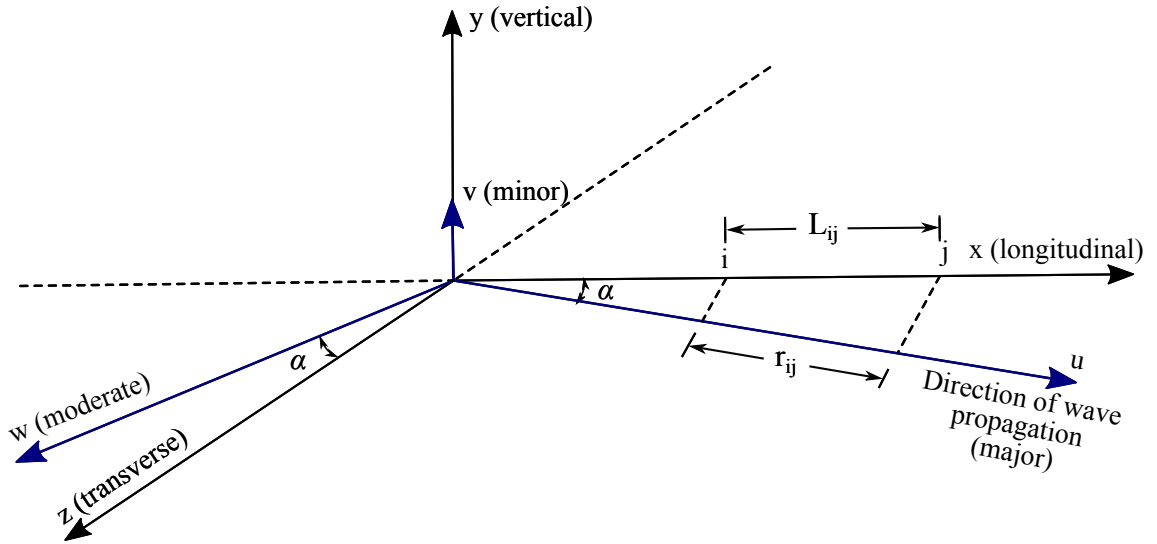
Figure 2.11: Principal axes of the 335-m span cable-stayed bridge (x, y, z) and the principal directions of the ground motion (u, v, w); \alpha is the incidence angle of the seismic waves (taken from Allam and Datta (2004)).
