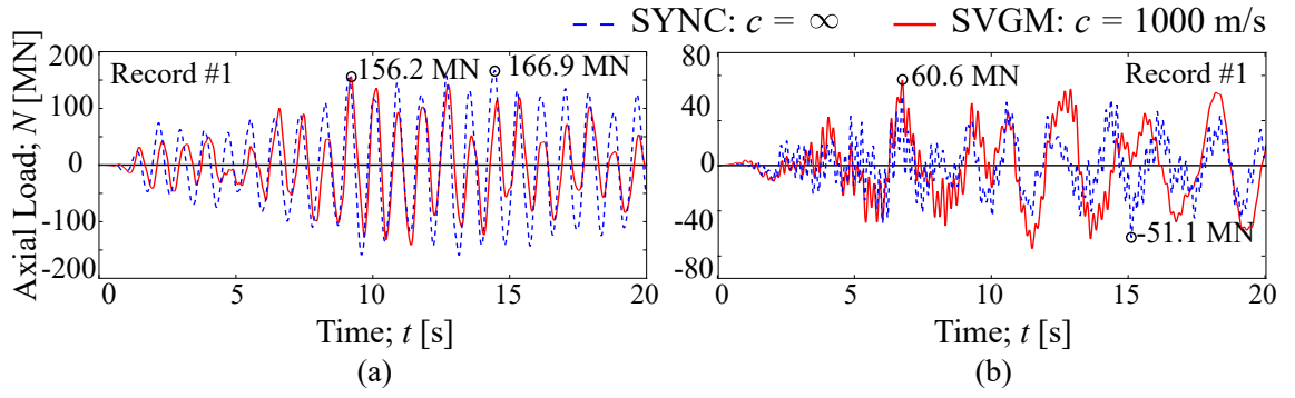
Figure 6.15: Time-history response of the seismic axial force ( N ) at the base of pylon P1 in the models: (a) Y-CCP, (b) YD-CCP. Results for record #1, \theta = 0^\circ , L_P = 400 m. The peak responses are annotated.
