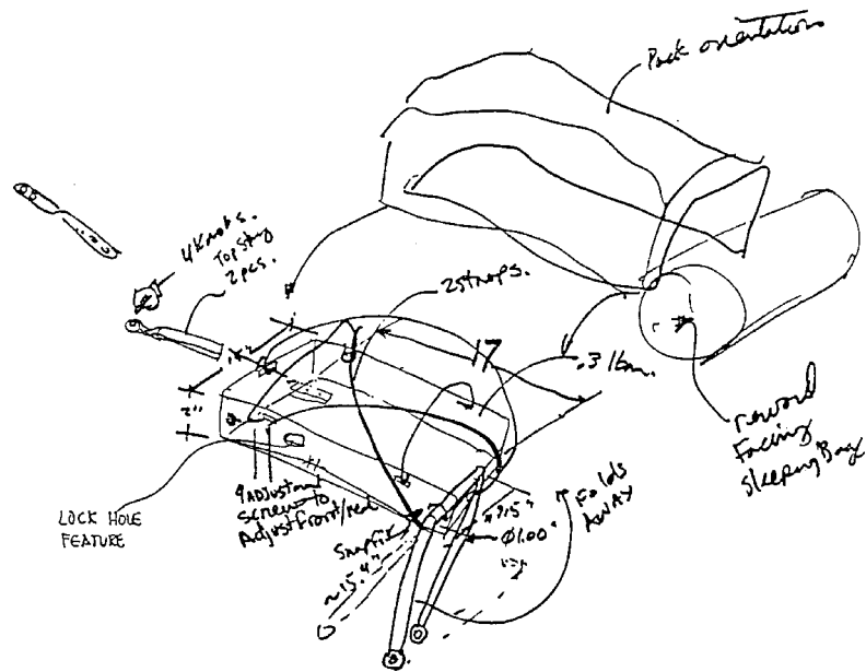
Figure 4.12 – The team’s drawing of their final design concept
