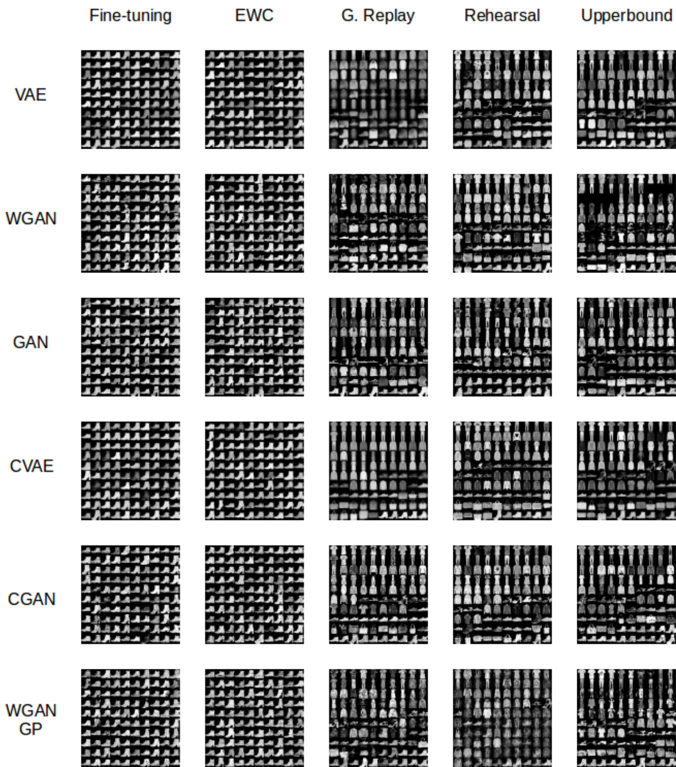
Fig. 15: Fashion MNIST samples for each generative model and each Continual Learning strategy, at the end of training on 10 sequential tasks. The goal is to produce samples from all categories.
