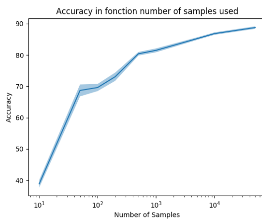
(b) fashion-MNIST Classifier accuracy
