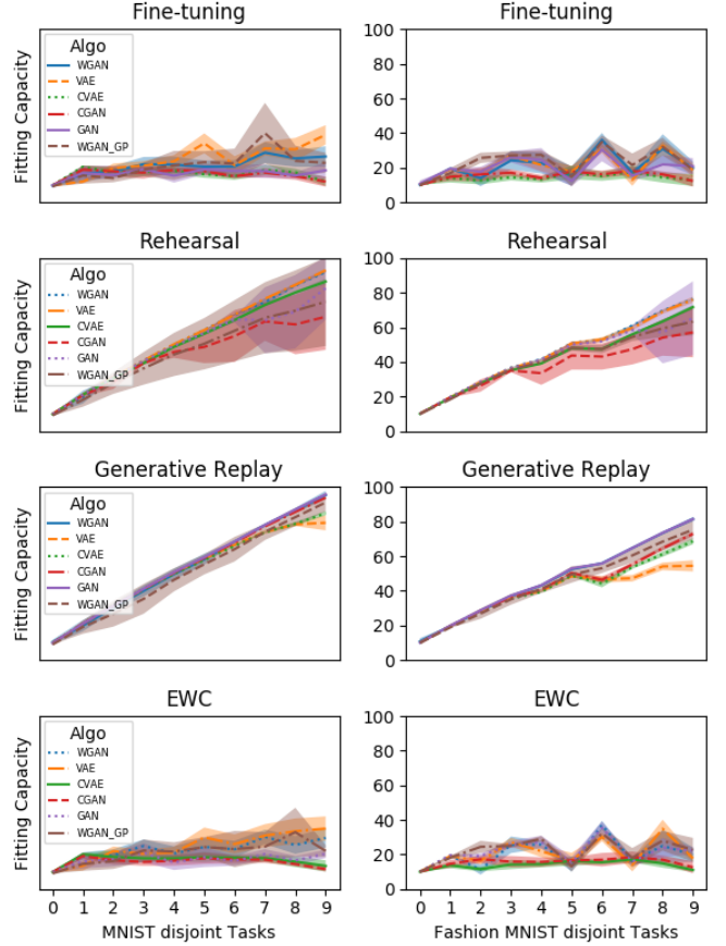
Fig. 3: Means and standard deviations over 8 seeds of Fitting Capacity metric evaluation of VAE, CVAE, GAN, CGAN and WGAN. The four considered CL strategies are: Fine Tuning, Generative Replay, Rehearsal and EWC. The setting is 10 disjoint tasks on MNIST and Fashion MNIST.
