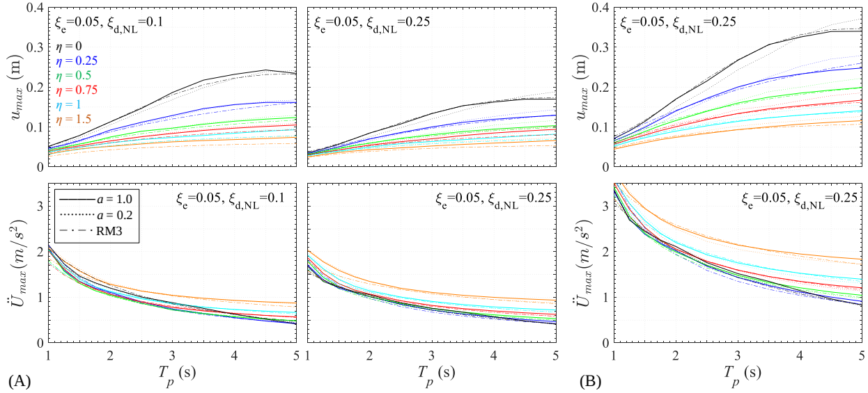
Figure 11 NLRHA response u_{\max} and \ddot{u}_{\max} under Art B considering energy-equivalent dampers of a=1, 0.2 , compared to RM3 predicted response for PGA of (A) 0.21g ( T_R=475 yrs), and (B) 0.42g ( T_R \approx 2500 yrs) at bedrock, \zeta=15, 30\% , \eta=0 \sim 1.5
