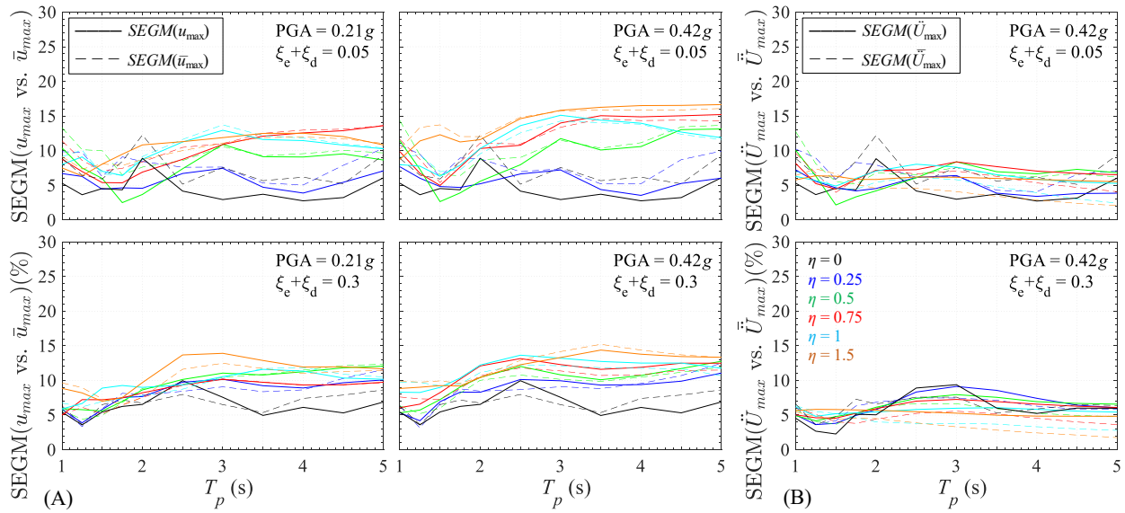
Figure 5 NLRHA results under Art B suite: SEGM (%) for (A) u_{\max} , \bar{u}_{\max} , and (B) \dot{U}_{\max} , \ddot{U}_{\max} , for PGAs of 0.21g ( T_R=475 yrs, \gamma_{EQ}=1 ), 0.42g ( T_R\approx 2500 yrs, \gamma_{EQ}=2 ) at bedrock, \xi=5 , 30%, and \eta=0\sim 1.5
