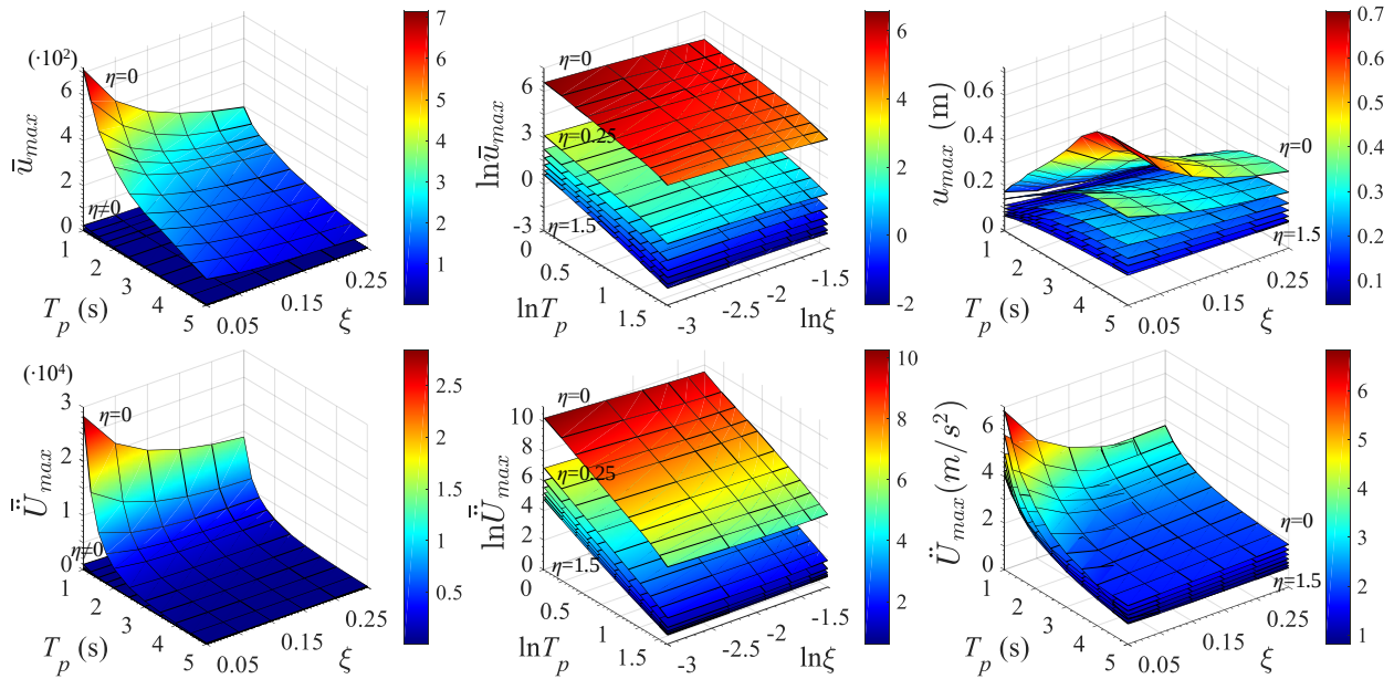
Figure 4 NLRHA results under Art B suite: GMs of \bar{u}_{\max} , \bar{U}_{\max} , \ln \bar{u}_{\max} , \ln \bar{U}_{\max} , u_{\max} , \ddot{U}_{\max} for PGA of 0.42g ( T_R \approx 2500 yrs, \gamma_{EQ} = 2 ) at bedrock
