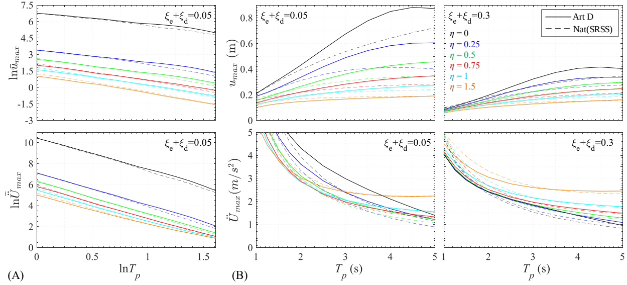
Figure 12 NLRHA results under Art D, Nat(SRSS) ( \gamma_{EC8}=1 ) suites: GM of (A) \ln \bar{u}_{\max} , \ln \ddot{U}_{\max} , and (B) u_{\max} , \ddot{U}_{\max} , for PGA=0.42g ( T_R \approx 2500 yrs, \gamma_{EQ}=2 ) at bedrock, \xi=5, 30\% , and \eta=0 \sim 1.5
