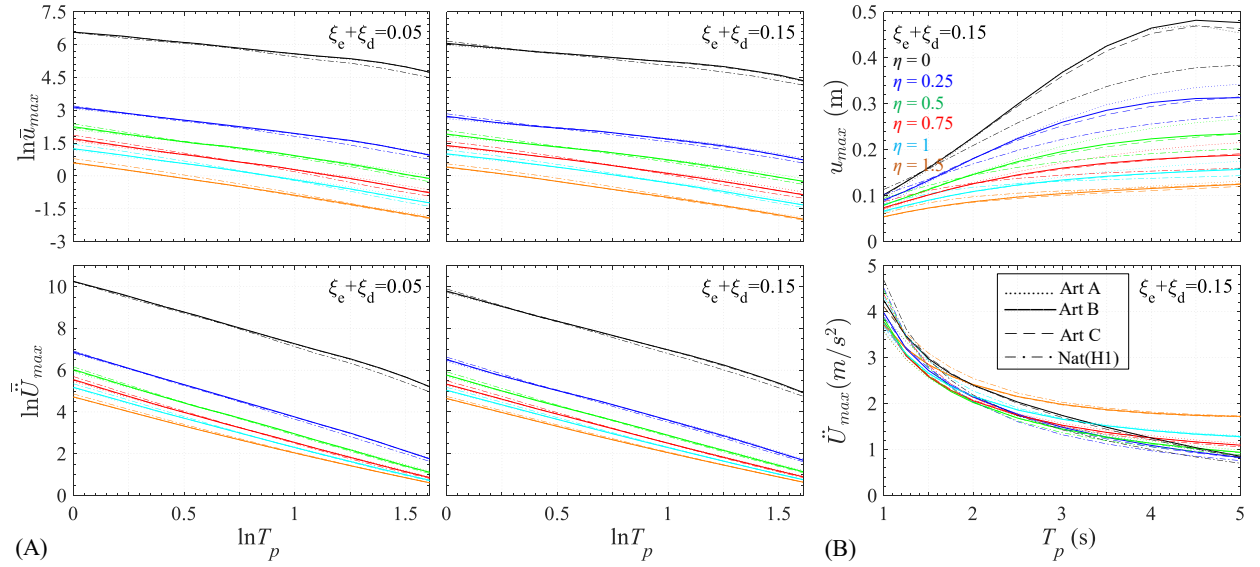
Figure 7 NLRHA results under Art A, Art B, Art C, Nat(H1) ( \gamma_{ECB}=1 ): GM of (A) \ln \bar{u}_{max} , \ln \bar{U}_{max} , and (B) u_{max} , \bar{U}_{max} for PGA of 0.42g ( T_R \approx 2500 yrs, \gamma_{EQ}=2 ) at bedrock, \zeta=5, 15\% , and \eta=0 \sim 1.5
