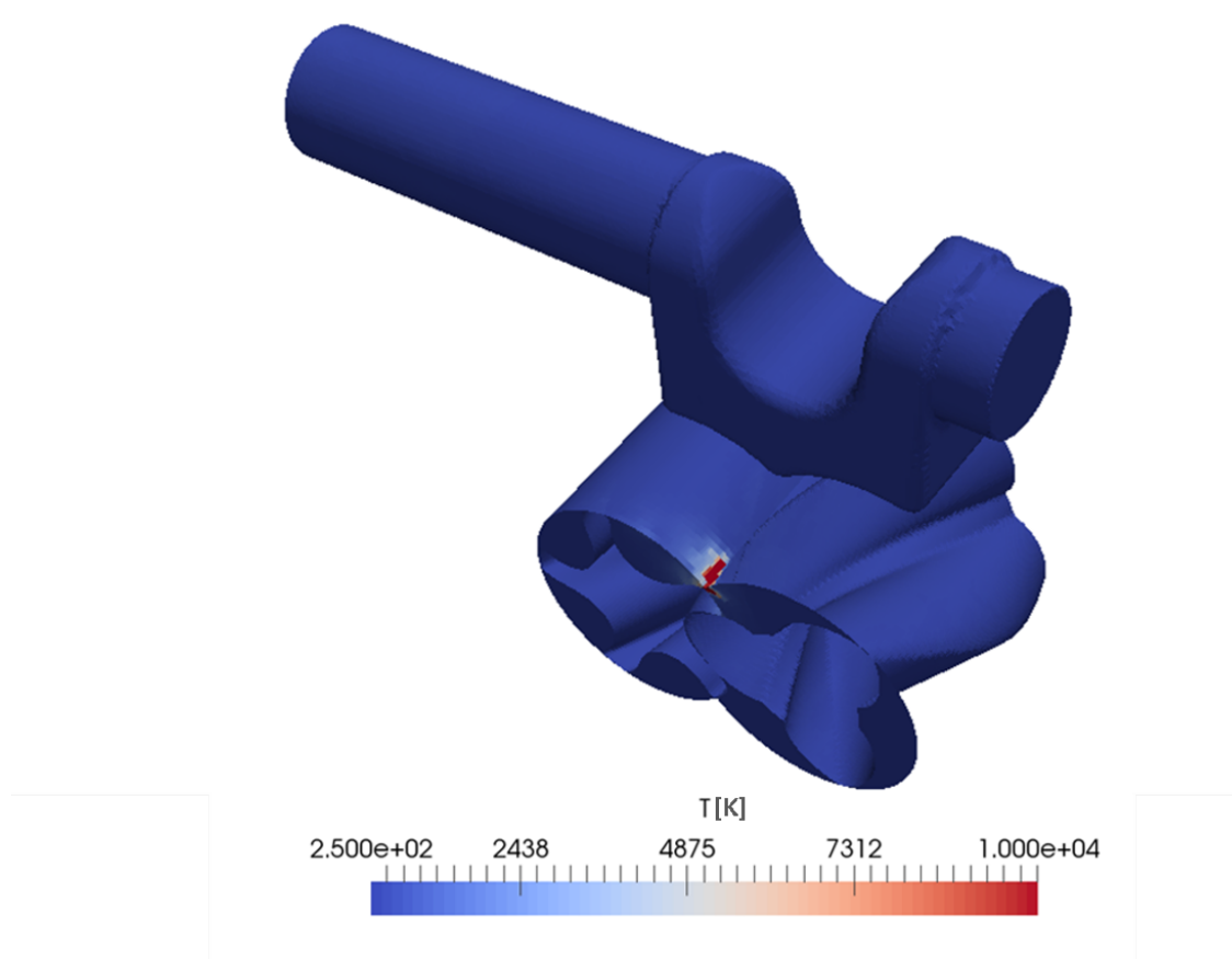
Figure 5. Temperature spike originated in the gap between thread head and casing on the female rotor
