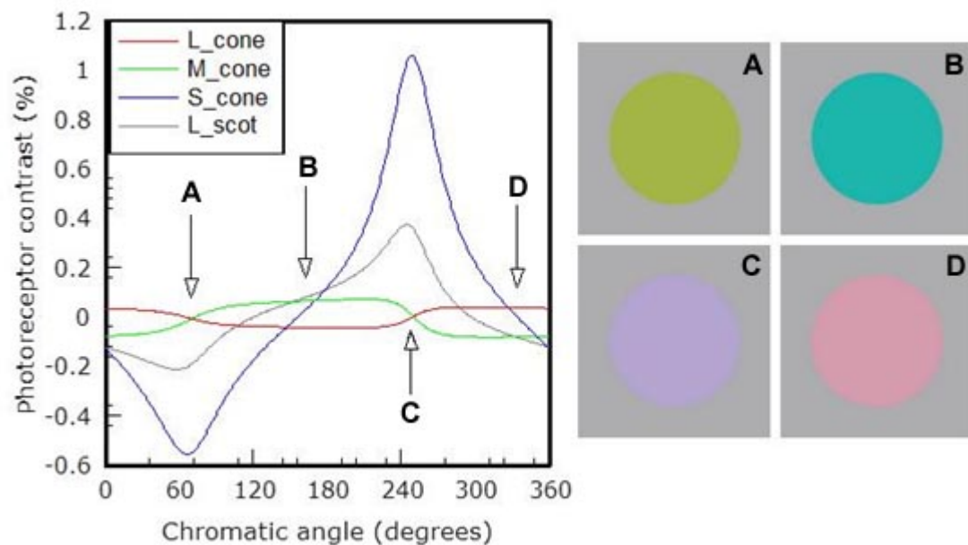
Figure 4-17. The graph shows selected chromatic displacement angles that have minimum and maximum S-cone contrasts. Examples of the corresponding visual stimuli are also shown – chromatic angle equals 70^\circ (A); 155^\circ (B); 249^\circ (C) and 335^\circ (D).
