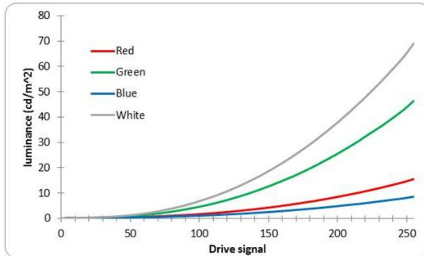
Figure 3-9. luminance calibration for each phorsphor gun. Driven signal from 0 to 255. The real calibration process employed a interval step of 4 to save time, and the values in between were then interpolated.
