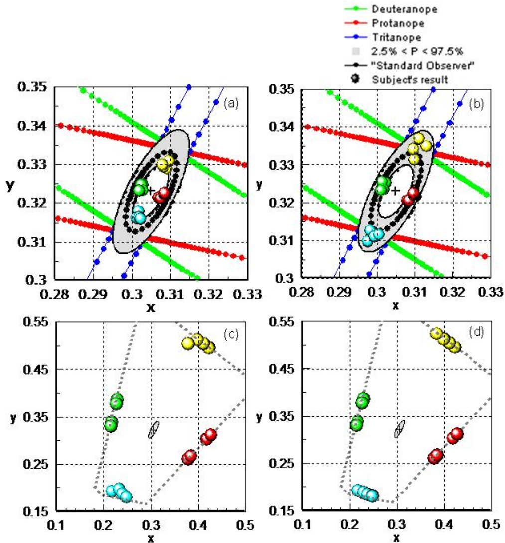
Figure 6-6. CAD test results in the normal trichomat (a), in the mild rod deficient subject (b), in the retinitis pigmentosa subject (c) and in the rod monochromat (d). The colour vision tests are carried out with a background of 26\text{cd/m}^2 . The mild rod deficient subject has excellent colour vision whereas neither the RP subject or the rod monochromat show any sign of colour vision and are unable to see or detect the presence of the colour defined targets even for chromatic saturations that are limited only by the phosphors of the display.
