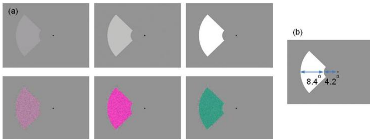
Figure 5-1. (a) Illustration of the visual stimuli designed to isolate luminance and chromatic channels. The chromatic stimuli were buried in RLM noise to minimize the detection of any residual luminance signal. (b) The angle of the sector (section b) subtends 92° and they were presented 4.2° away from fixation, along the horizontal meridian. The uniform background field subtended a visual angle of 30°x24°.
