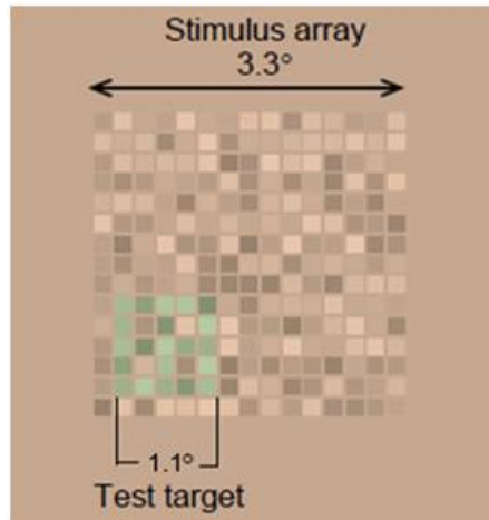
Figure 2-5. An example stimulus from the CAD test.
