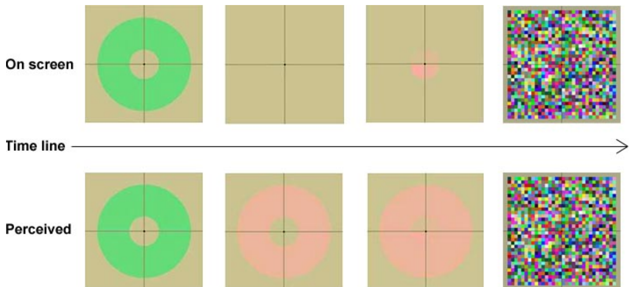
Figure 2-8 A schematic diagram that illustrates the four-alternative forced choice QAA test. The upper show shows the stimulus presentation sequence that is presented on the screen. In a typical QAA test, the reference (adaptation) stimulus is presented for 5s, followed by a blank screen for certain durations according to the gap time. Then the test stimulus is presented. At last, a square patch with random luminance and coloured noise is presented. The bottom row shows an example of perceived images from a trichromat. The trichromat sees the reference stimulus when it is presented on the screen. However, when the reference stimulus is turned off and the blank screen is presented, the subject perceives
