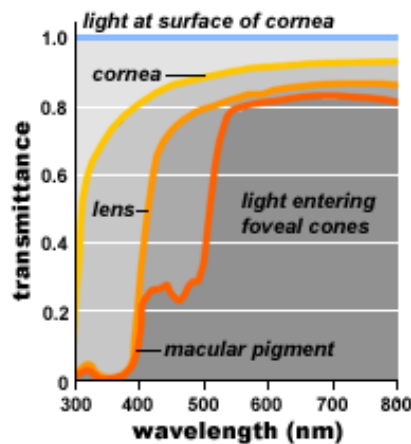
Figure 1-4. Prereceptoral filtering in an adult eye (adapted from Packer & Williams 2003).
