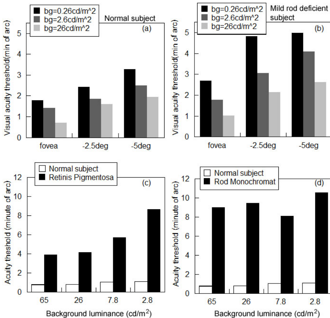
Figure 6-7. Contrast acuity results from a normal subject (a) compared with the mild rod deficient subject (b) measure in the fovea, -2.5^\circ and -5^\circ eccentricity when at 3 different background levels (26, 2.6 and 0.26\text{cd/m}^2 ). The rod monochromat shows similar visual acuity threshold at the fovea when light level is high, but shows a much higher threshold in the periphery especially when light level is low and the rods are more dominate in visual performance. c & d show the contrast acuity results for the RP subject (c) and the rod monochromat (d) measured in the foveal region at each of four different background luminance levels (65, 26, 7.8 and 2.8\text{cd/m}^2 ).
