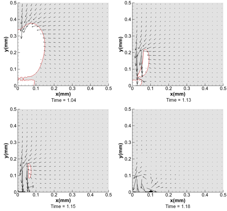
Figure 3.16: Depiction of the supercritical (black), vapour (white) and liquid (grey) regions, combined with velocity vectors for d = 416 \mu m . Time has been non-dimensionalized with \tau = 2.88 \mu s .
