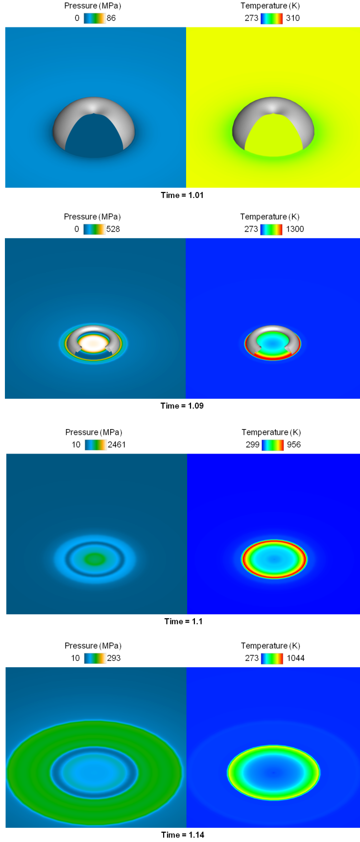
Figure 3.14: Wall pressure and temperature contours combined with bubble iso-surface of \rho = 380 \text{ kg/m}^3 for d = 140 \text{ }\mu\text{m} . Time has been non-dimensionalized with \tau = 2.88 \text{ }\mu\text{s} .
