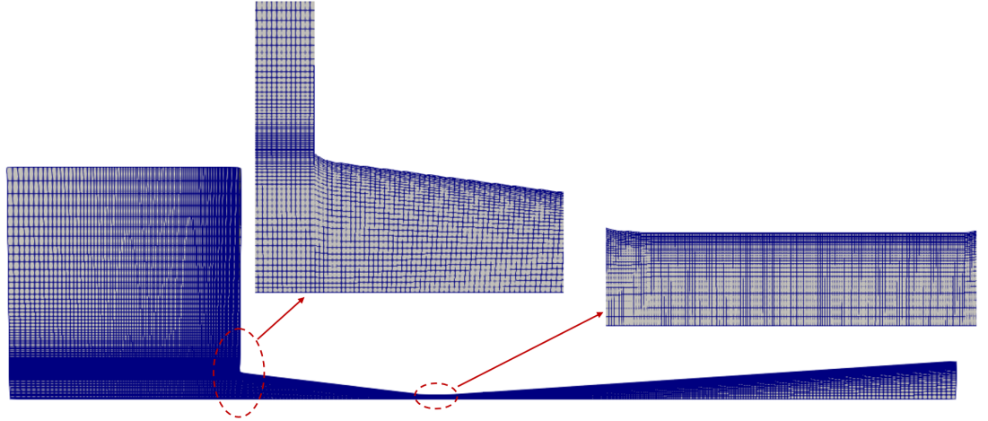
Figure 4.15: Computational grid for the conical nozzle case.
