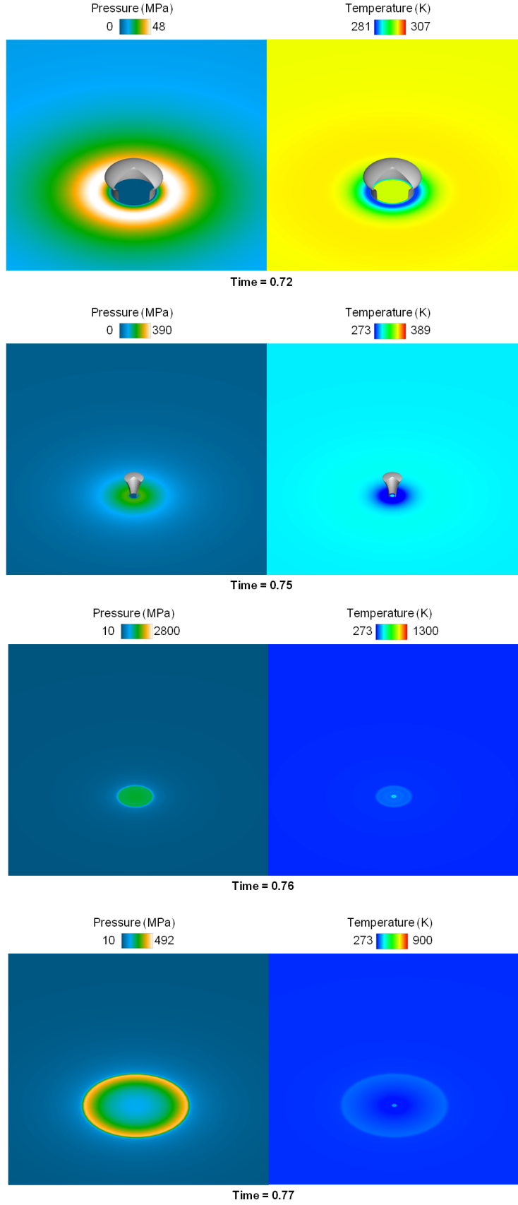
Figure 3.15: Wall pressure and temperature contours combined with bubble iso-surface of \rho = 380 \text{ kg/m}^3 for d = -140 \text{ }\mu\text{m} . Time has been non-dimensionalized with \tau = 2.88 \text{ }\mu\text{s} .
