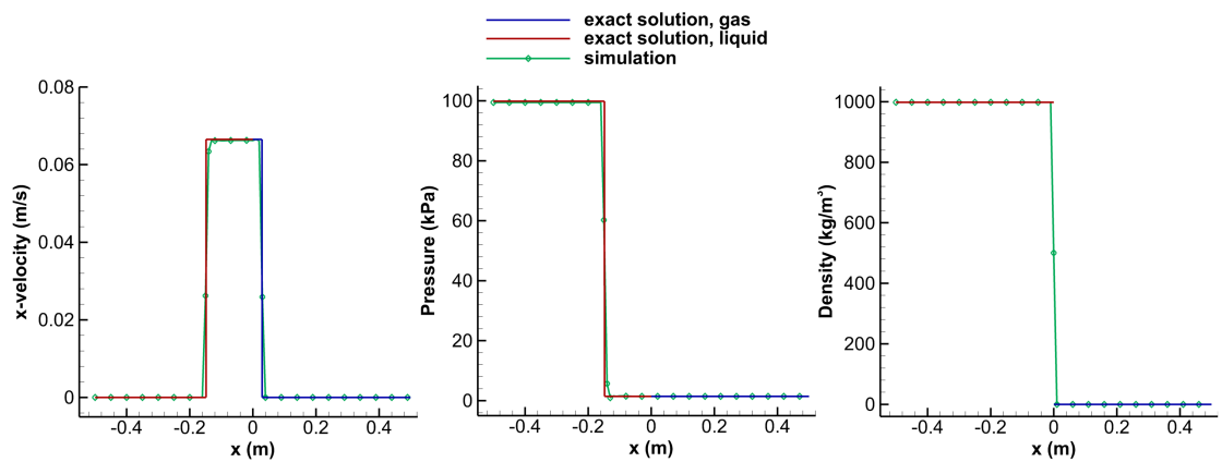
Figure 3.2: Verification of the two-phase solver for the Riemann problem. Comparison of the x-velocity (left), pressure (middle) and density (right) between the exact and the numerical solution at time t = 0.1 \mu\text{s} . Second order accuracy in space with 500 cells has been used.
