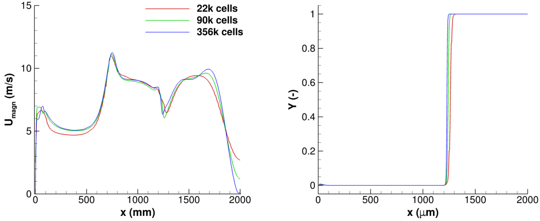
Figure 4.5: Grid independence study for the needle-free device. Plots of velocity magnitude (left) and gas mass fraction(right) along a line parallel to the x-axis ( y = 175 \mu m ) at t = 10 \mu s .
