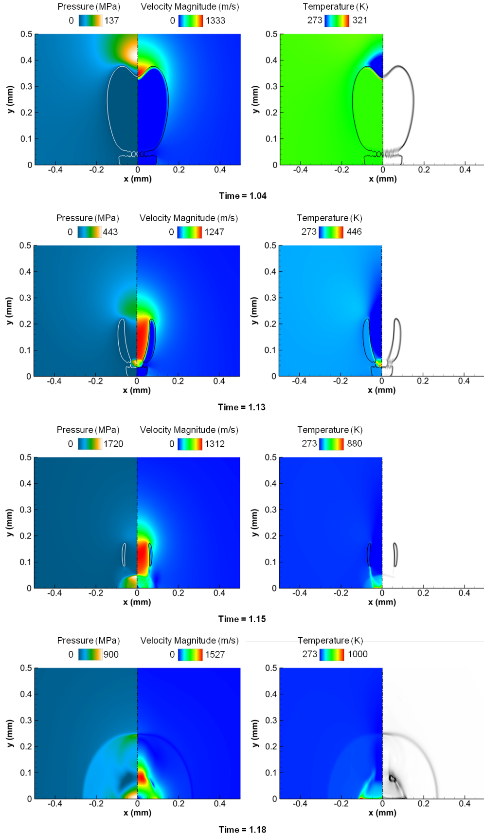
Figure 3.10: Contour field instances during vapour bubble collapse for d = 416 \mu m . Time has been non-dimensionalized with \tau = 2.88 \mu s .
