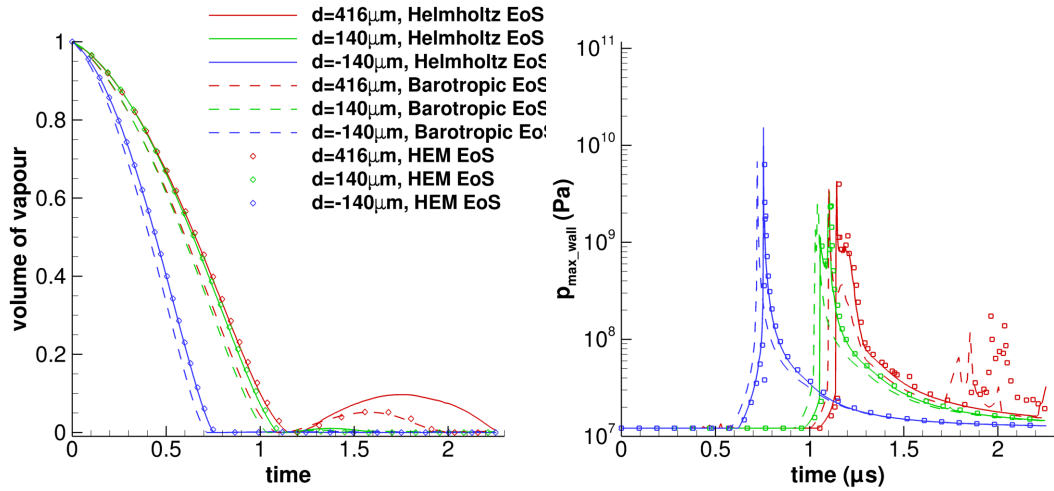
Figure 3.19: Vapour volume fraction of the bubble and maximum wall pressure with respect to time. Time has been non-dimensionalized with \tau = 2.88 \mu s .
