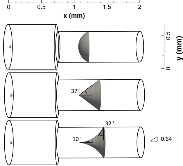
Figure 4.10: Initial condition of the meniscus, from top to bottom: hemispherical initialisation ( case 3 ), conic initialisation ( case 8 ) and trumpet initialisation ( case 9 ). The opening angle of the cone is 37^\circ , the opening angle of the trumpet is 10^\circ , the contact angle between the interface and the y axis is 32^\circ and the aspect ratio is 0.64.
