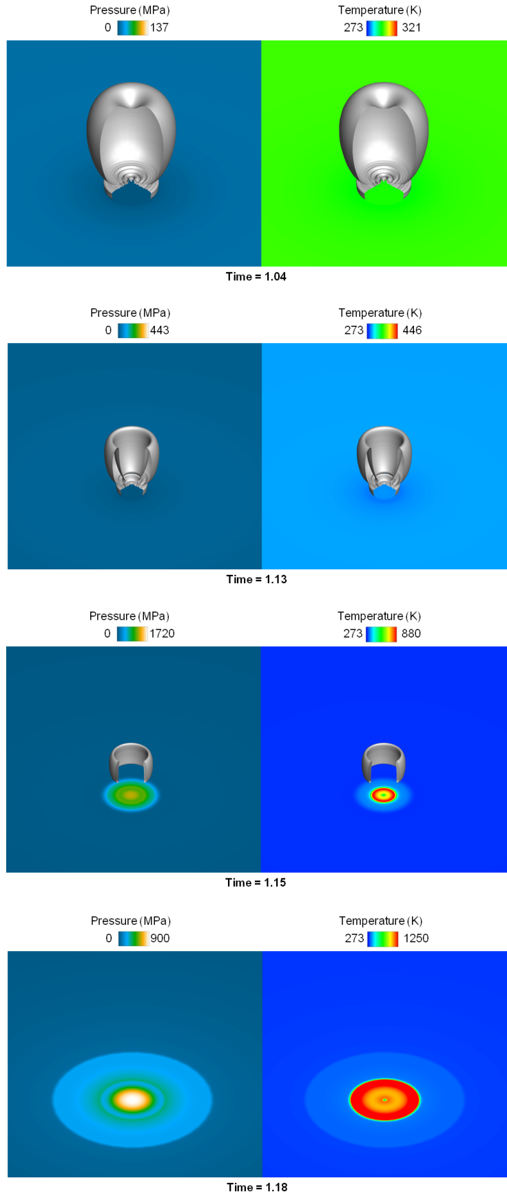
Figure 3.13: Wall pressure and temperature contours combined with bubble iso-surface of \rho = 380 \text{ kg/m}^3 for d = 416 \text{ }\mu\text{m} . Time has been non-dimensionalized with \tau = 2.88 \text{ }\mu\text{s} .
