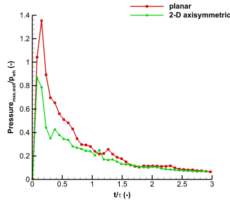
Figure 3.37: Comparison of the maximum wall pressure between a planar 2-D and a 2-D axisymmetric simulation at impact velocity 110 \text{ m/s} . Wall pressure is non-dimensionalized with p_{wh} and time is measured from the moment of the impact and it has been non-dimensionalized with \tau = D/c_l .
