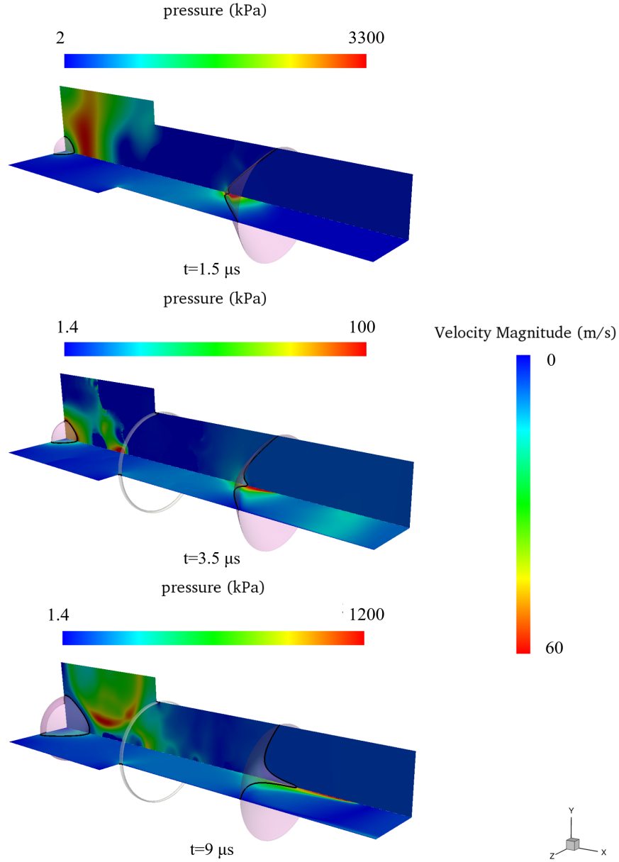
Figure 4.12: 2-D axisymmetric needle-free device simulation for p_{bub} = 5 \cdot 10^7 \text{ Pa} and the conical meniscus shape ( case 8 ). Pressure field on the x-y plane and velocity magnitude field on the x-z plane are shown, combined with iso-surface for vapour volume fraction \alpha = 0.5 (white) and iso-surface for gas volume fraction B_g = 0.5 (pink).
