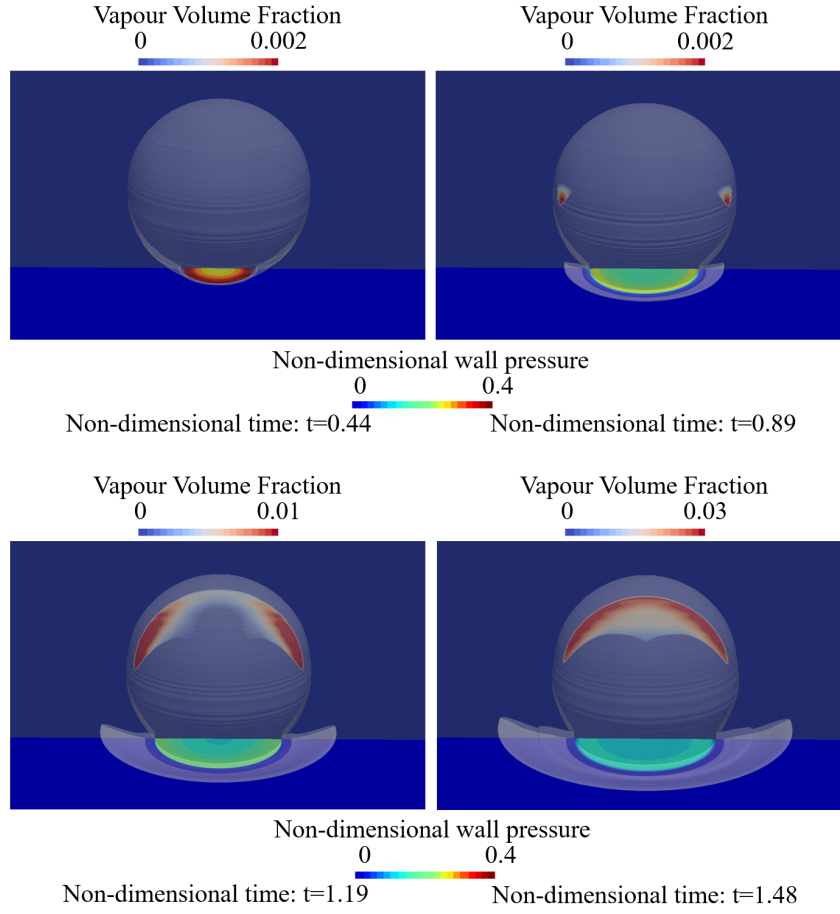
Figure 3.36: Drop impact at velocity 110 \text{ m/s} . Iso-surface of liquid mass fraction for Y_g = 0.5 combined with wall pressure (bottom slice) and vapour volume fraction (upper slice). Pressure is divided by p_{wh} and time is measured from the moment of the impact and it has been non-dimensionalized with D/c_l .
