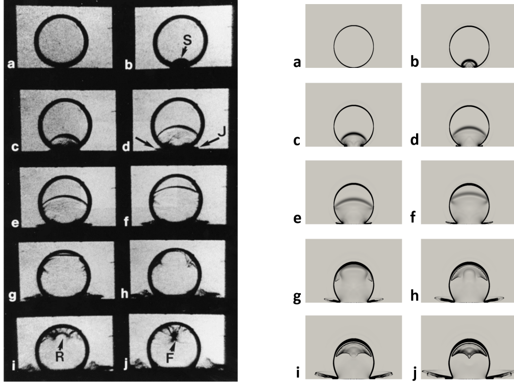
Figure 3.32: Validation of the numerical solution (right) against experiment (left) for a 2-D drop impact on a solid wall with impact velocity 110\text{ m/s} . The interframe time is t = 1\text{ }\mu\text{s} . The left figure is taken from Field et. al [163].
