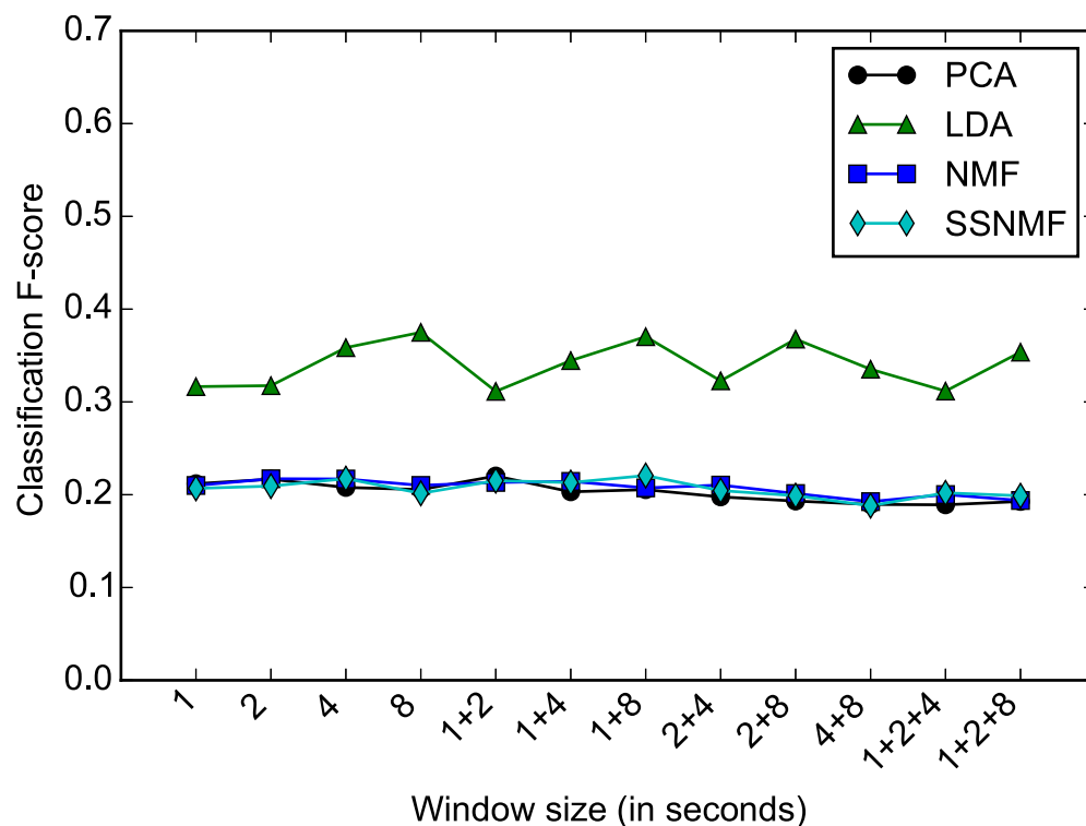
Fig 6. Classification F-score on the validation set for the best performing classifier (LDA) across different window sizes. Accuracies are compared for different feature learning methods (PCA, LDA, NMF, SSNMF). Combinations of window sizes are marked by '+' in (a), for example '4+8' represents the accuracy when combining features from the 4-second and the 8-second windows. Considering the performance of all feature learning methods, the optimal window size is 8 seconds.
