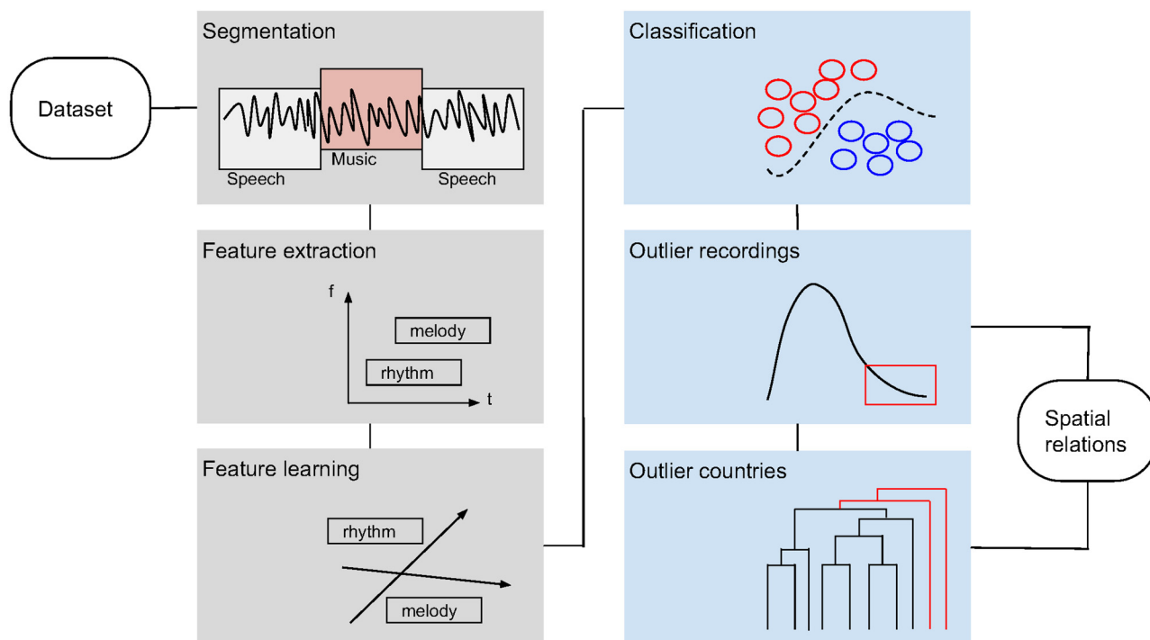
Fig 1. Overview of the methodology.
