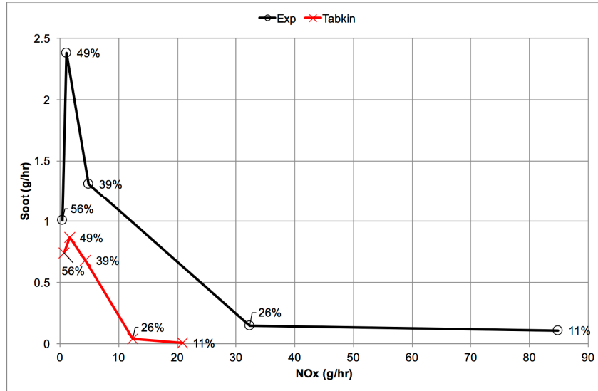
Fig. 5 NO x / soot trade-off measured vs. simulated; percentages indicate EGR level.
