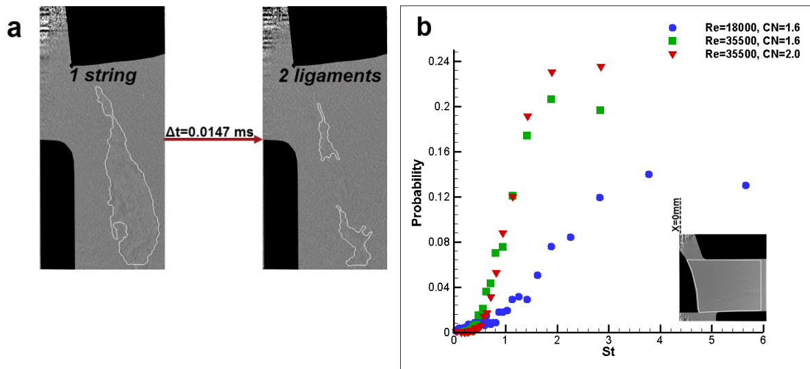
Figure 5. (a) Detection of string break-up and (b) effect of the flow conditions on the string break-up behaviour.
