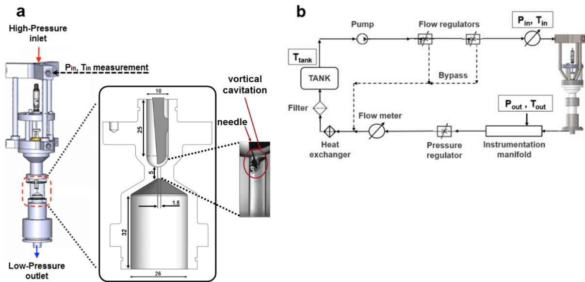
Figure 1. Schematic layout of (a) the test-bench and (b) the hydraulic flow loop.
