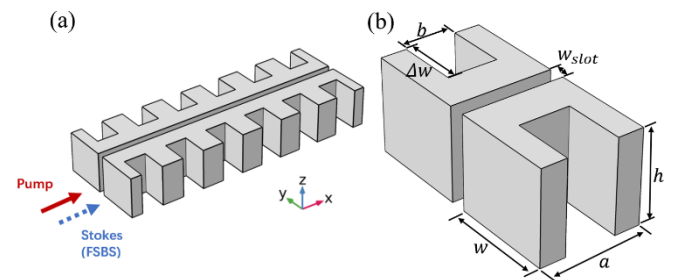
Fig. 1. (a) Proposed structure of the slot waveguide Bragg grating suspended in air. (b) Unit cell of the proposed structure
