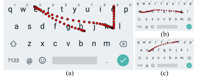
Figure 1: The coordinates captured as a user uses gesture typing to enter the words (a) "hello", (b) "ask" and (c) "is" onto the device. We note the diverse nature of gestures for different words.
