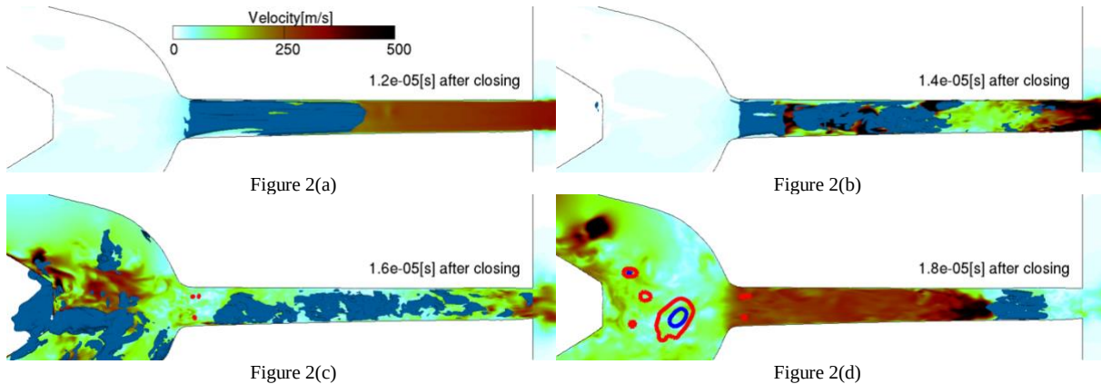
Figure 2 – Flow fields at different instants after the needle touches the wall. Y-cut of the velocity field, iso-surface at 0.9 of the vapor volume fraction in blue and iso-lines at 3,500 [bar] (red) and 5,000 [bar] (blue) of the recorded pressure peaks on the walls.
