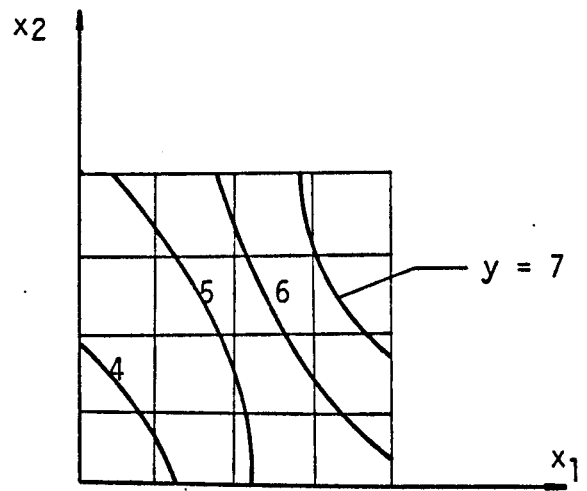
Fig. 2.2. Contour representation of a response surface
