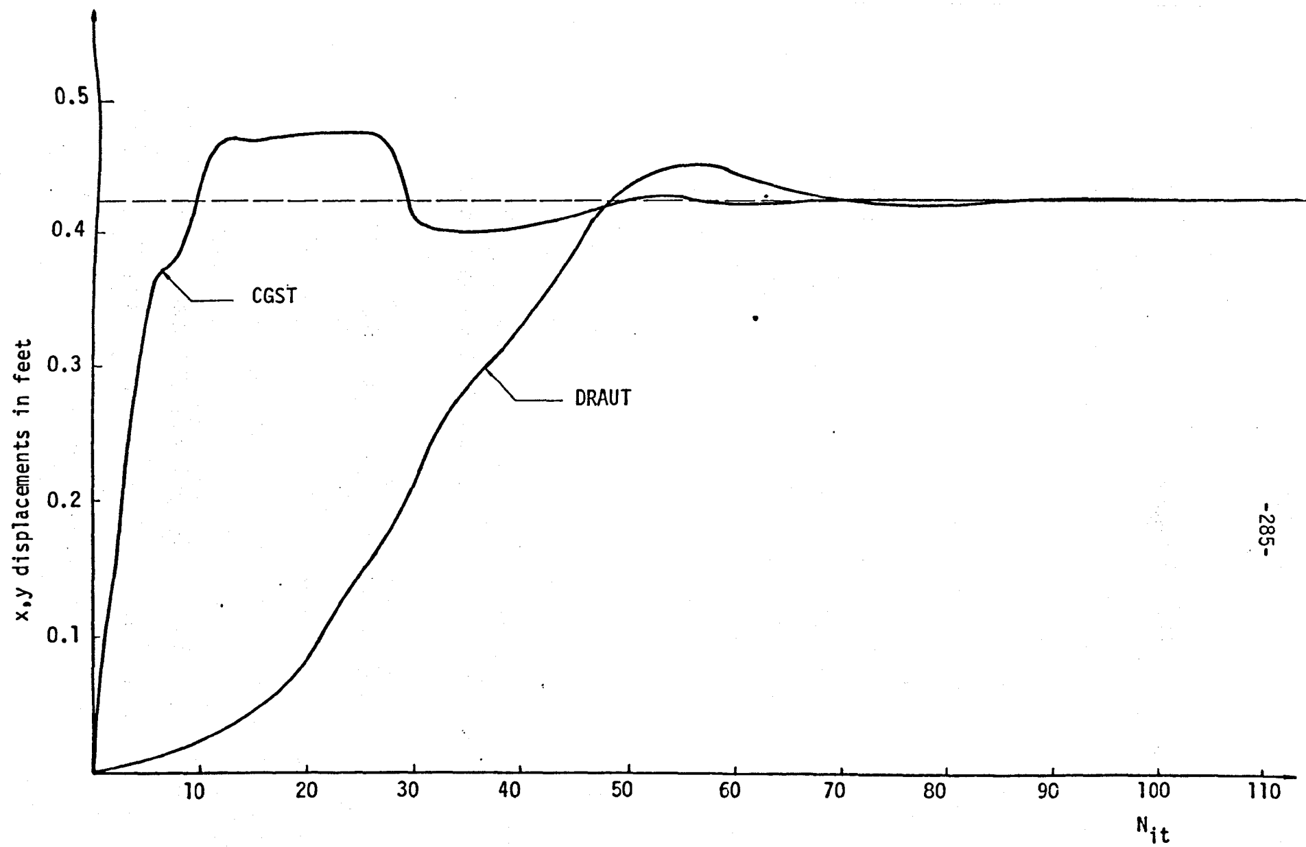
Fig.9.3 Convergence of horizontal deflections of point 5 versus the iteration index N_{it} , for example 4
