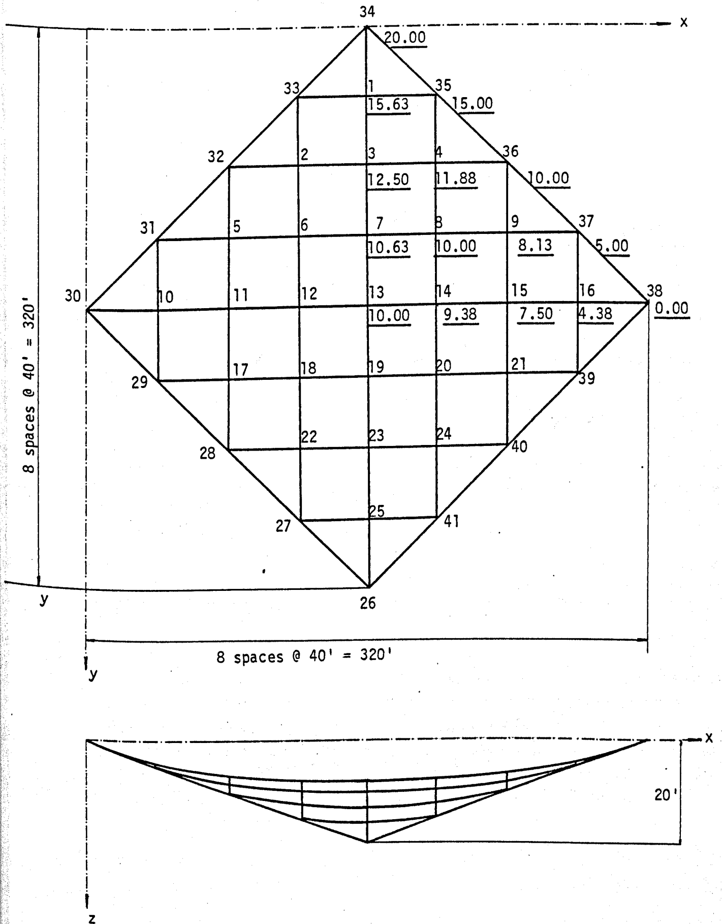
Fig. 2.9 Hyperbolic-paraboloid prestresset net, example 3.
