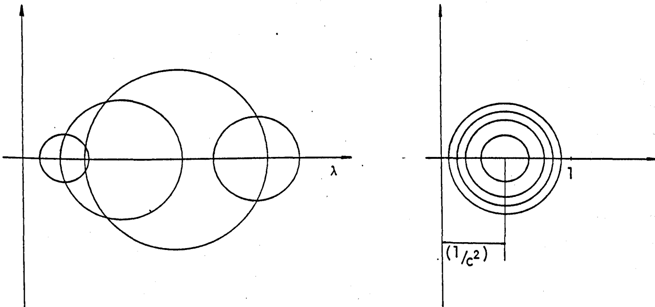
(a) Gerschgorin discs for an unscaled matrix
