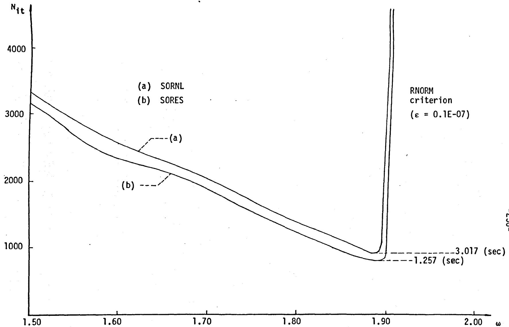
Fig. 7.3. Convergence of SORN and SORES with different relaxation parameters \omega (example 2. Load case "B")
