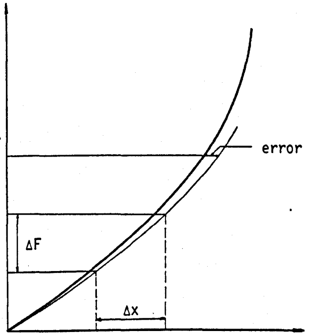
Fig. 8.14 Perturbation method
