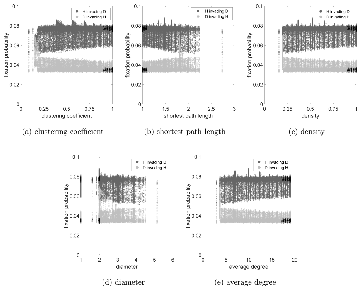
FIG. 3. Fixation probability as a function of a. Clustering coefficient, b. shortest path length, c. density, d. diameter and e. average degree for all networks simulations for the Hawk-Dove game. The dark grey dots represent case of H invading D, the light grey dots represent the case of D invading H and for both cases, black dots represent simulations with well-mixed networks. The parameter values are R = 10 , C = 1 , V = 2 .
