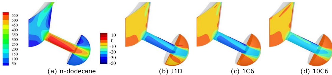
Figure 5: Velocity contour profile for n-dodecane and the relative value for the mixture surrogates with respect to n-dodecane.
