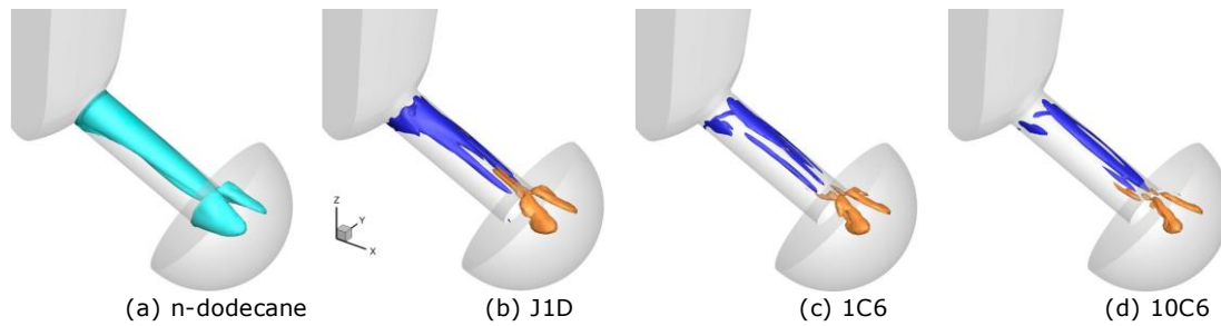
Figure 6: Vapour volume fraction isosurface at 10% for n-dodecane and the relative value for the mixture surrogates with respect to n-dodecane. The color code for the relative values is blue for higher vapour fraction and orange for a lower value than that for n-dodecane.
