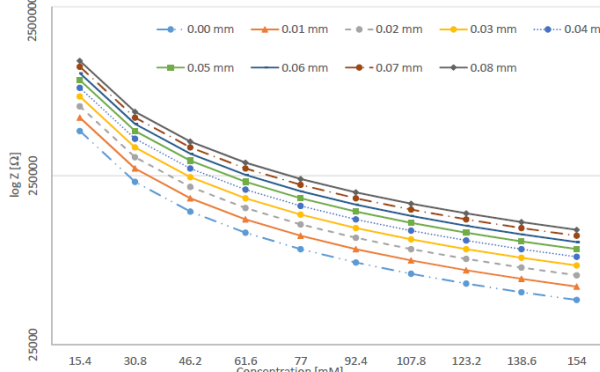
Figure 5. Impedance vs concentration for varying parameter A – distance between PU electrodes
