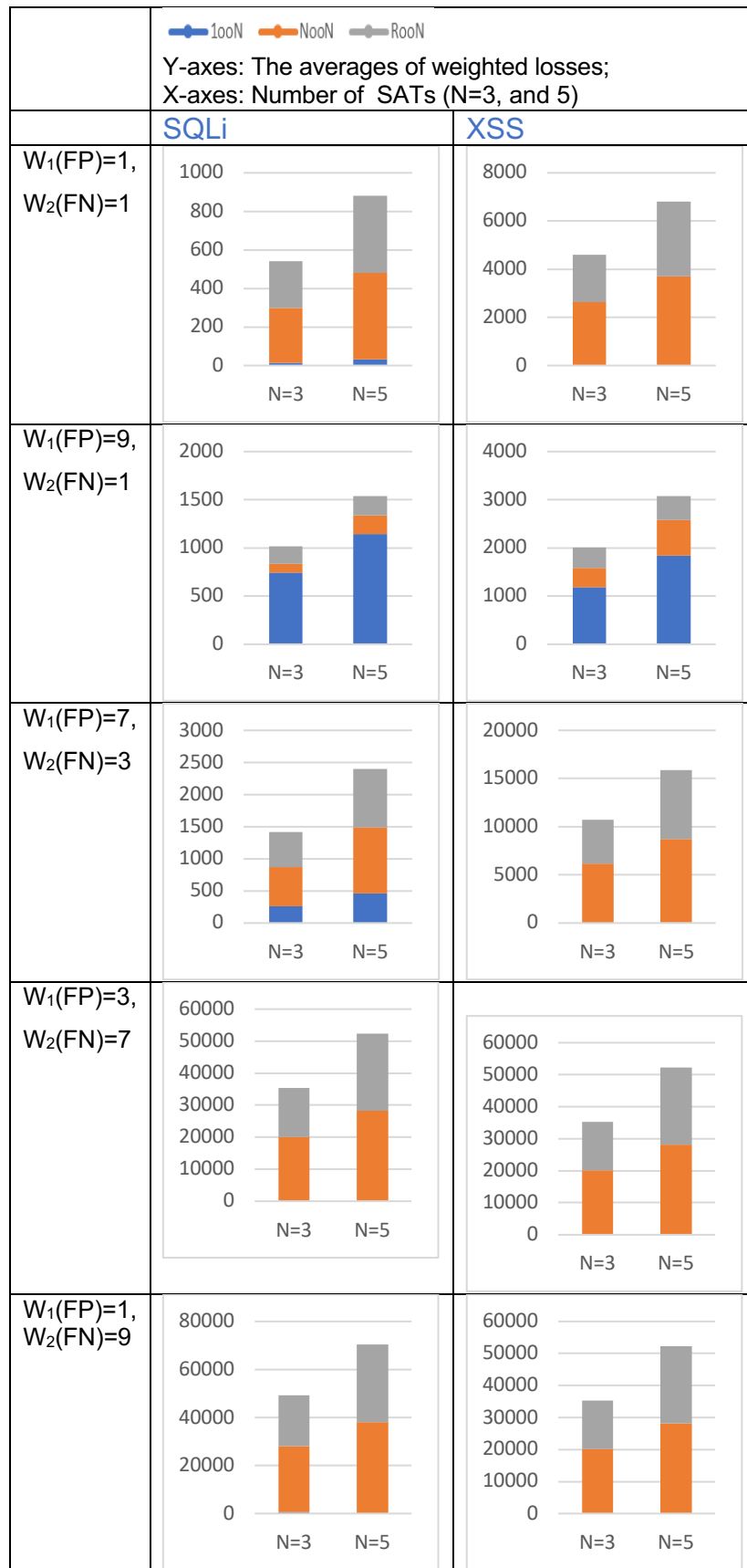
Figure 8-6 The average loss difference between the optimal adjudication function and the other diverse SAT setup (100N,majority vote and N00N) for each application.
