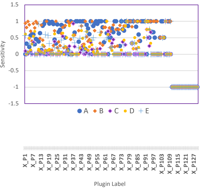
Figure 7-5 Vulnerable and non-vulnerable lines count per plugin and sensitivity measures, for SQLi and XSS.
