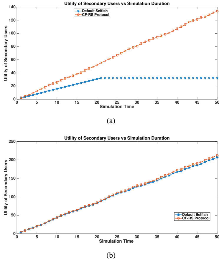
Figure 5.17 Utility of secondary user for configurations b and c : (a) Only one nearby relay; and (b) All relays located on coverage boundary.
