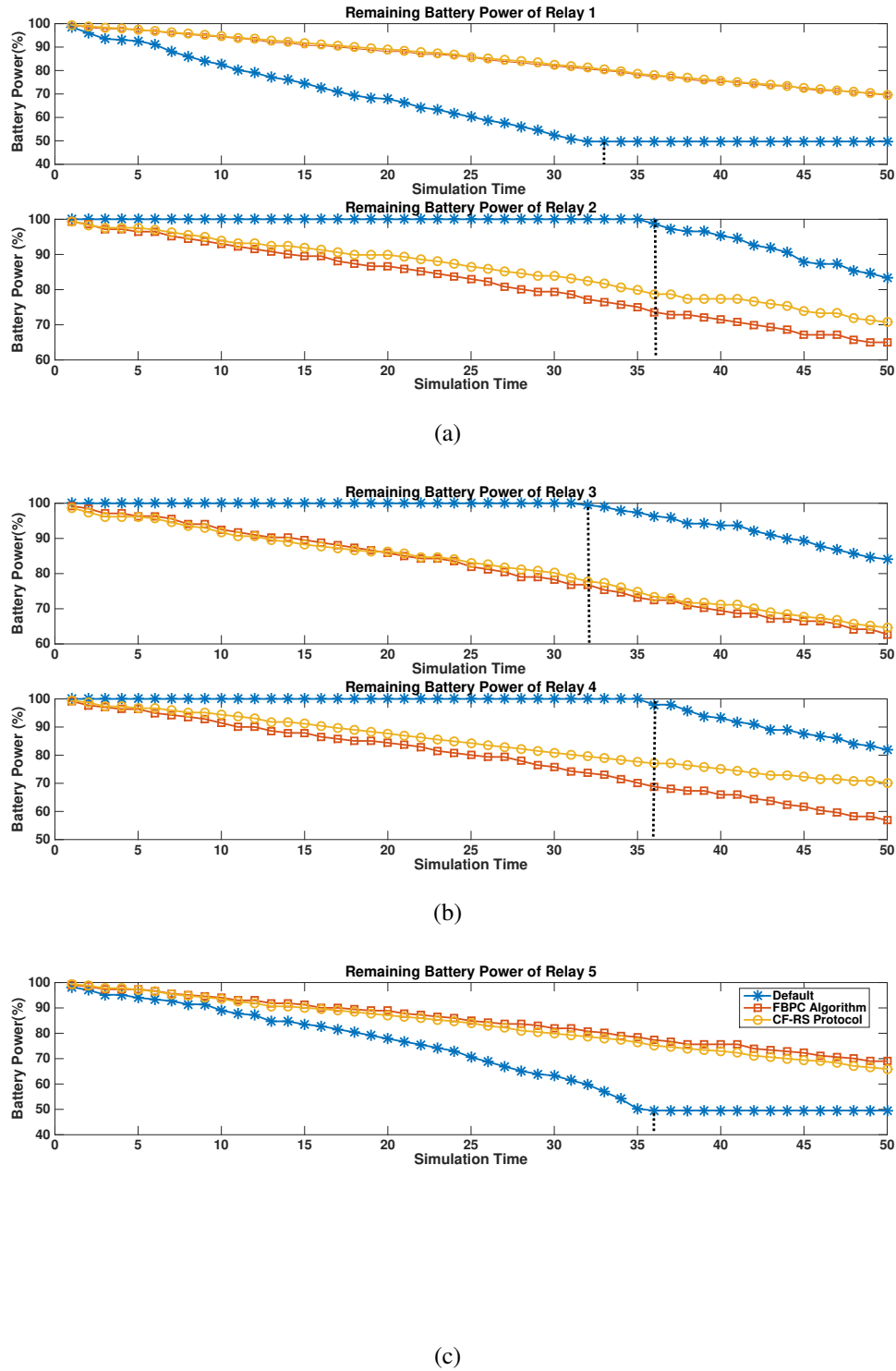
Figure 5.4 Comparison of utilization of battery power of individual relays for the default and FBPC algorithms and CF-RS protocol : (a) Battery power of relays 1 and 2 ; (b) Battery power of relays 3 and 4 and (c) Battery power of relays 5.
