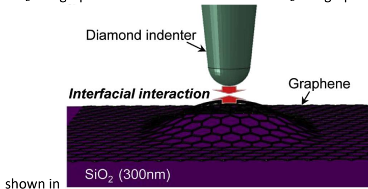
Fig.3. The classic Hertz, Johnson-Kendal-Roberts (JKR) and Derjaguin-Muller-Toporov (DMT) contact mechanics models were utilized to convert the mapped force profile into the adhesion energies. Other researchers have used AFM cantilever tips of different materials and shapes as the nano-indenter so as it approaches or moves away from the graphene, the measured resultant forces can be converted to the appropriate adhesion energies. The graphene was either in the form of a few layers as a free-standing beam [39] or on a metallic substrate [40][41][42].
