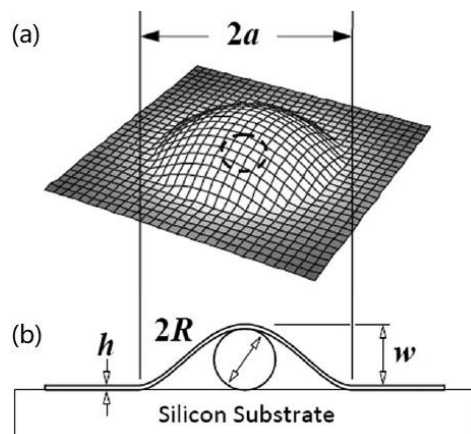
Fig.13 A typical circular blister traps a nanoparticle at the interface: (a) a 3D characterization; (b) schematic of blister for modelling and analysing [111].
