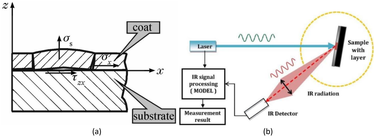
Fig.6(a) Force diagram of coating peel-off after scratched by laser [71]; (b) Schematic of Nd-YAG pulse laser active and lock-in thermography for non-destructive testing [72].
