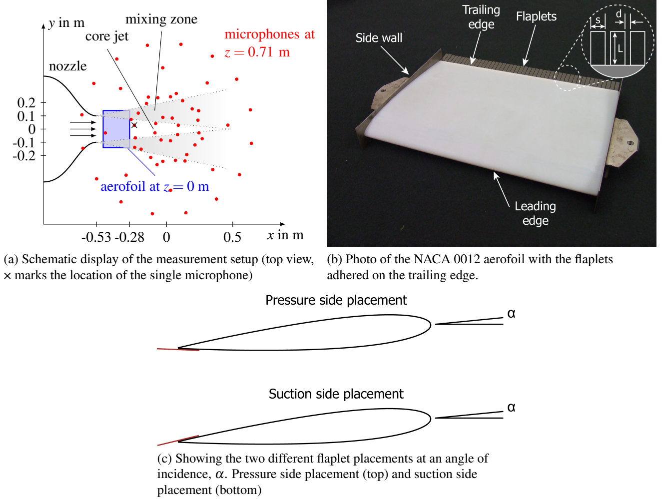
Figure 1: Experimental set-up
