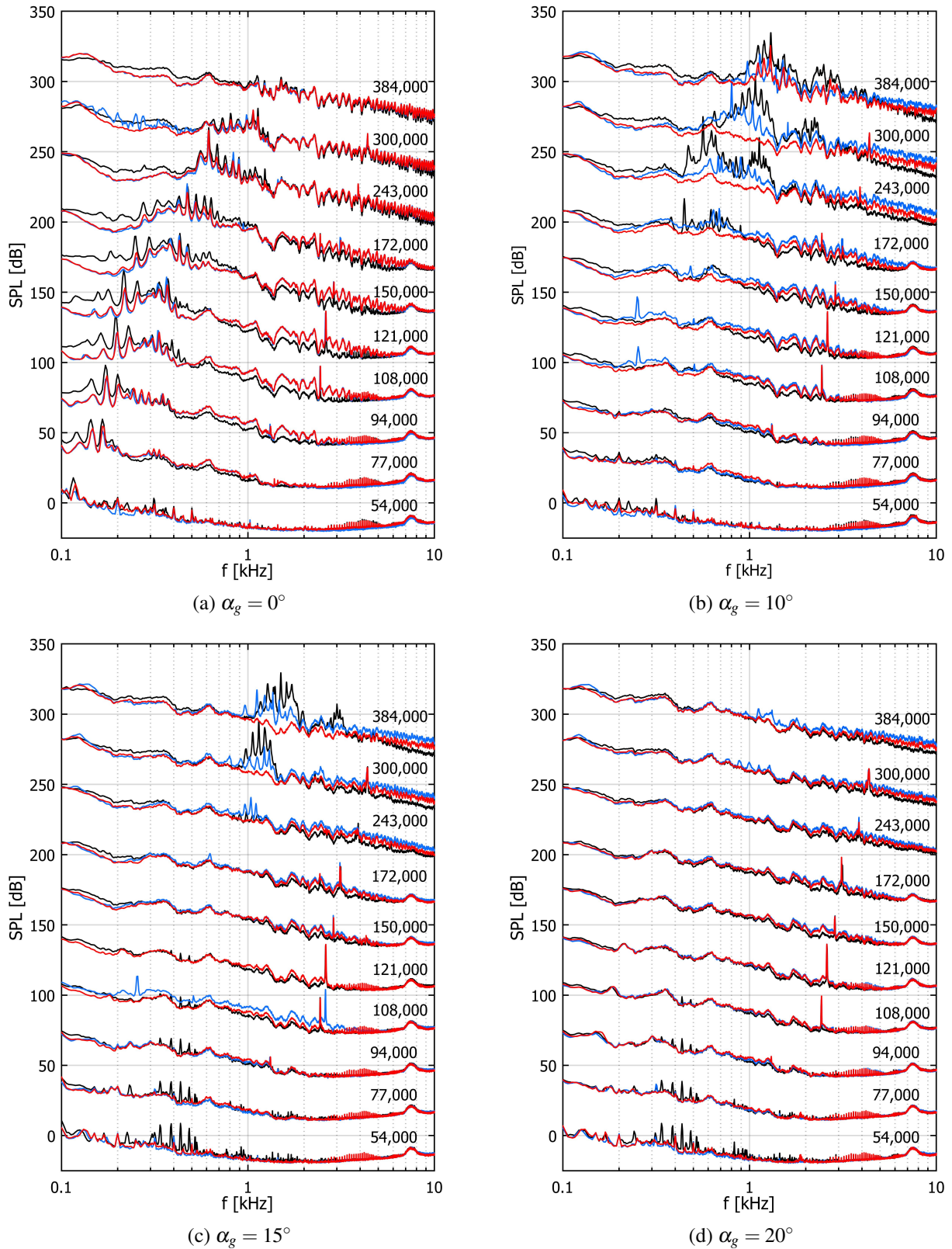
Figure 4: Single microphone measurements for each Reynolds number case, are spaced with 30dB increments for clarity. Each of the angles stated are the geometric angles of attack. For each angle and Reynolds number there are three test cases: a baseline case with no flaplets (—), the case where the flaplets are affixed to the pressure side (—) and when the flaplets are affixed onto the suction side (—).
