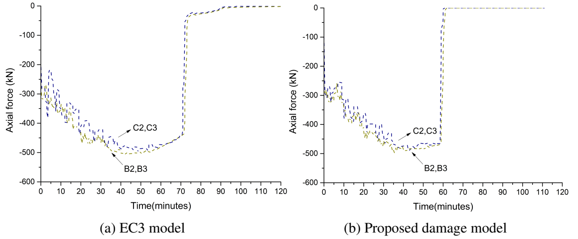
Fig. 5.86 Axial forces in columns during fire event
