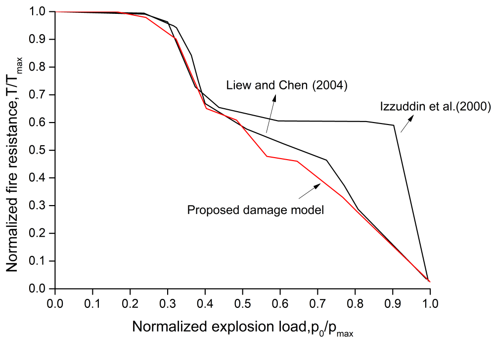
Fig. 4.34 Influence of explosion loads on the fire resistance of steel frame
