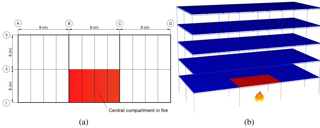
Fig. 5.16 Location of the central compartment fire on the ground floor
