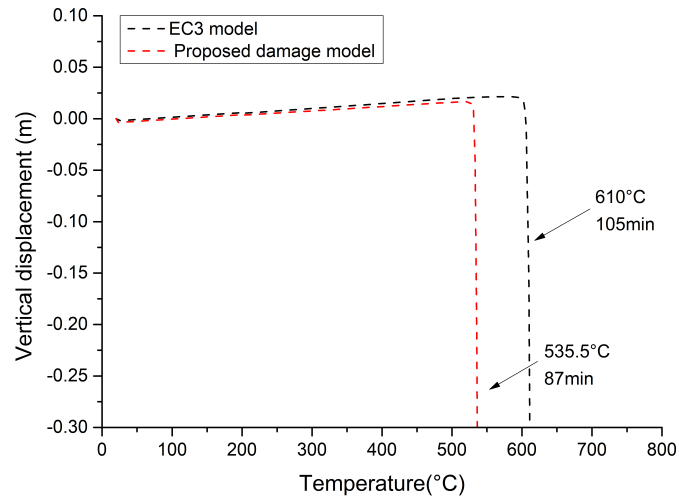
Fig. 5.92 Vertical displacement of the heated interior column B2
