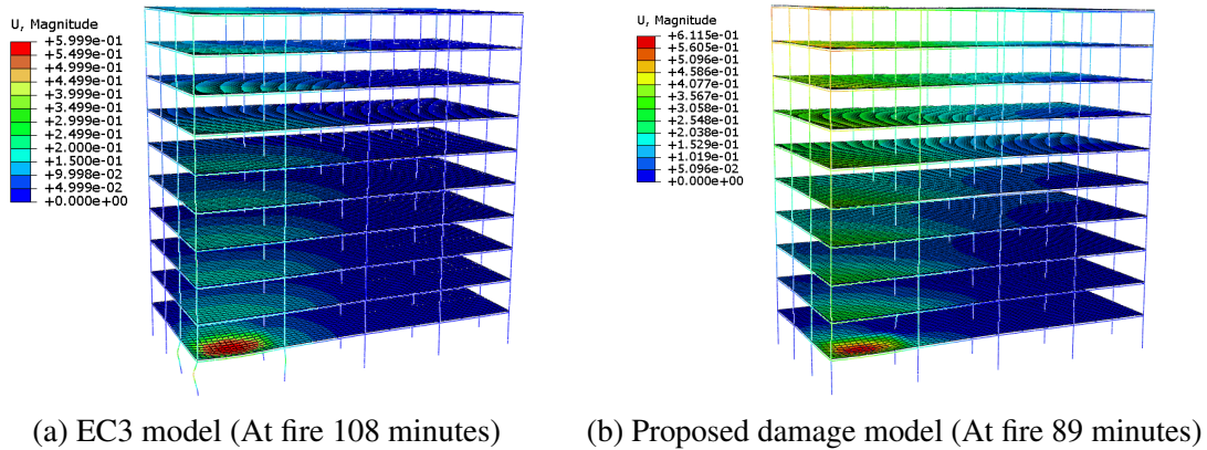
Fig. 5.35 The deformed shape of the building before column buckling initiates
