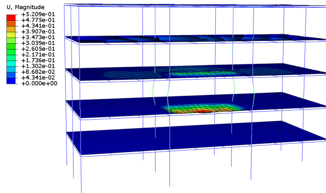
Fig. 5.64 Blast induced deformation after the blast analysis in the central compartment on the third floor
