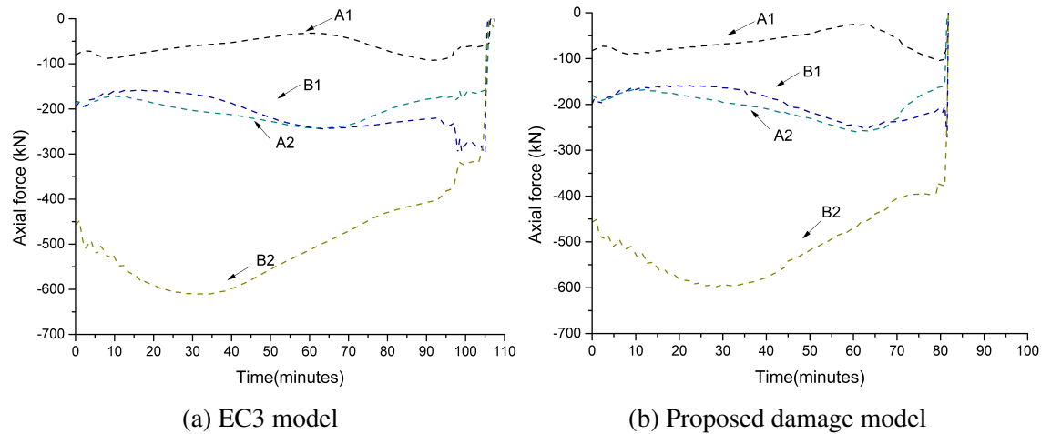
Fig. 5.29 Axial forces in columns during fire event
