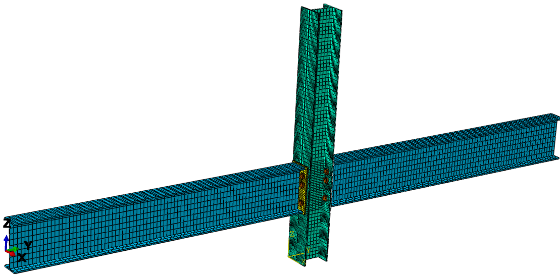
Fig. 4.9 Numerical model of flush end plate connection in ABAQUS
