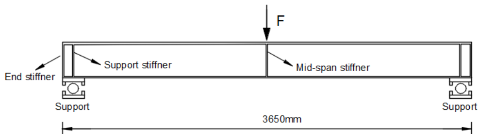
Fig. 4.1 Test set-up (Dharma and Tan, 2007)
