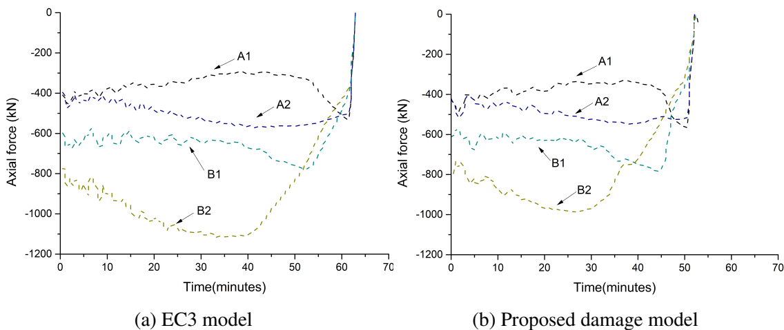
Fig. 5.62 Axial forces in columns during fire event
