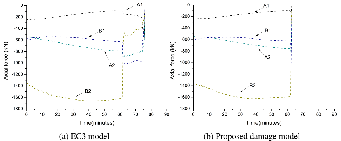
Fig. 5.22 Axial forces in columns during fire event
