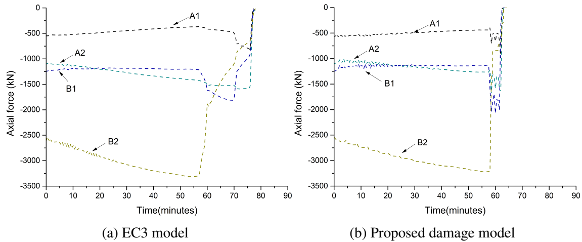
Fig. 5.43 Axial forces in columns during fire event
