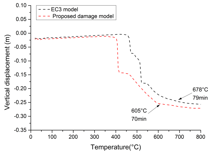
Fig. 5.79 Vertical displacement of the heated interior column B2
