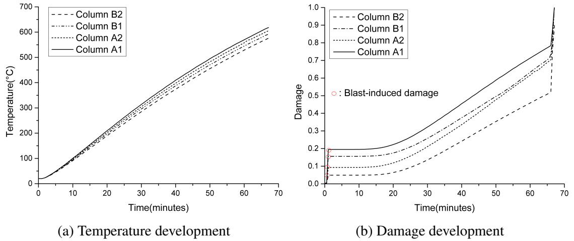
Fig. 5.56 Damage development in the top of columns subjected to blast and fire
