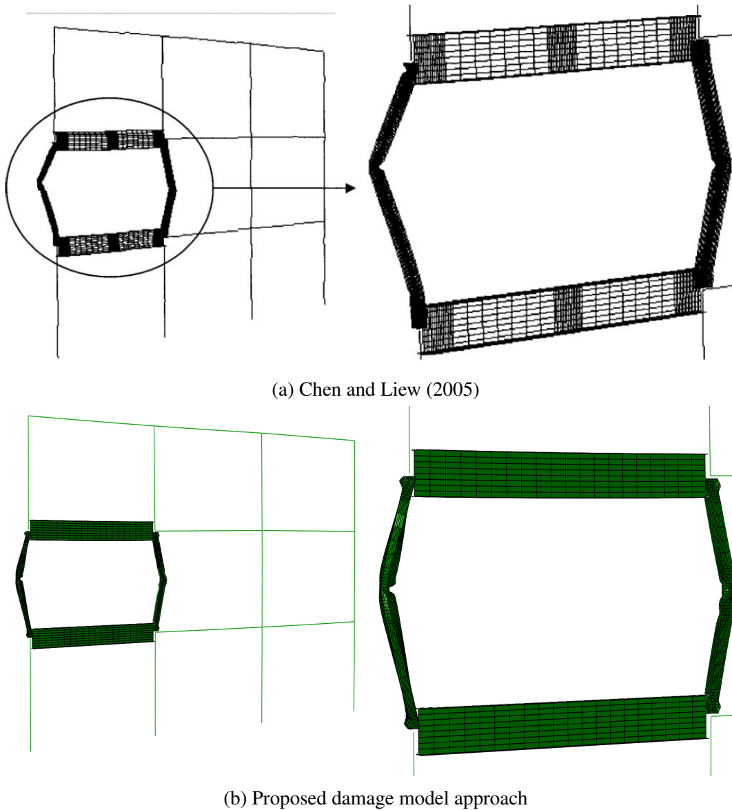
Fig. 4.40 Collapse modes of steel frame under blast load 90 \text{ kN/m} followed by fire
