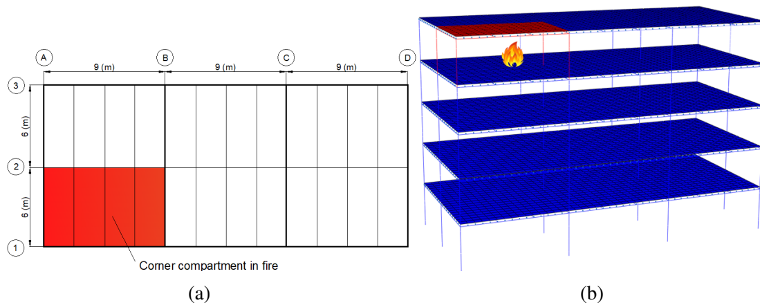
Fig. 5.27 Location of the corner compartment fire on the top floor
