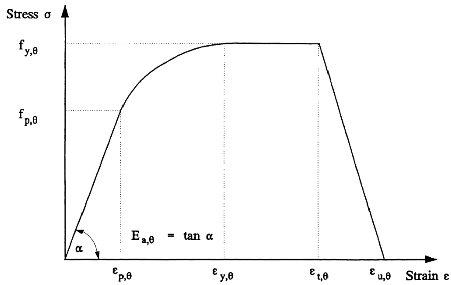
Fig. 2.7 Graphical presentation of the stress-strain relationships of structural steel at elevated temperatures (EN 1993-1-2, 2005)
