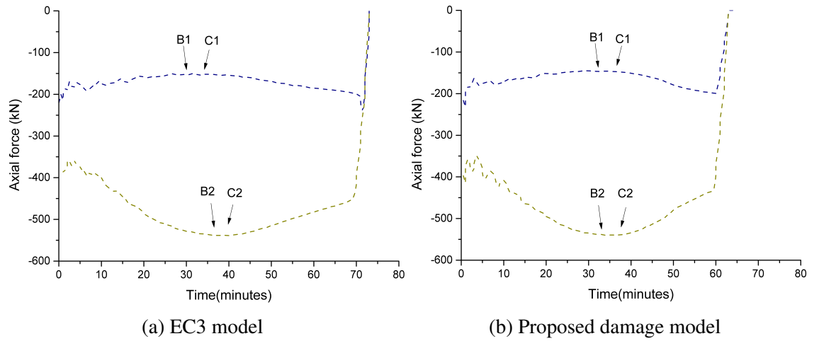
Fig. 5.72 Axial forces in columns during fire event
