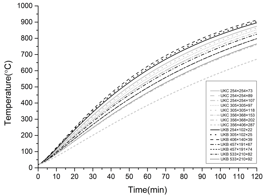
Fig. 5.4 Temperature histories of steel structural members
