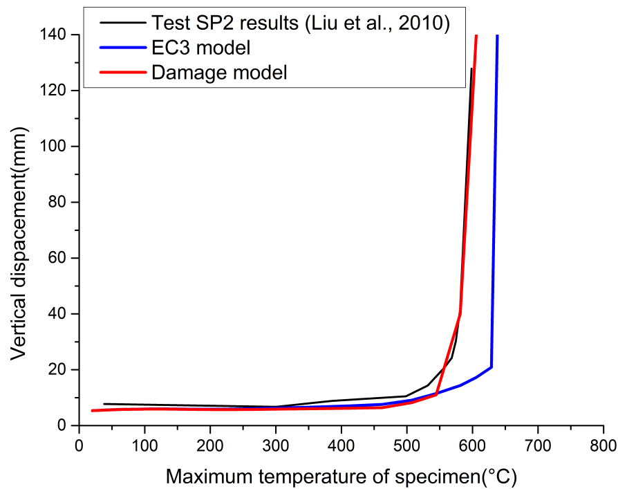
Fig. 4.25 Vertical displacement versus maximum temperature curve of specimen SP2
