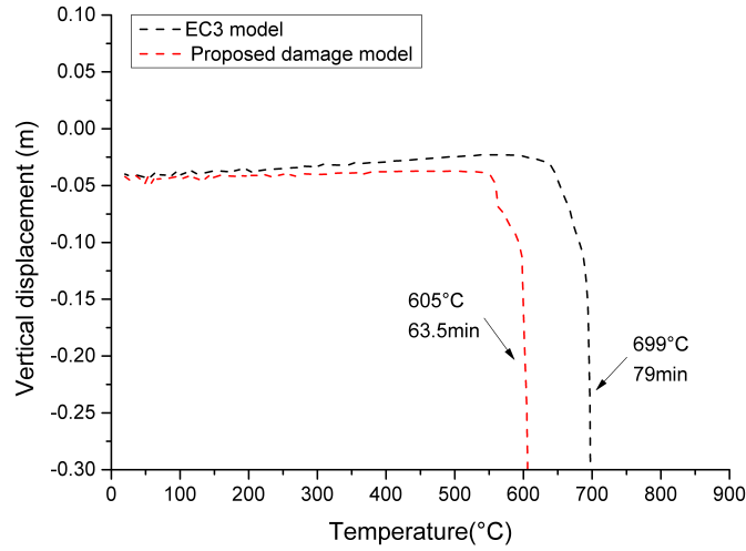
Fig. 5.82 Vertical displacement of the heated interior column B2
