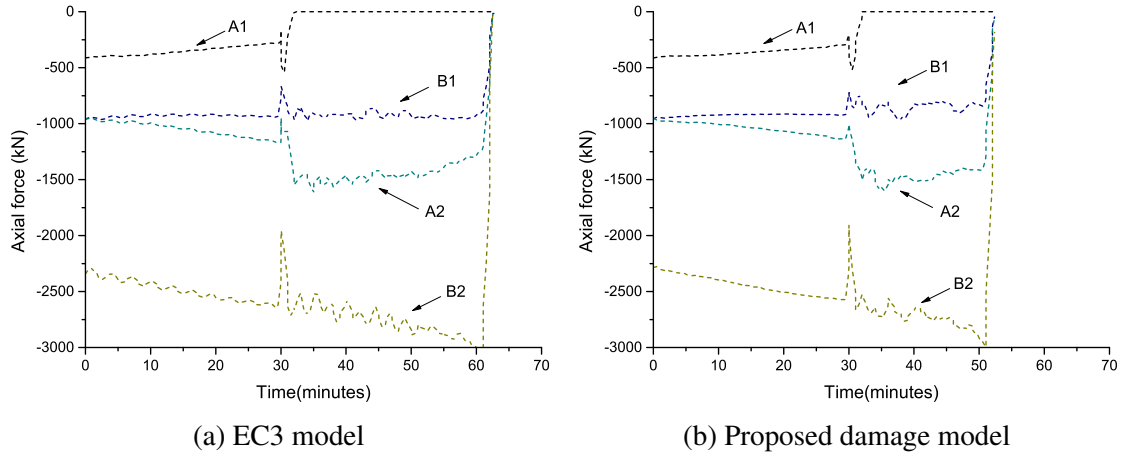
Fig. 5.89 Axial forces in columns during fire event
