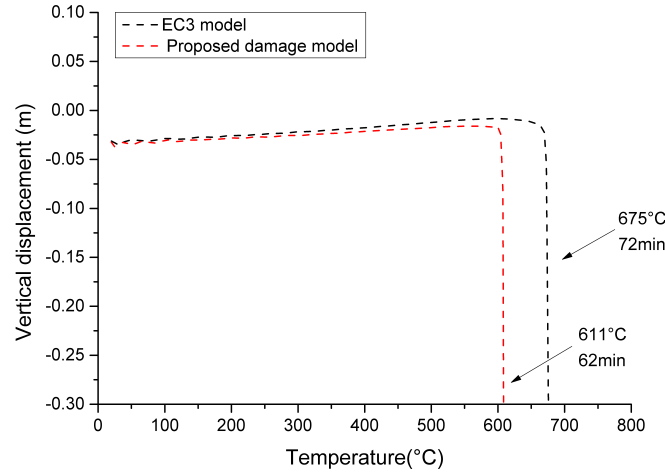
Fig. 5.71 Vertical displacement of the heated interior column
