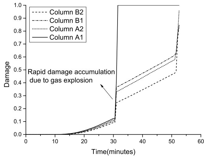
Fig. 5.90 Damage development in the top of blast-damaged columns
