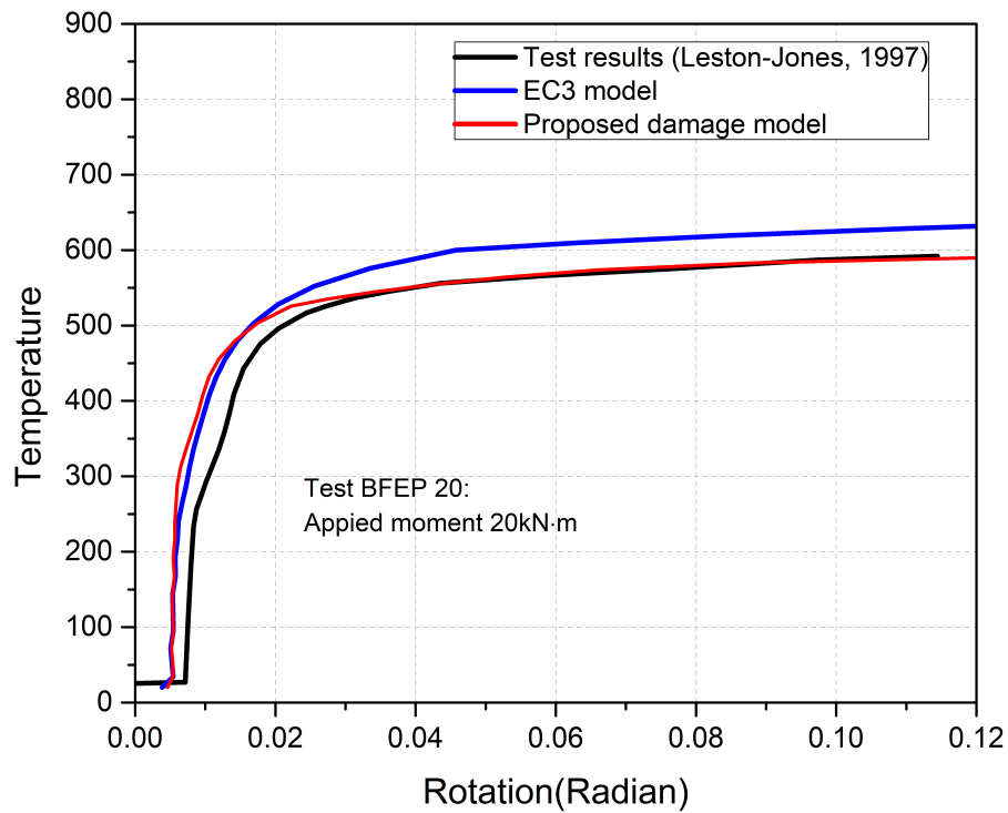
Fig. 4.19 Comparison of connection response between numerical cases and fire test 4 (BFEP20)
