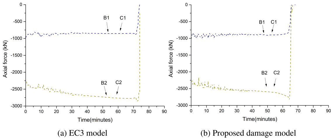
Fig. 5.59 Axial forces in columns during fire event
