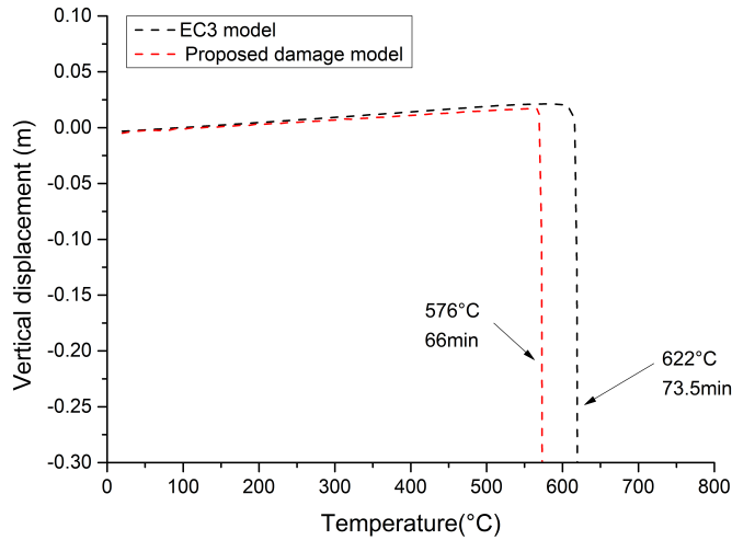
Fig. 5.54 Vertical displacement of the heated interior column B2
