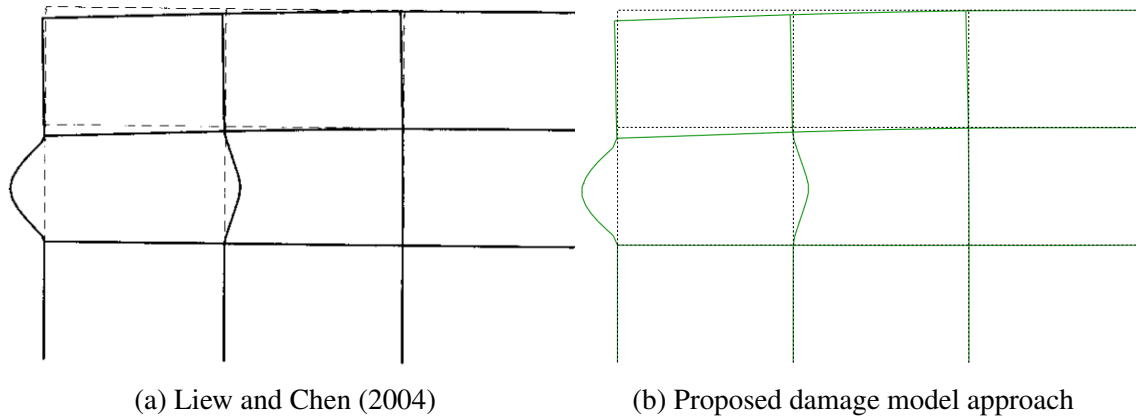
Fig. 4.32 Collapse modes of steel frame under blast loads (displacement scale factor enlarged)
