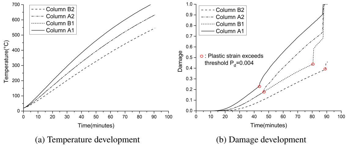
Fig. 5.37 Damage development in the top of heated columns
