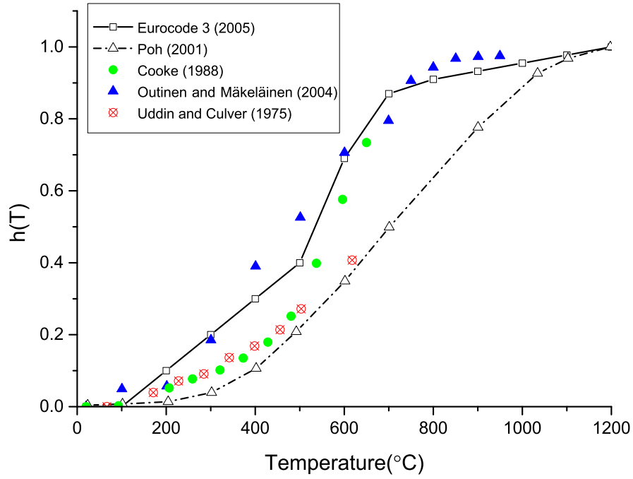
Fig. 3.1 Thermal damage variable h(T) determined from literature sources
