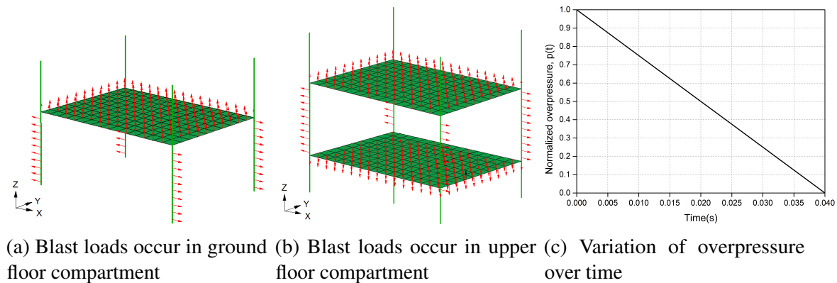
Fig. 5.9 Schematic view of the occurrence of internal blast loads
