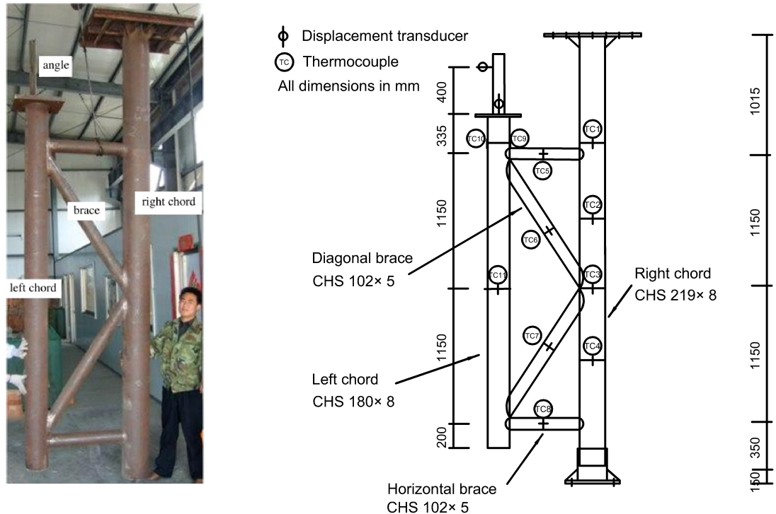
Fig. 4.21 Test set-up (Liu et al., 2010)
