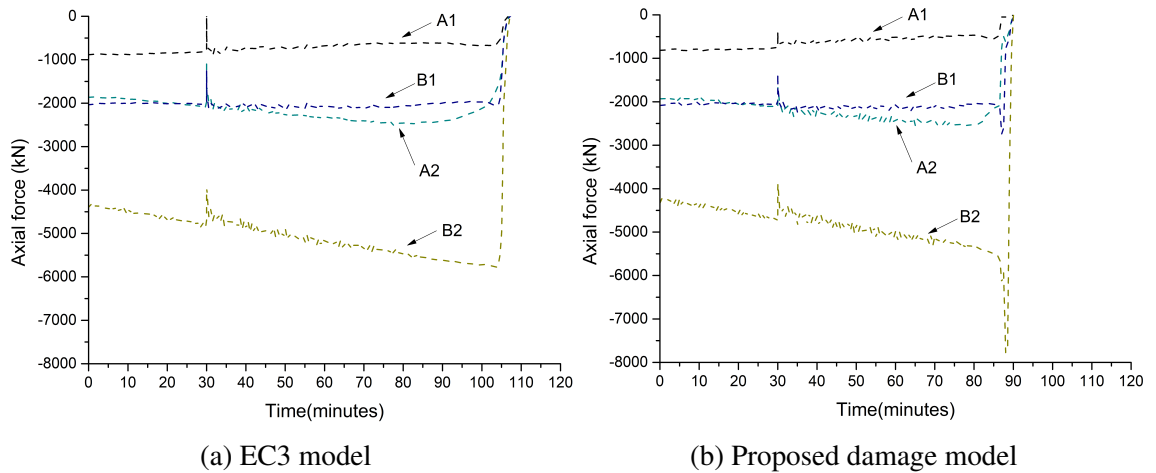
Fig. 5.93 Axial forces in columns during fire event
