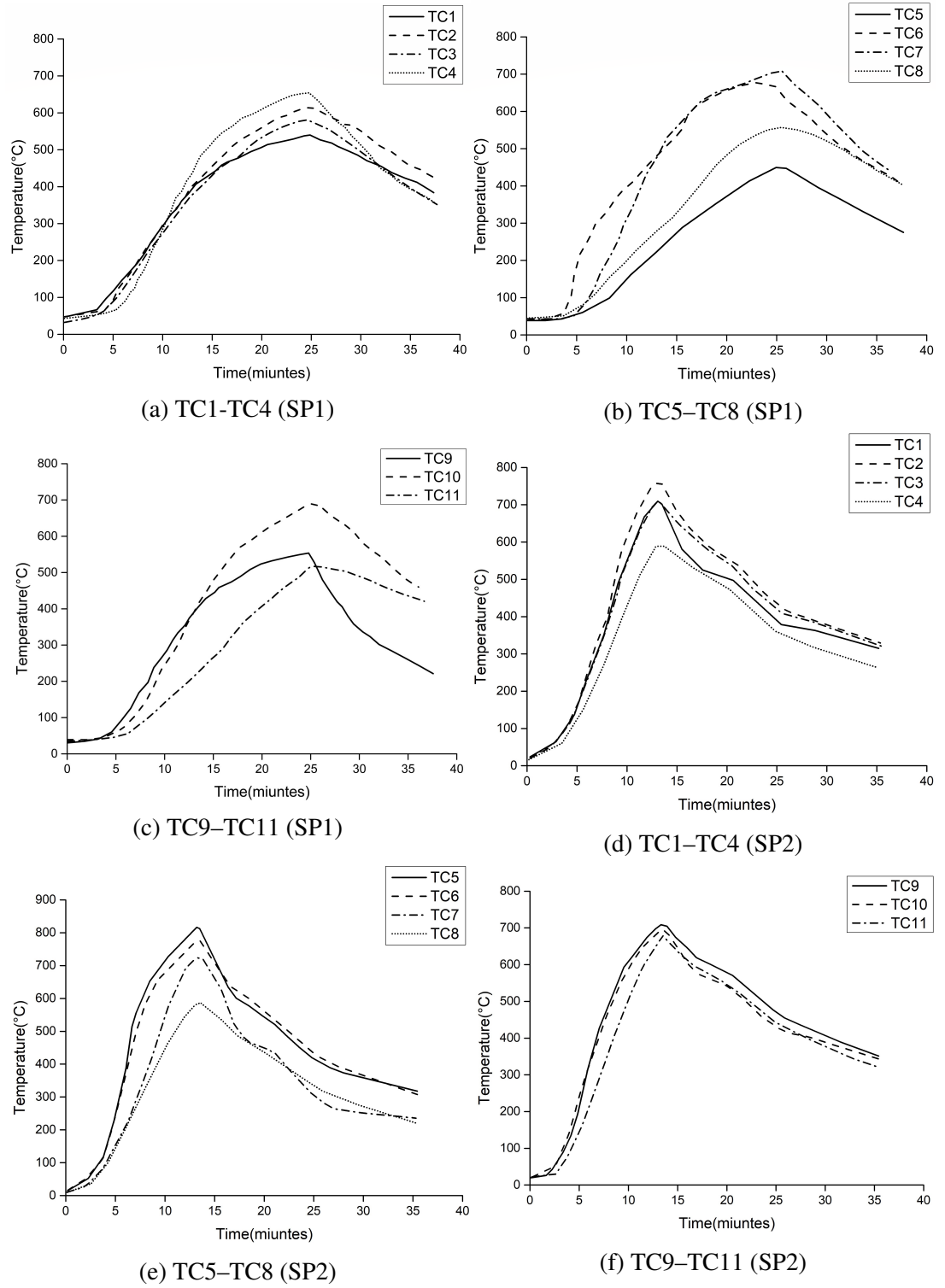
Fig. 4.23 Temperature–time curves of thermocouples TC1–TC11 for specimen SP1 and SP2 (Liu et al., 2010)
