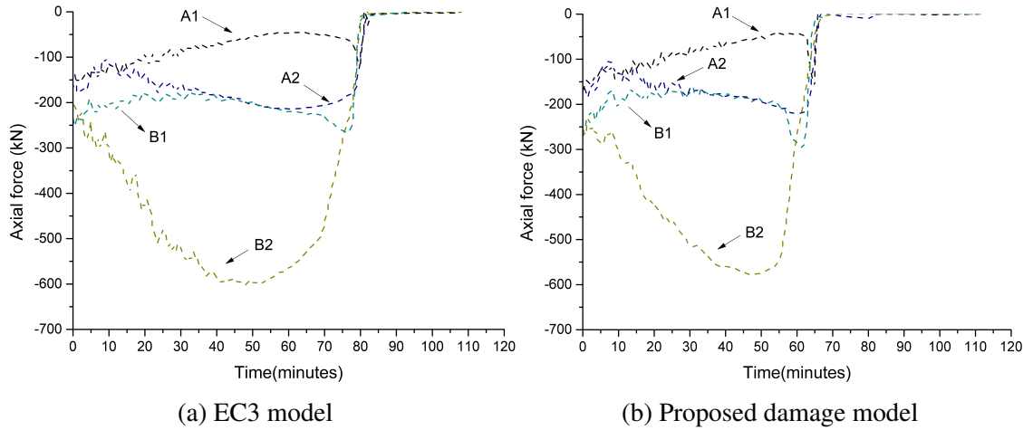
Fig. 5.83 Axial forces in columns during fire event
