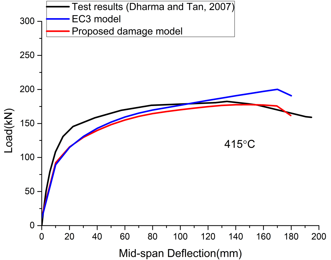
Fig. 4.5 Mid-span load–deflection of specimen S3-2
