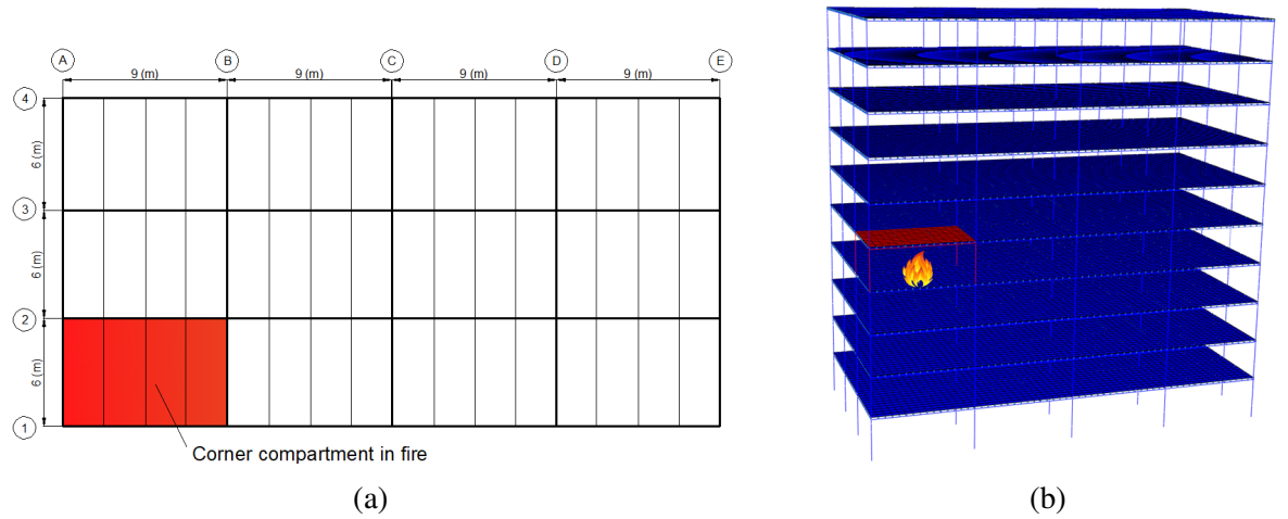
Fig. 5.41 Location of the corner compartment fire at the mid-height of the building
