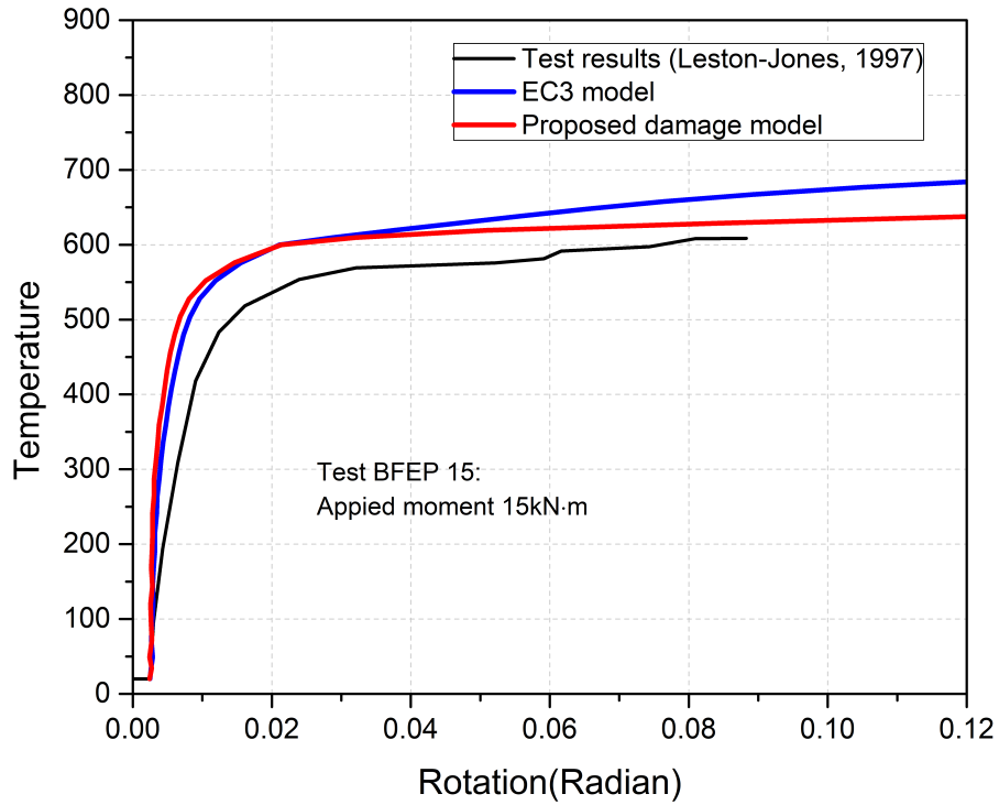
Fig. 4.18 Comparison of connection response between numerical cases and fire test 3 (BFEP15)
