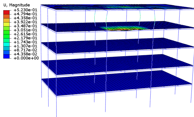
Fig. 5.70 Blast induced deformation after the blast analysis in the central compartment on the top floor
