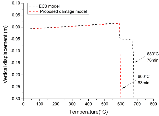
Fig. 5.21 Vertical displacement of the heated interior column B2
