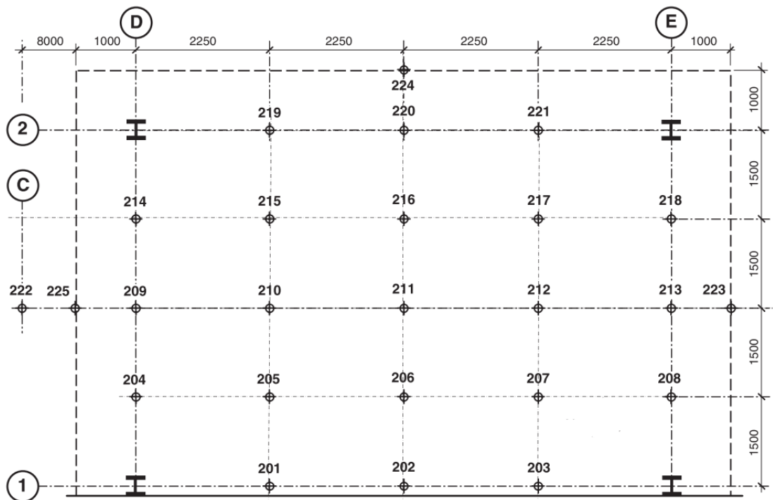
Fig. 4.50 Location of vertical displacements measurements on the fourth floor slab (Lennon, 2003)
