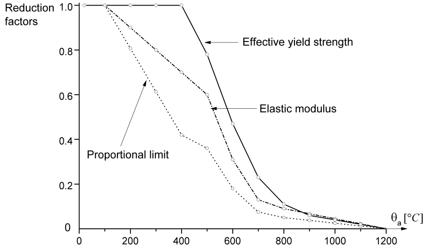
Fig. 2.8 Reduction factors for stress-strain relationships of structural steel at elevated temperatures (EN 1993-1-2, 2005)
