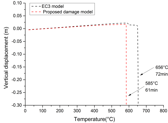
Fig. 5.25 Vertical displacement of the heated interior column B2
