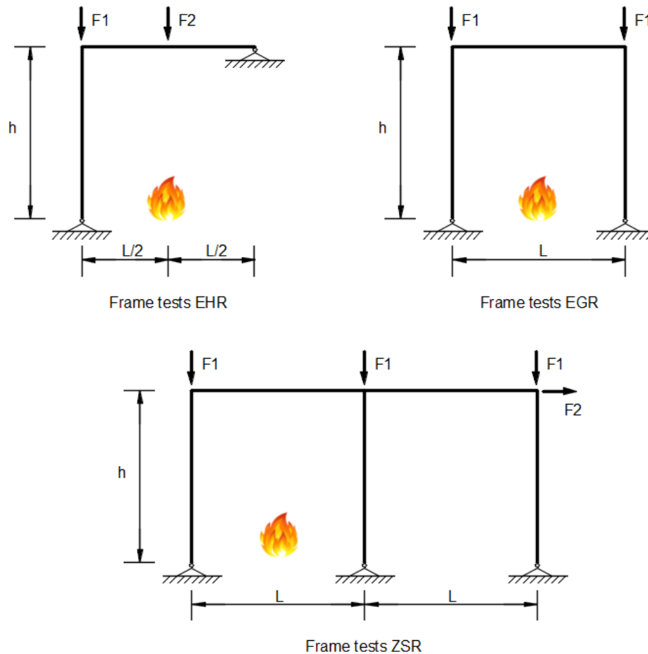
Fig. 4.26 Configurations of scaled steel frame tests (Rubert and Schaumann, 1986)
