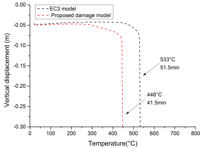
Fig. 5.65 Vertical displacement of the heated interior column B2
