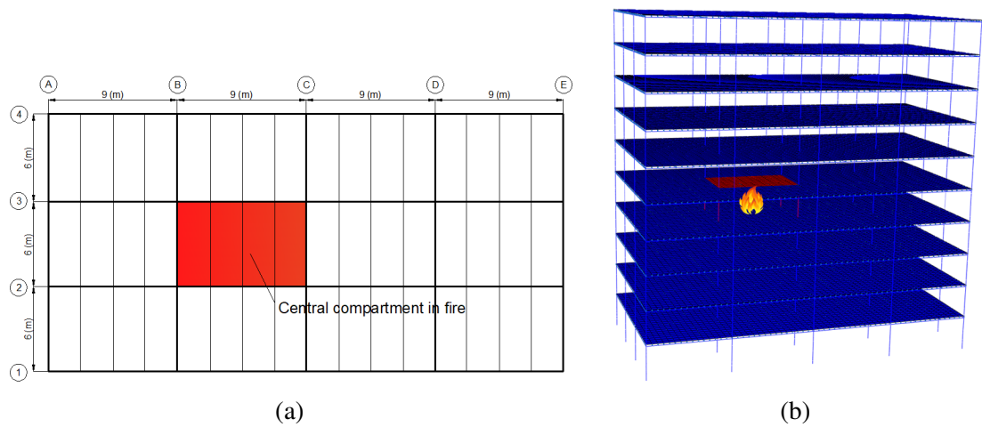
Fig. 5.44 Location of the central compartment fire at the mid-height of the building
