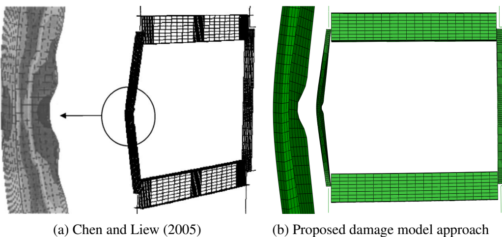
Fig. 4.38 Collapse modes of steel frame under blast loads
