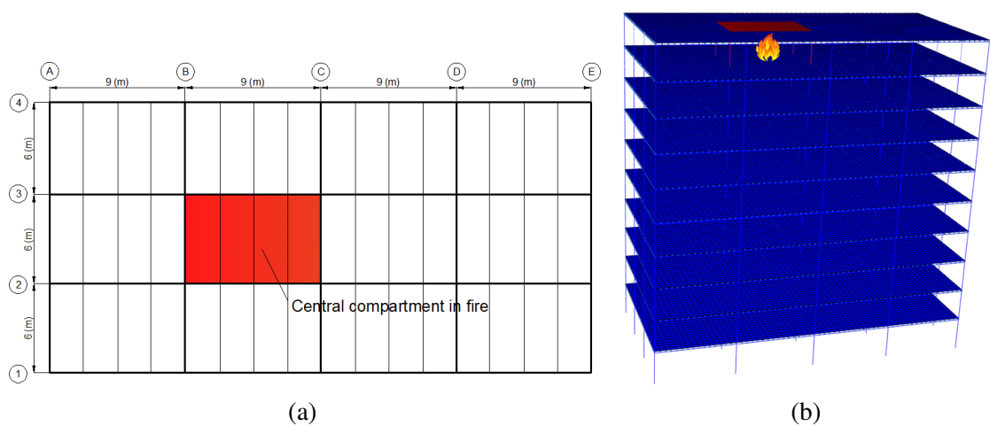
Fig. 5.50 Location of the central compartment fire on the top floor
