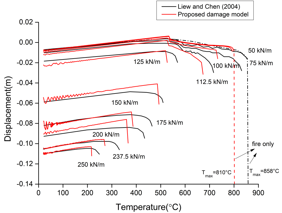
Fig. 4.33 Response of steel frame under explosion and followed by fire
