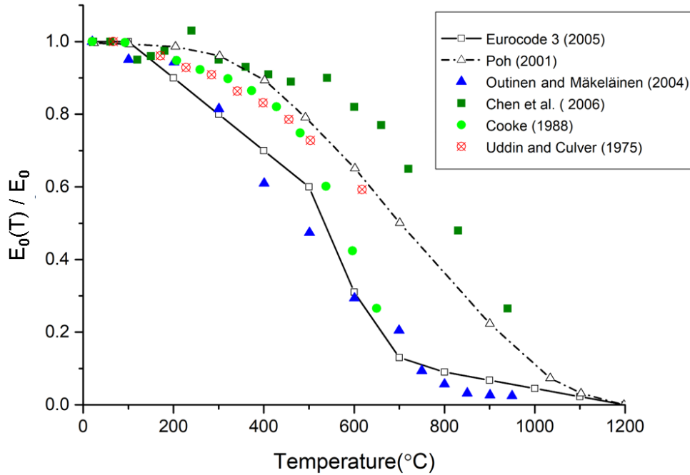
Fig. 2.6 Normalized elastic modulus of steel reported in literature sources
