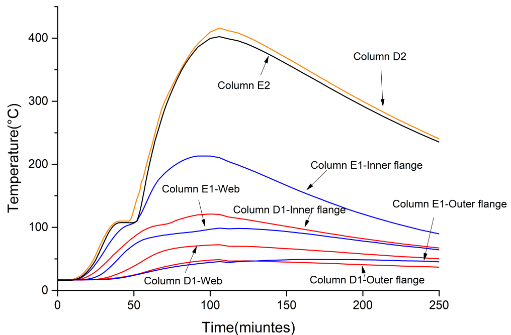
Fig. 4.47 Measured temperatures of columns (Lennon, 2003)
