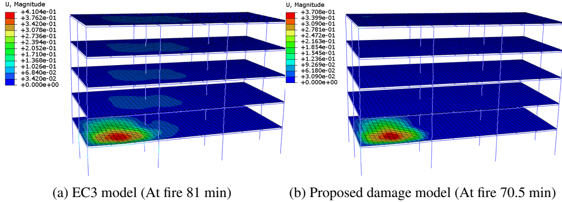
Fig. 5.13 The deformed shape of the building before column buckling initiates
