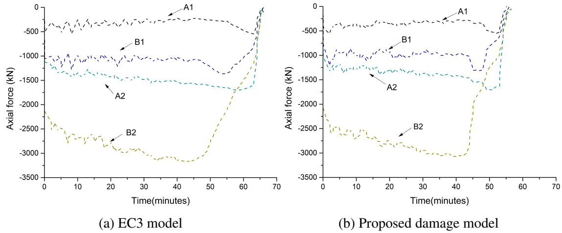
Fig. 5.76 Axial forces in columns during fire event
