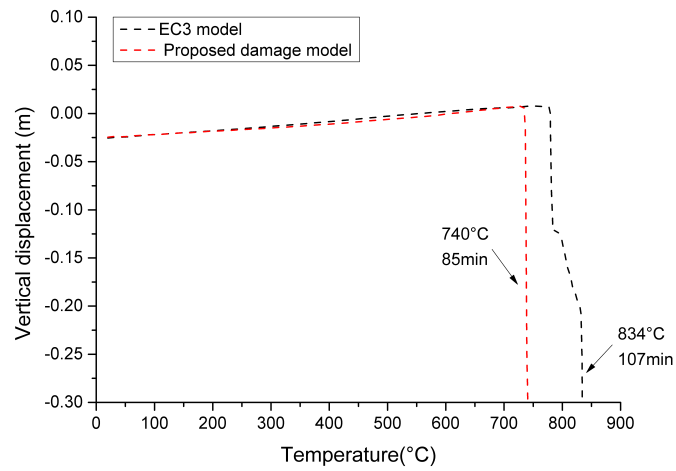
Fig. 5.48 Vertical displacement of the heated interior column B2
