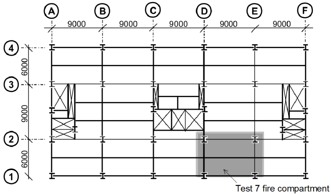
Fig. 4.42 The location of the fire compartment in Cardington fire test 7 (Lennon, 2003)
