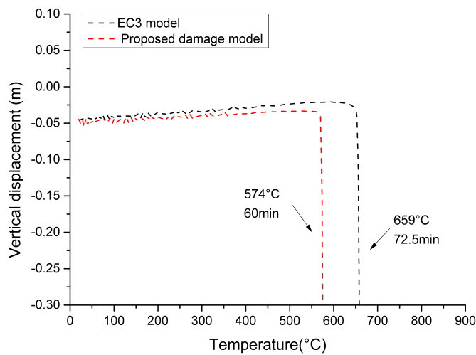
Fig. 5.85 Vertical displacement of the heated interior column B2
