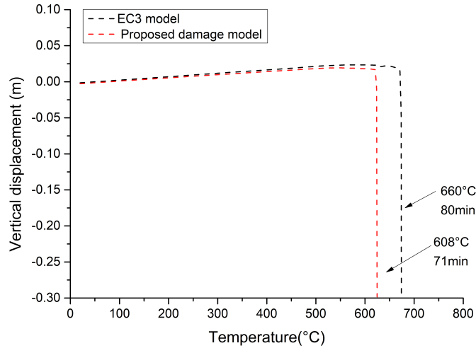
Fig. 5.17 Vertical displacement of the heated interior column B2
