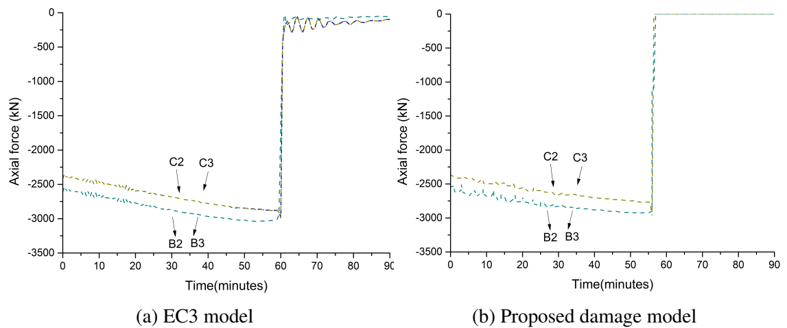
Fig. 5.46 Axial forces in columns during fire event
