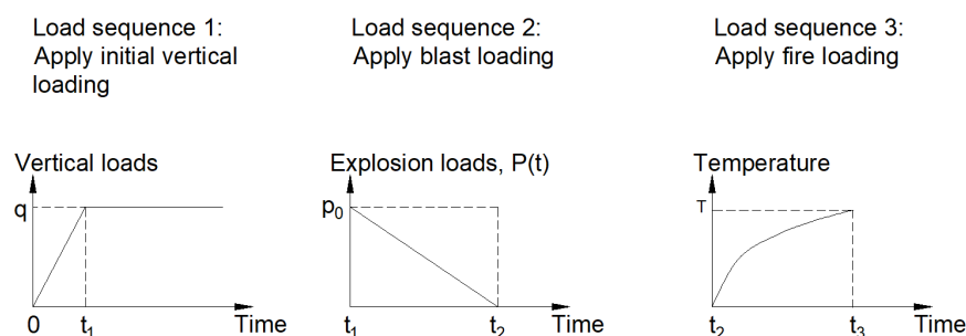
Fig. 5.8 Load sequences in post-blast fire analysis
