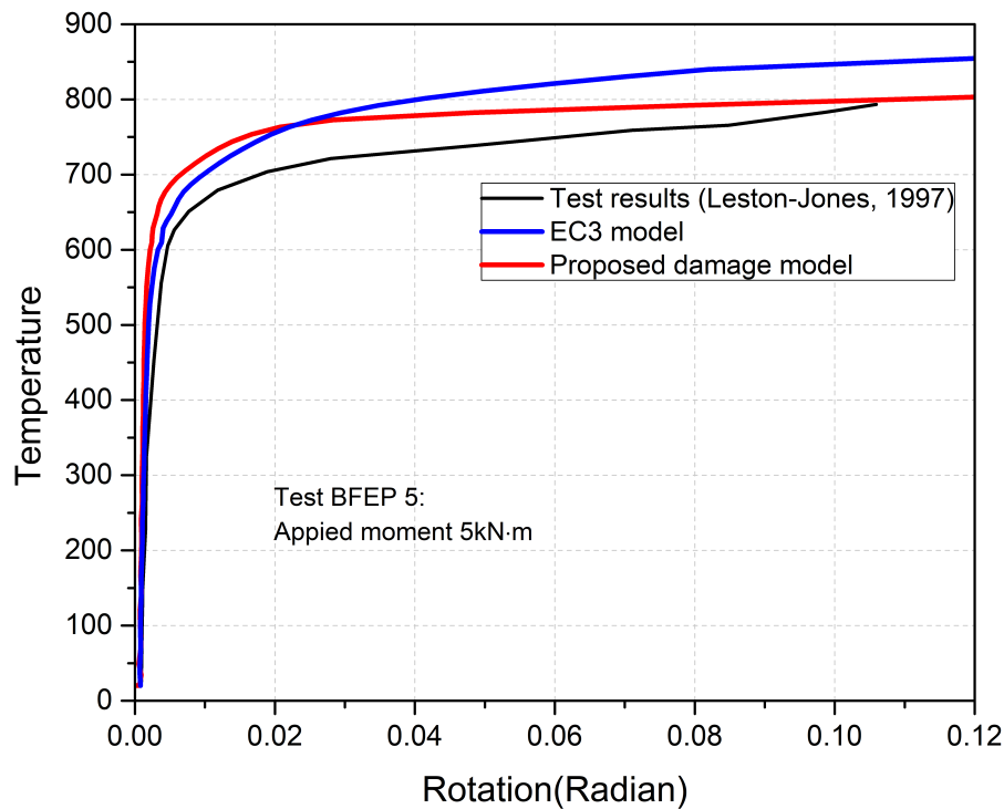
Fig. 4.16 Comparison of connection response between numerical cases and fire test 1 (BFEP5)
