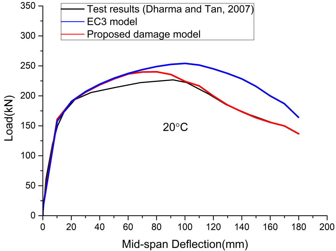
Fig. 4.4 Mid-span load–deflection of specimen S3-1
