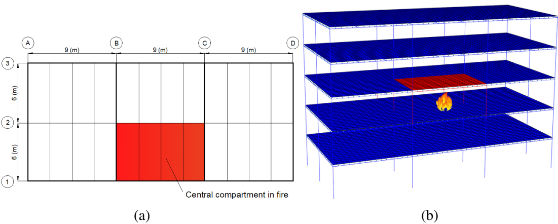
Fig. 5.24 Location of the central compartment fire at the mid-height of the building
