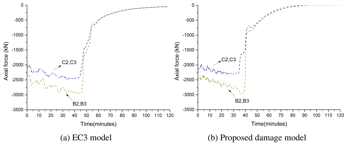
Fig. 5.80 Axial forces in columns during fire event
