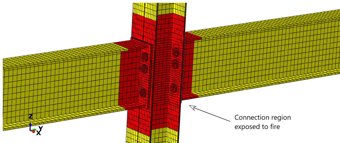
Fig. 4.14 Fire exposed region within connection model
