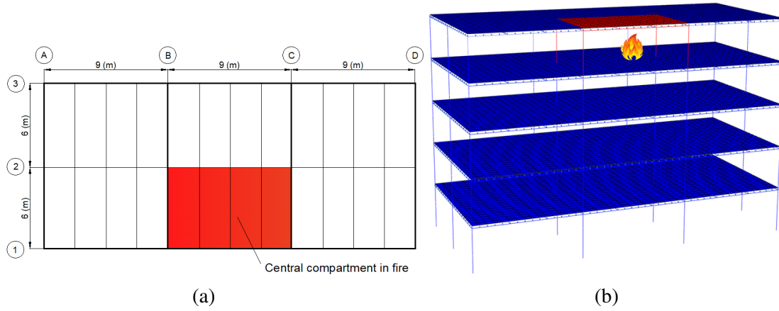
Fig. 5.30 Location of the central compartment fire on the top floor
