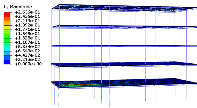
Fig. 5.53 Blast induced deformation after the blast analysis in the corner compartment on the ground floor
