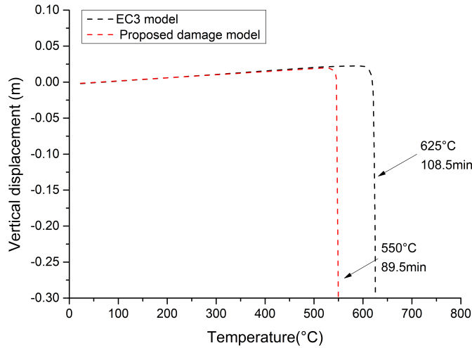
Fig. 5.34 Vertical displacement of the heated interior column B2
