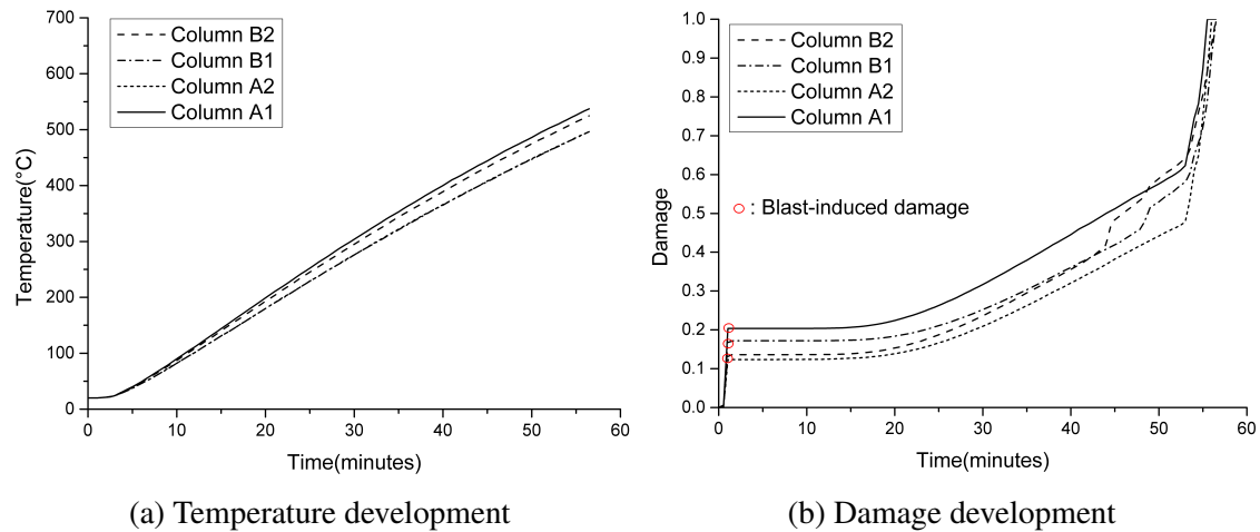
Fig. 5.77 Damage development in the top of columns subjected to blast and fire
