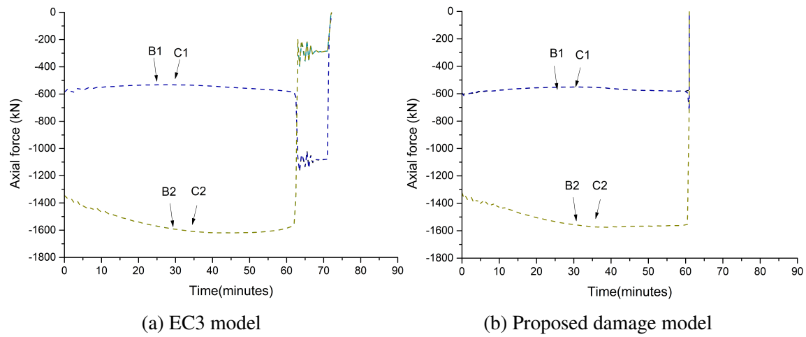
Fig. 5.26 Axial forces in columns during fire event
