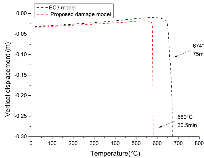
Fig. 5.68 Vertical displacement of the heated interior column B2
