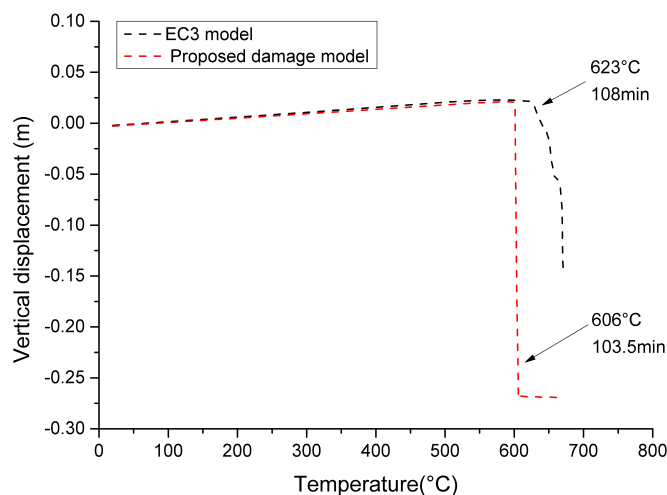
Fig. 5.39 Vertical displacement of the heated interior column B2
