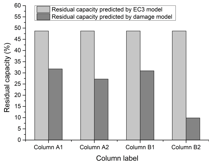
Fig. 5.23 Residual capacity of the heated columns upon column B2 buckling at 63 minutes of fire
