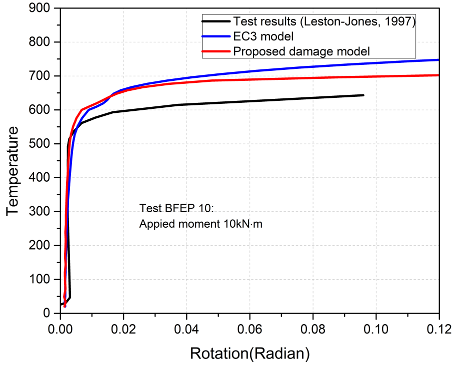
Fig. 4.17 Comparison of connection response between numerical cases and fire test 2 (BFEP10)
