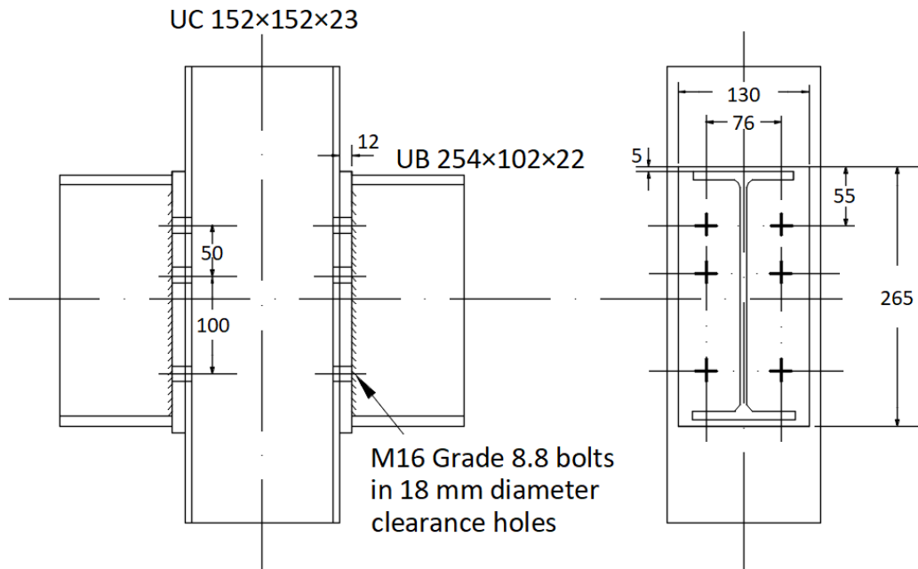
Fig. 4.8 Flush end plate connection detail (Leston-Jones, 1997)
