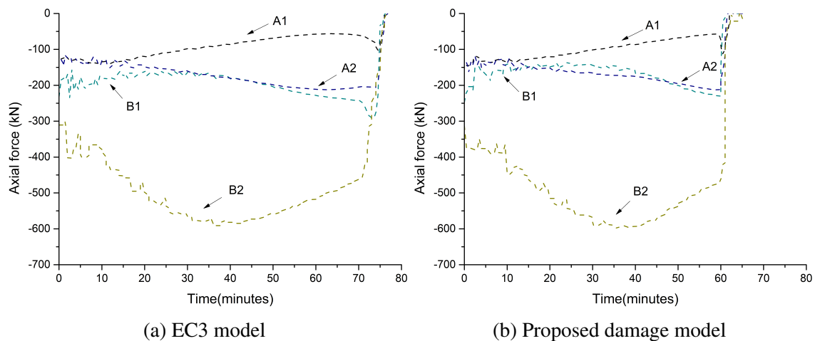
Fig. 5.69 Axial forces in columns during fire event
