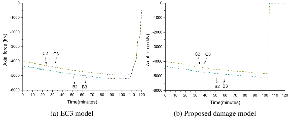
Fig. 5.40 Axial forces in columns during fire event
