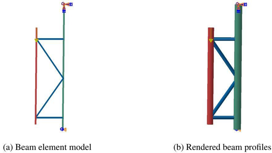
Fig. 4.22 Numerical model of steel tubular truss in ABAQUS
