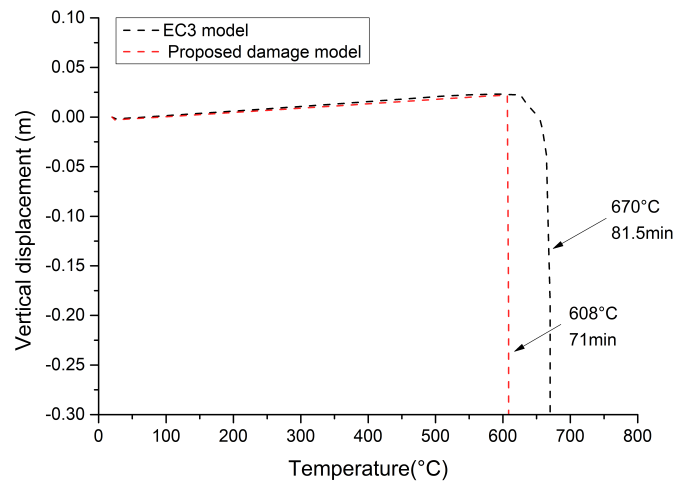
Fig. 5.12 Vertical displacement of the heated interior column B2
