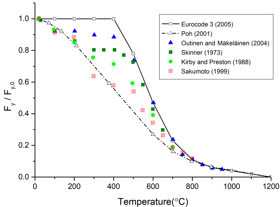
Fig. 2.5 Normalized yield strength of steel reported in literature sources
