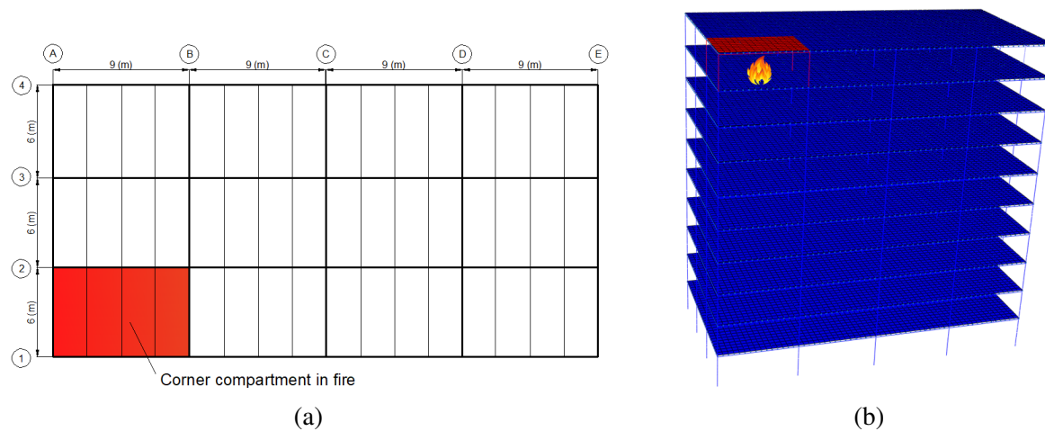
Fig. 5.47 Location of the corner compartment fire on the top floor
