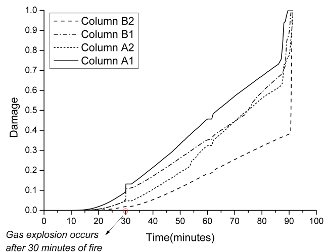
Fig. 5.94 Damage development in the top of blast-damaged columns
