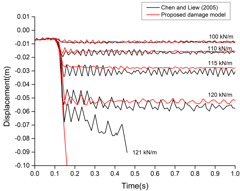
Fig. 4.37 Responses of steel frame under explosion only
