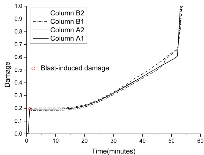
Fig. 5.63 Damage development in the top of blast-damaged columns
