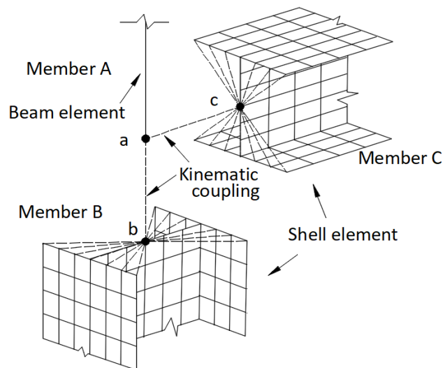
Fig. 4.35 Connecting techniques employed in the mixed element approach (Chen and Liew, 2005)
