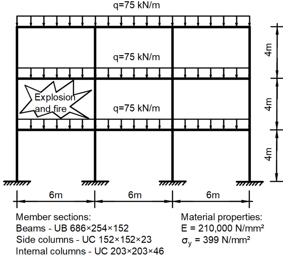
Fig. 4.27 Geometric configuration and loading of three-storey steel frame (Chen and Liew, 2005; Izzuddin et al., 2000; Liew and Chen, 2004)
