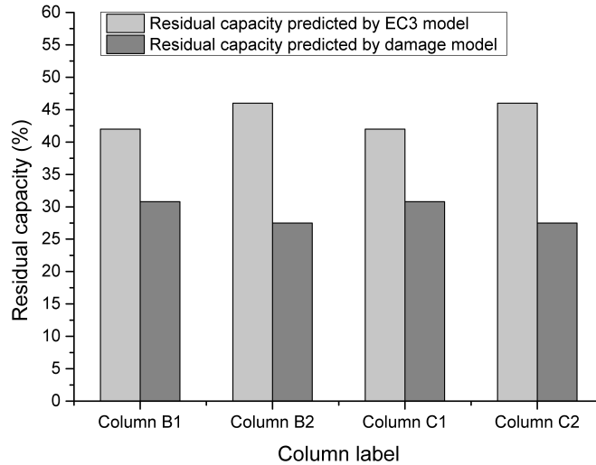
Fig. 5.19 Residual capacity of the heated columns upon interior column buckling at 71 minutes of fire
