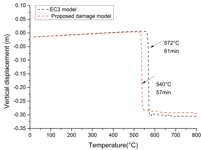
Fig. 5.45 Vertical displacement of the heated interior column B2
