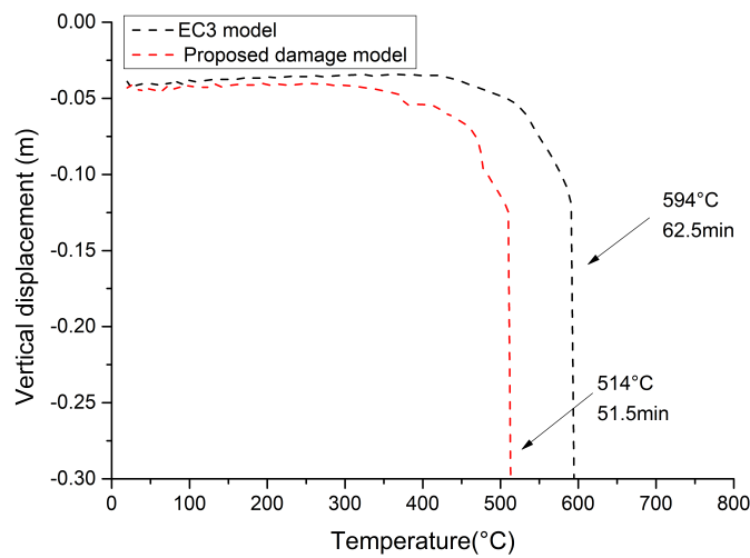
Fig. 5.61 Vertical displacement of the heated interior column B2
