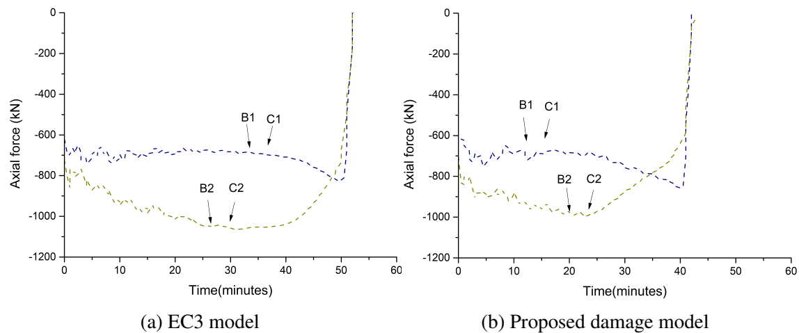
Fig. 5.66 Axial forces in columns during fire event
