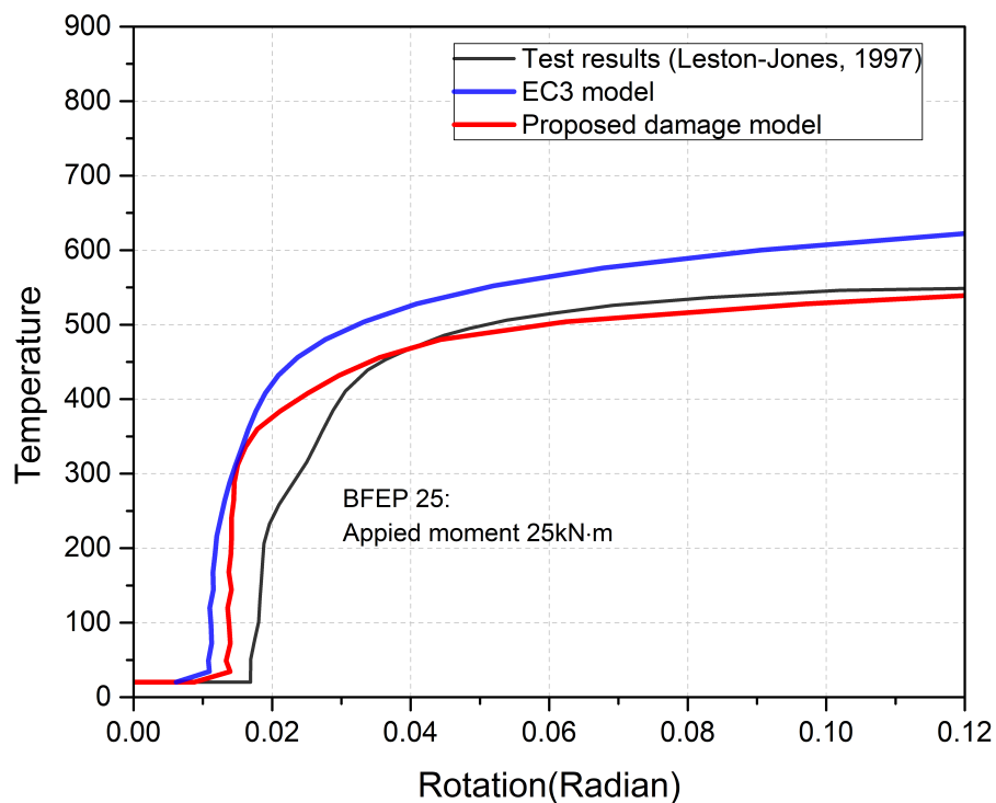
Fig. 4.20 Comparison of connection response between numerical cases and fire test 5 (BFEP25)
