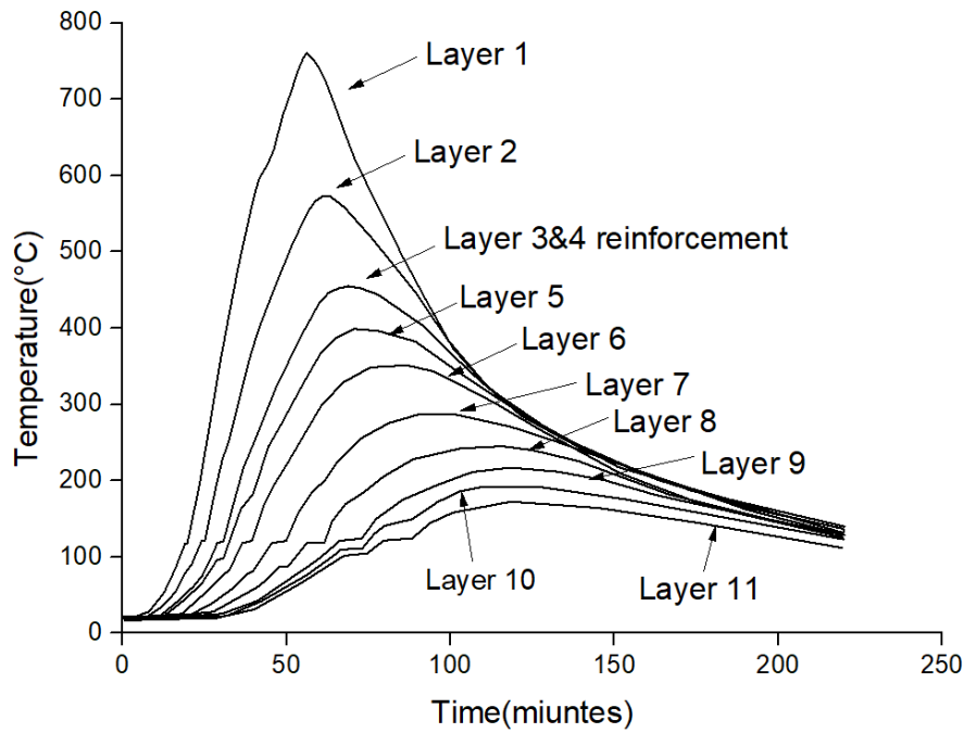
Fig. 4.48 Temperature variation throughout the depth of slab (Foster et al., 2007)
