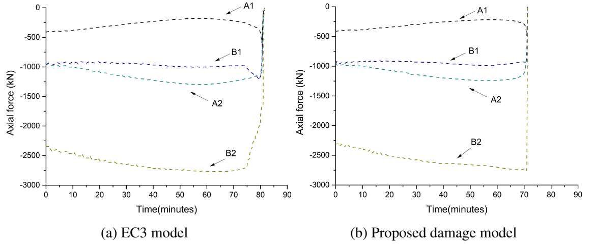
Fig. 5.14 Axial forces in columns during fire event
