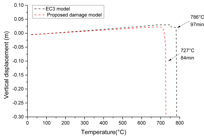
Fig. 5.31 Vertical displacement of the heated interior column B2
