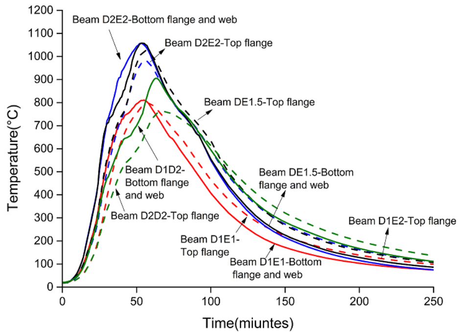
Fig. 4.46 Measured temperature distributions of beams (Lennon, 2003)
