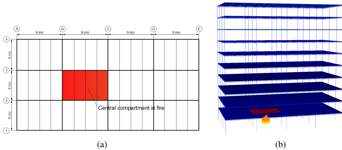
Fig. 5.38 Location of the central compartment fire on the ground floor
