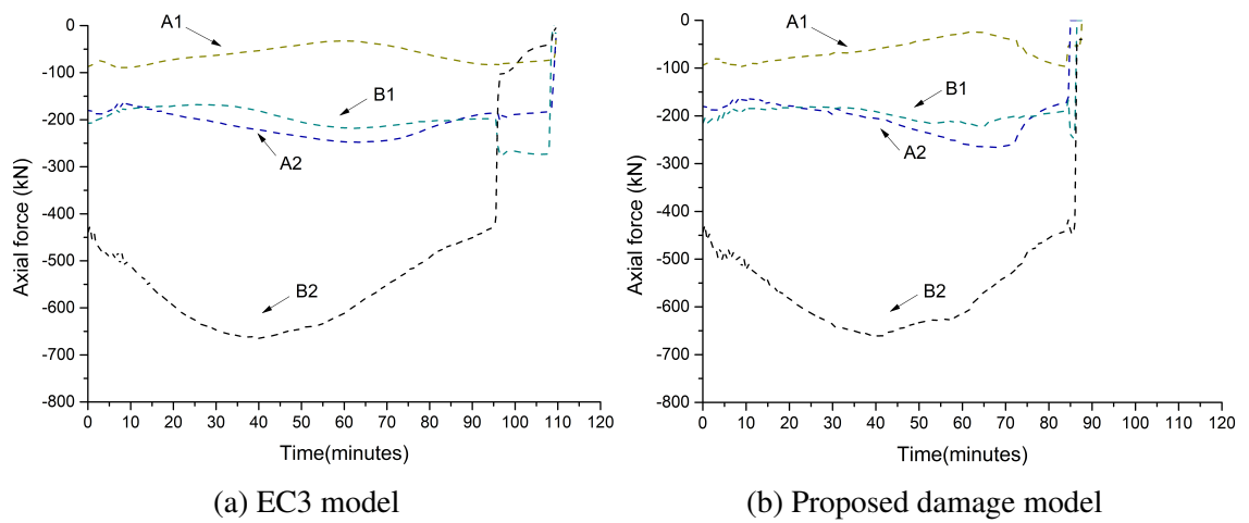
Fig. 5.49 Axial forces in columns during fire event
