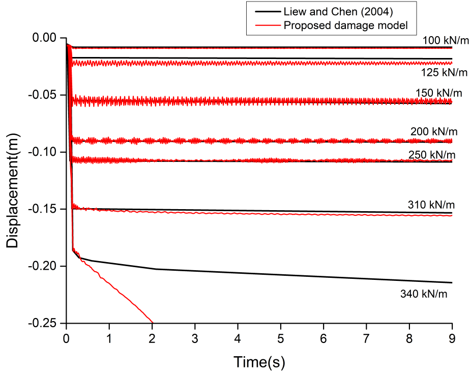
Fig. 4.31 Responses of steel frame under explosion only
