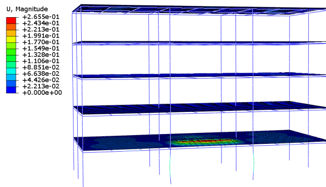
Fig. 5.57 Blast induced deformation after the blast analysis in the central compartment on the ground floor
