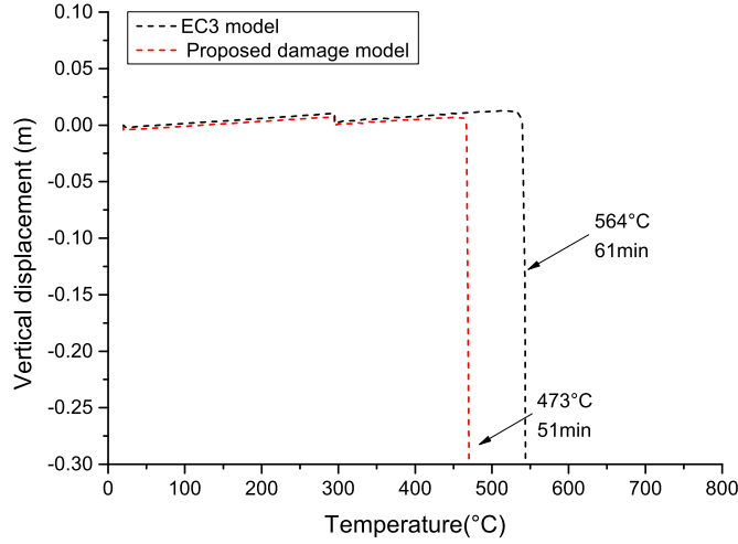
Fig. 5.88 Vertical displacement of the heated interior column B2
