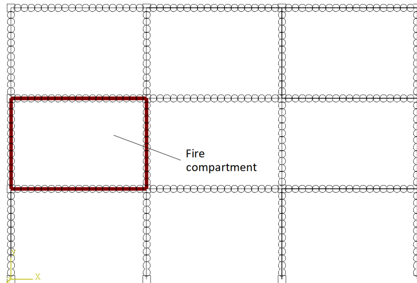
Fig. 4.30 FE beam element model of three-storey steel frame
