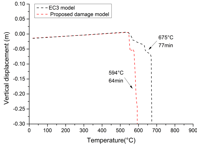
Fig. 5.42 Vertical displacement of the heated interior column B2
