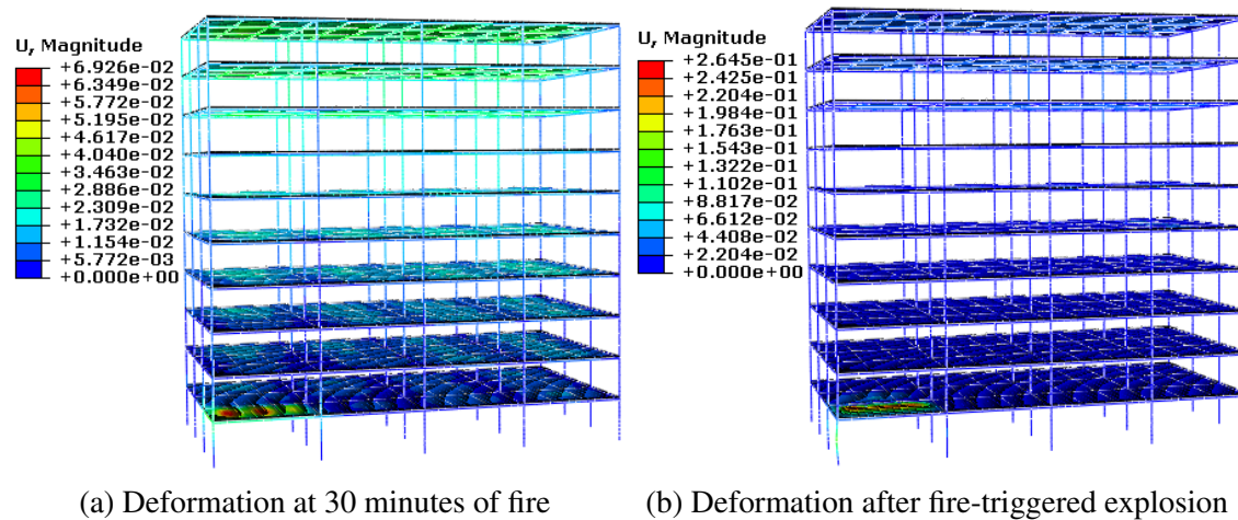
Fig. 5.91 Deformation before and after fire-triggered explosion occurrence
