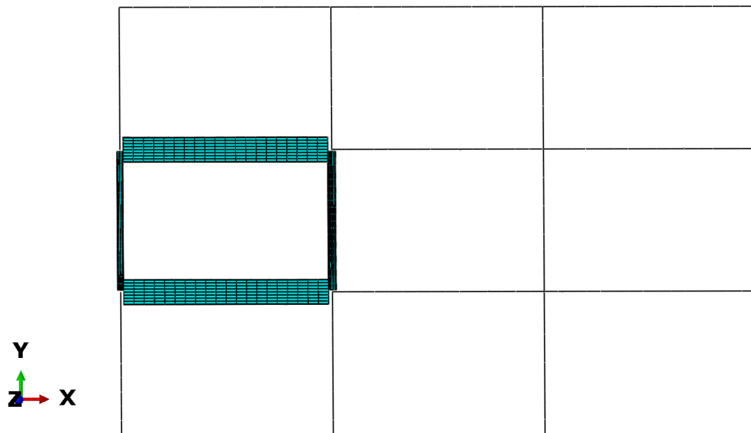
Fig. 4.36 FE mixed element model of three-storey steel frame
