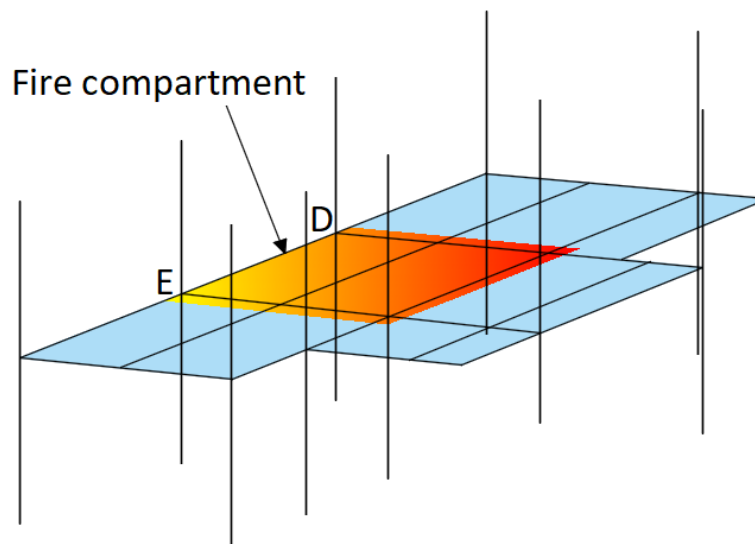
Fig. 4.43 The extent of the structure incorporated within the numerical model
