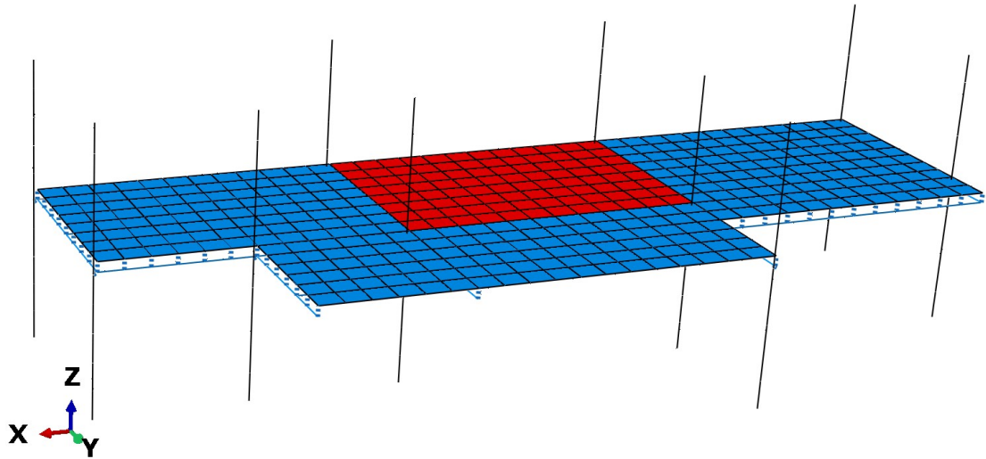
Fig. 4.44 FE model of Cardington test 7 in ABAQUS
