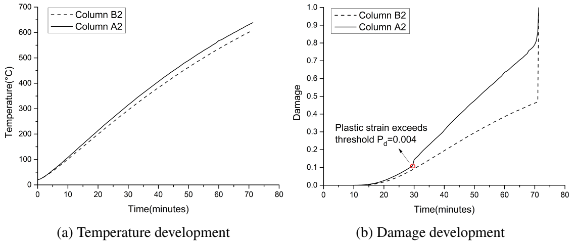
Fig. 5.15 Damage development in the top of column A2 and column B2
