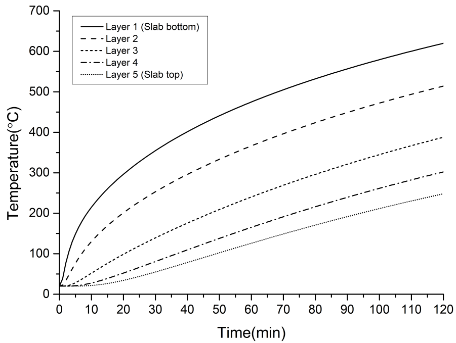
Fig. 5.5 Temperatures across concrete slab depth
