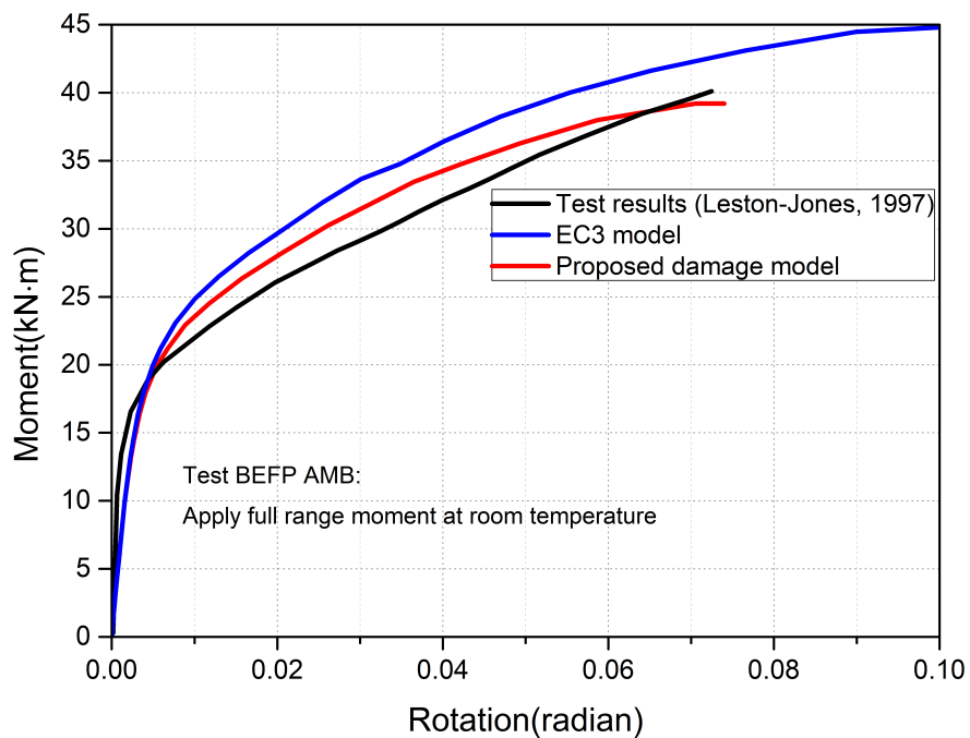
Fig. 4.11 Comparison of ambient-temperature connection response between numerical cases and test data
