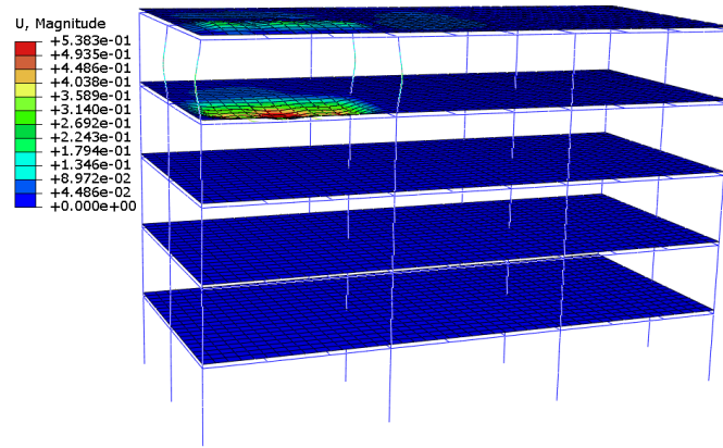
Fig. 5.67 Blast induced deformation after the blast analysis in the corner compartment on the top floor
