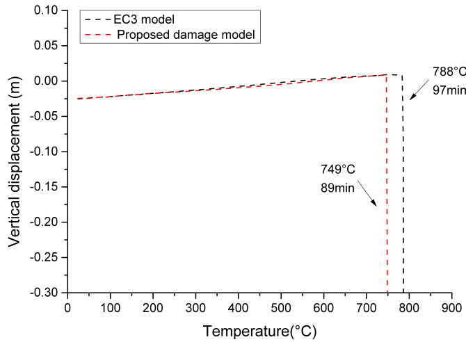
Fig. 5.51 Vertical displacement of the heated interior column B2
