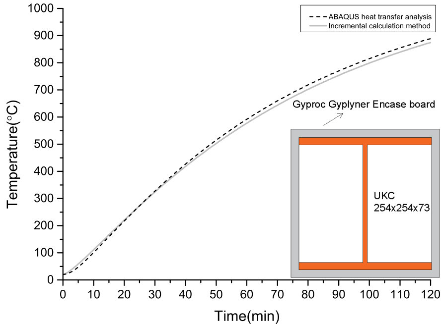
Fig. 5.3 Comparison of temperature histories of UKC254x254x73
