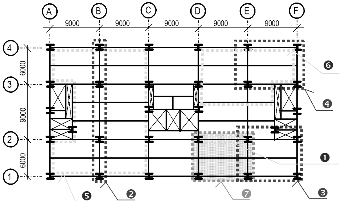
Fig. 2.4 Floor layout and location of the fire tests (Foster et al., 2007)
