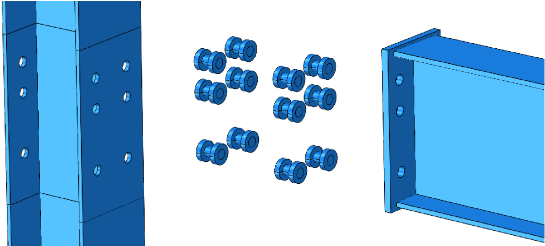
Fig. 4.10 Modelling details of flush end plate connection
