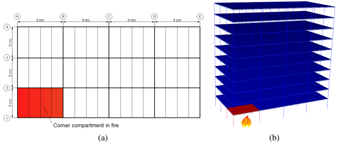
Fig. 5.33 Location of the corner compartment fire on the ground floor
