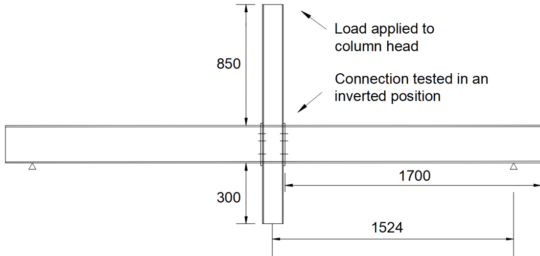
Fig. 4.7 Ambient-temperature test arrangement (Leston-Jones, 1997)
