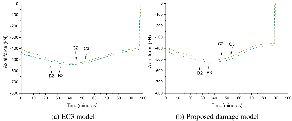
Fig. 5.52 Axial forces in columns during fire event
