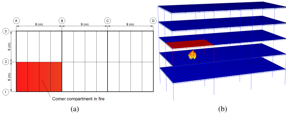
Fig. 5.20 Location of the corner compartment fire at the mid-height of the building
