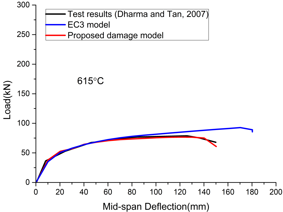
Fig. 4.6 Mid-span load-deflection of specimen S3-3
