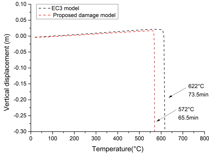
Fig. 5.58 Vertical displacement of the heated interior column B2
