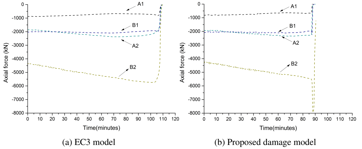
Fig. 5.36 Axial forces in columns during fire event
