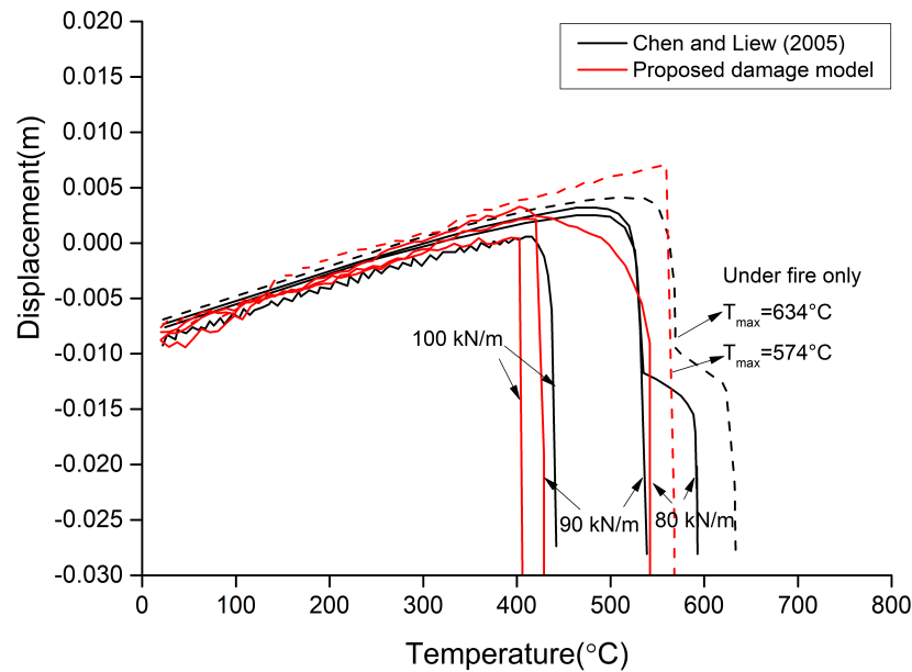
Fig. 4.39 Response of steel frame under explosion and followed by fire
