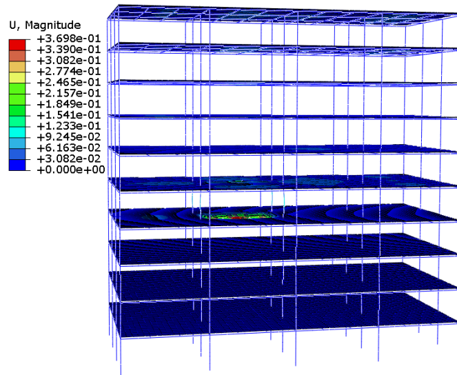
Fig. 5.78 Blast induced deformation after the blast analysis in the central compartment on the fifth floor
