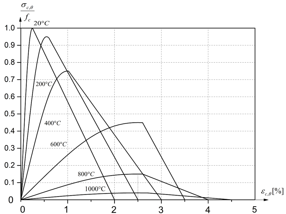
Fig. 4.49 Stress-strain relationships of concrete at elevated temperatures (EN 1994-1-2, 2005)
