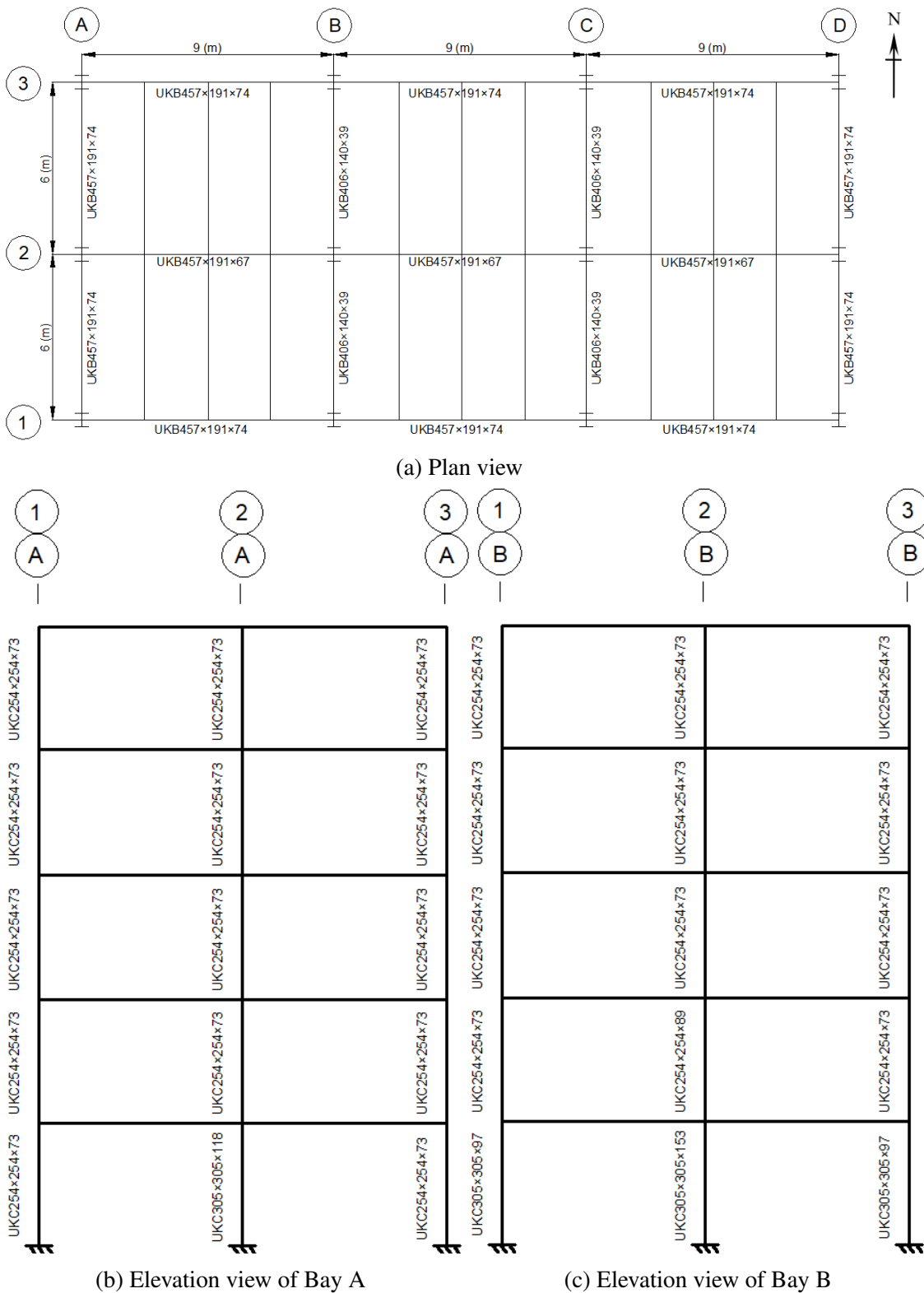
Fig. 5.1 Schematic view of the five-storey building structural design
