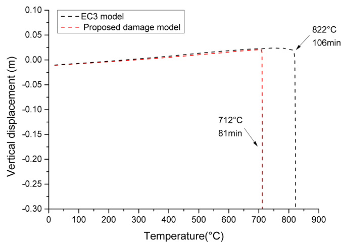
Fig. 5.28 Vertical displacement of the heated interior column B2
