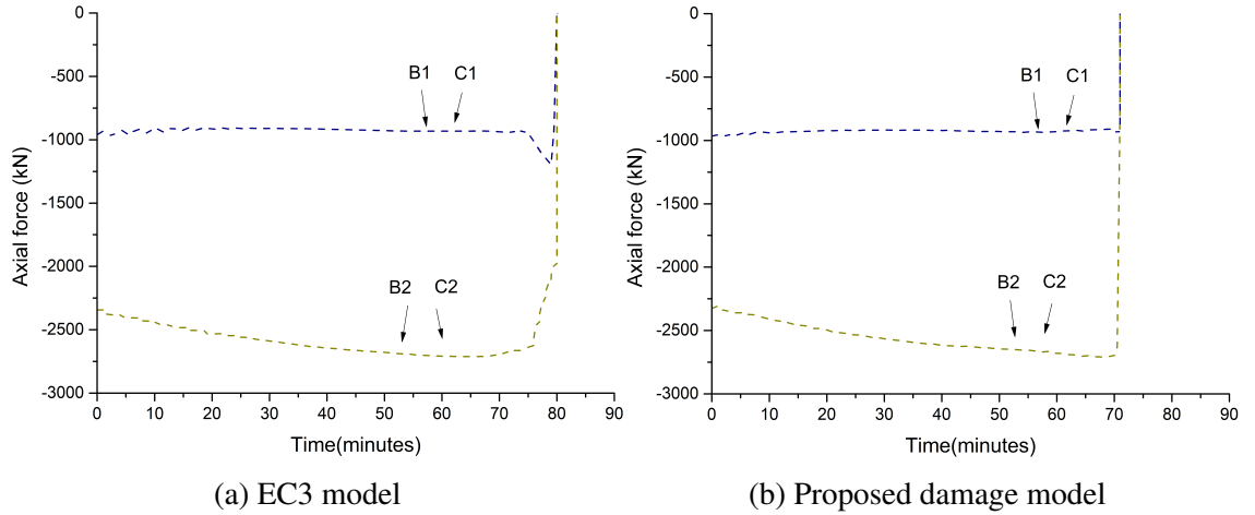
Fig. 5.18 Axial forces in columns during fire event
