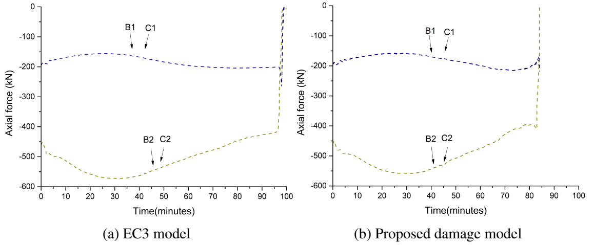
Fig. 5.32 Axial forces in columns during fire event
