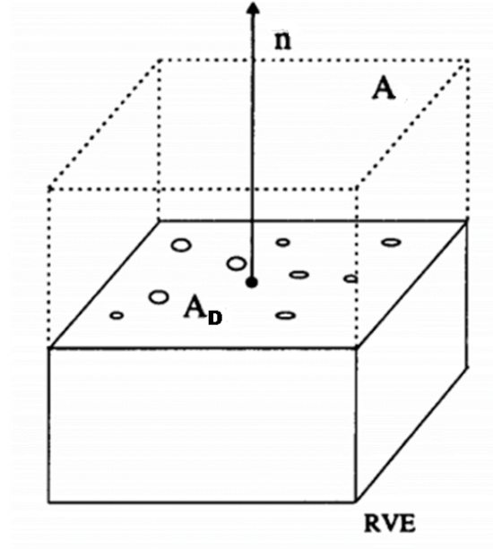
Fig. 2.9 Damaged element (Lemaitre, 1985)
