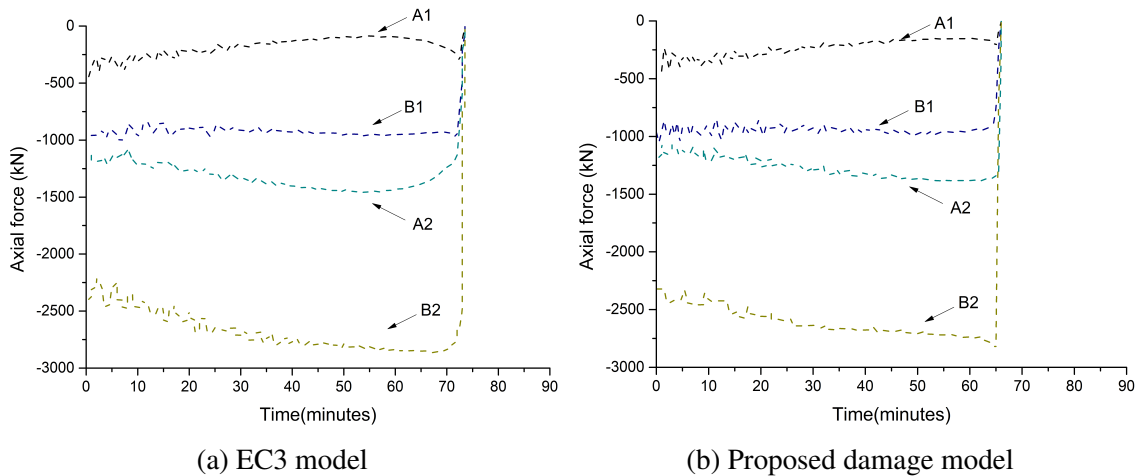
Fig. 5.55 Axial forces in columns during fire event
