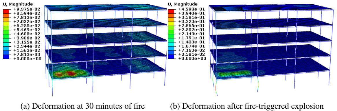
Fig. 5.87 Deformation before and after fire-triggered explosion occurrence
