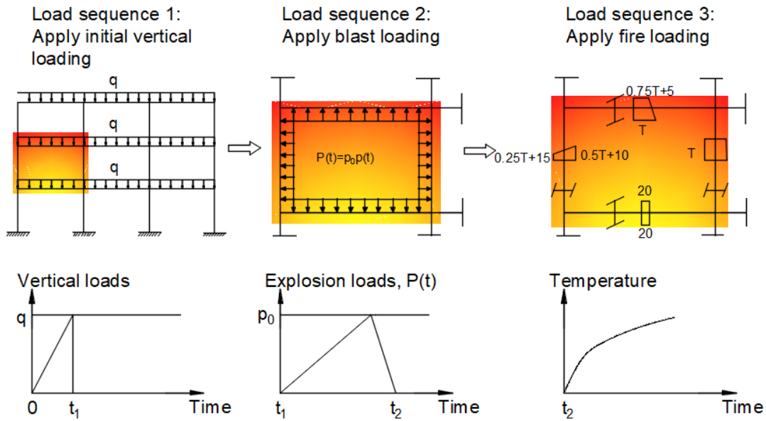
Fig. 4.28 Load sequences in explosion and fire analysis
