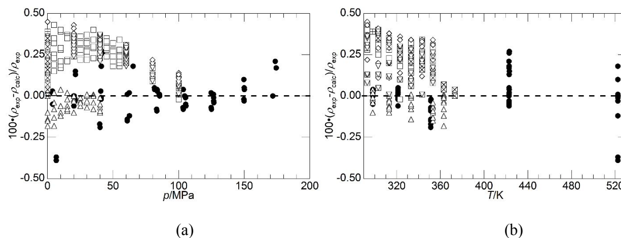
Figure 8. Comparison of experimental 2,2,4,4,6,8,8-heptamethylnonane (HMN) densities, \rho_{\text{exp}} , obtained in the present study and other studies to Tait calculated densities, \rho_{\text{calc}} . ● - This study, □ - Cannet et al. 31 , ◇ - Barrahou et al. 63 , △ - Et-Tahir et al. 32 , ▽ - Zeberg-Mikkelsen et al. 37 , ⊠ - Fermeglia and Torriano 33 , and ⊞ - Lunning-Prak et al. 36, 64, 65 .
