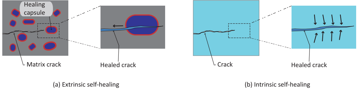
Figure 1: Schematic of (a) a capsule-based extrinsic self-healing material: A matrix crack is attracted towards the healing capsule, which upon fracture releases the healing agent into the crack, resulting in crack healing and (b) an intrinsic self-healing material: the healing agent is available directly from the material chemical composition. The material that fills the crack is typically different than the matrix material for both the extrinsic and intrinsic cases.
