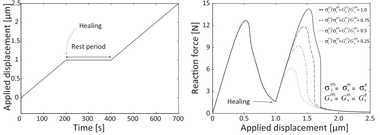
(a) Time history of the specified displacement. (b) Reaction force vs. applied displacement
