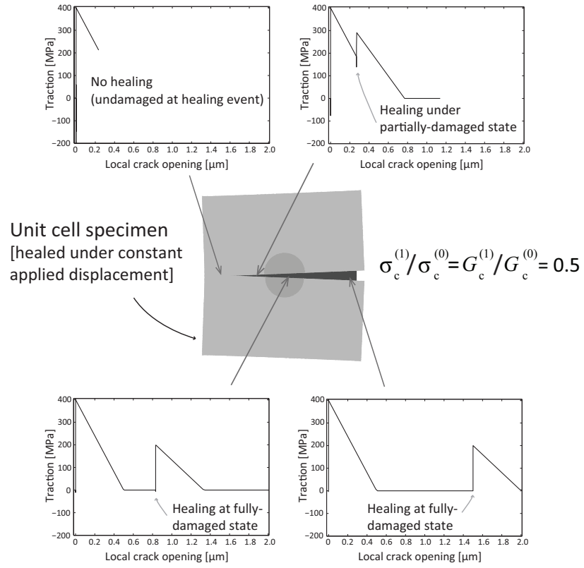
Figure 10: Unit cell specimen at the final state of the applied loading given in Fig. 9a. Representative local response curves illustrate how the introduction of a shift in the (local) crack opening displacement accounts for the proper origin upon resumption of the load after healing.
