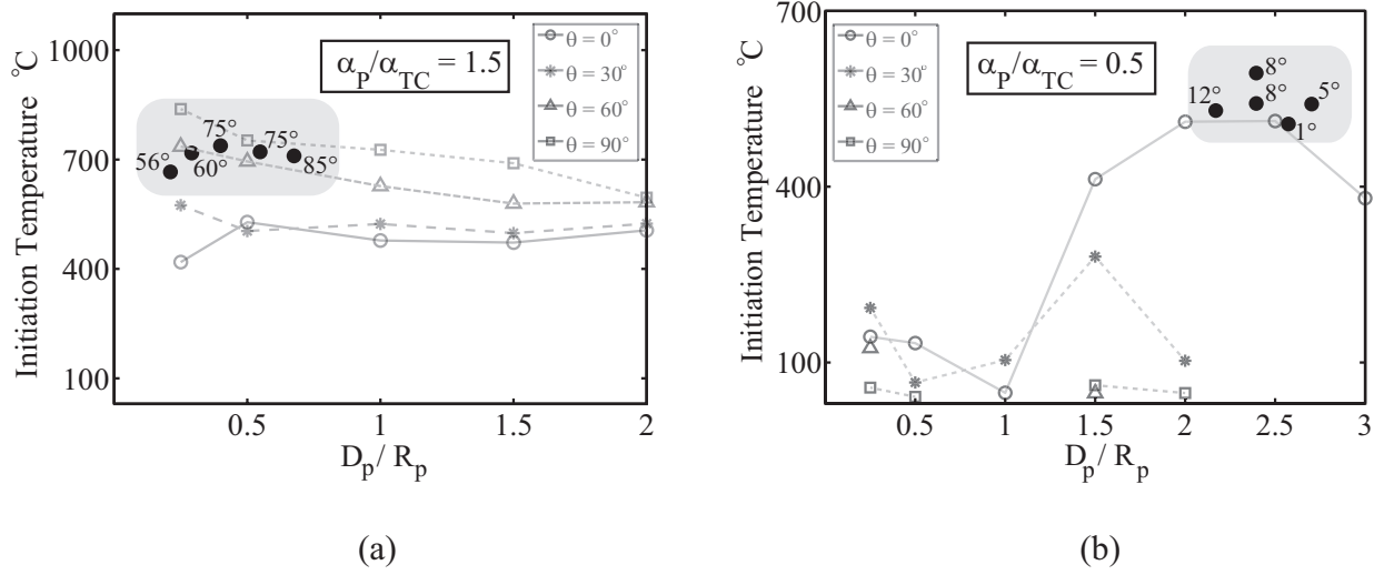
Figure 7: Correlation of crack initiation temperature of multiparticle simulation with two particle simulation case for \alpha_P/\alpha_{TC} = 0.5 and 1.5 . This figure is analogous to Fig. 4, but the new data points marks the crack initiation temperature of multiparticle simulations (five different realisations) along with the angular dependence.
