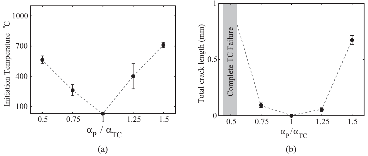
Figure 6: Variation of (a) crack initiation temperature and (b) total crack length for different CTE mismatch ratios \alpha_P / \alpha_{TC} = 1.5, 1.25, 1, 0.75 and 0.5 . For the CTE mismatch ratio of 0.5 , there is a complete failure of the TC before reaching the final temperature ( 30^\circ\text{C} ) as indicated by a grey shade.
