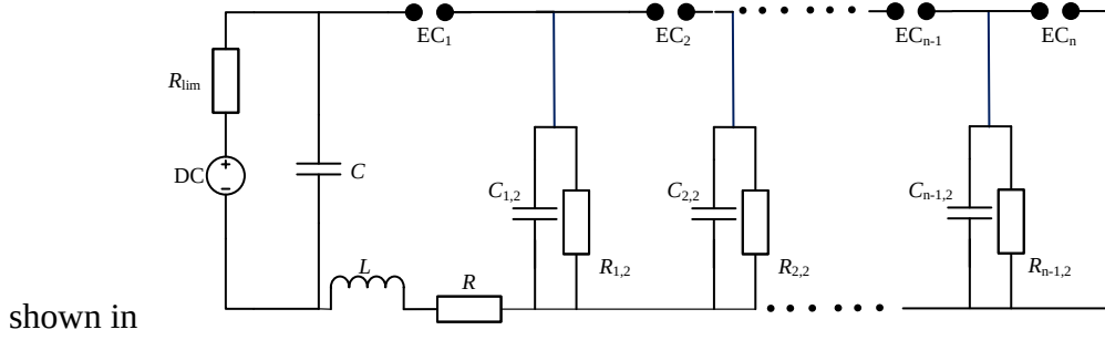
shown in Fig. 1. A high voltage DC power system is adopted as the power supply. The discharge frequency can be adjusted by changing the current limiting resistor R_{lim} . The inductance L represents the wire inductance. The inductance R represents the wire resistance and the equivalent series resistance of the capacitor C . The discharge energy is controlled by the capacitor C and the breakdown voltage of the first electrode couple (EC) EC_1 . The relay capacitor, C_{1,2} , C_{2,2} , ..., C_{n-1,2} , and the resistor, R_{1,2} , R_{2,2} , ..., R_{n-1,2} are used to relay the high voltage and ensure the multichannel discharge.
