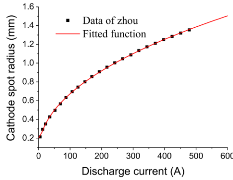
Fig. 8 Cathode spot radius at different discharge currents
