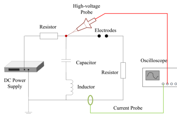
Fig. 9 Experiment system
