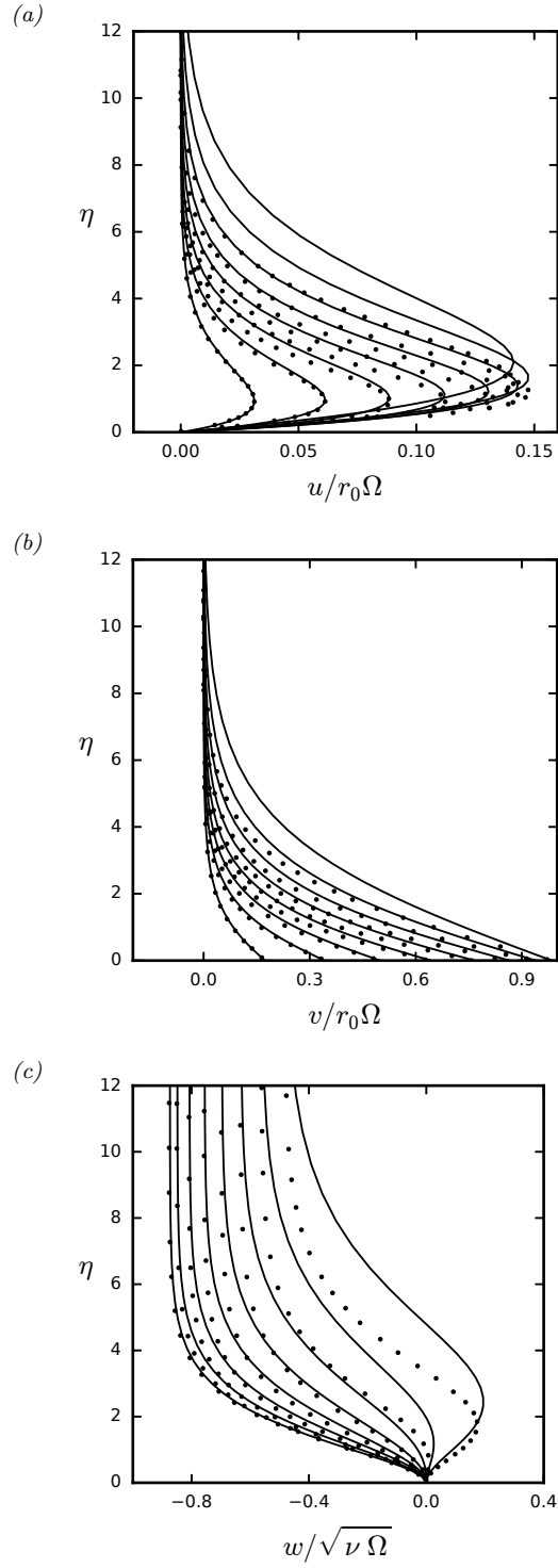
Figure 10: Comparison of the velocity profiles on a rotating prolate spheroid (in still air) with eccentricity 0.7 at \theta from 10^\circ \rightarrow 80^\circ in 10^\circ increments (left to right), obtained using the present approach, with those reported by Samad and Garrett (2010) ( \cdot ); \eta as defined in equation (13d).
