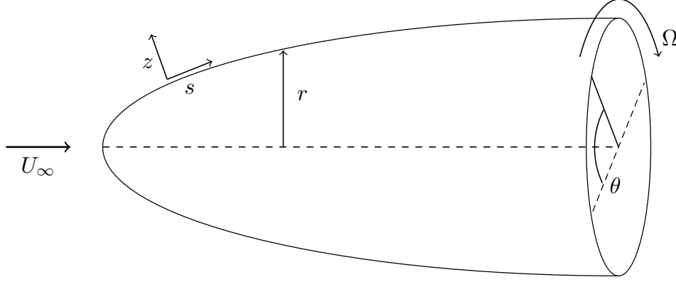
Figure 1: Sketch of the co-ordinate system for generalised body of revolution.
