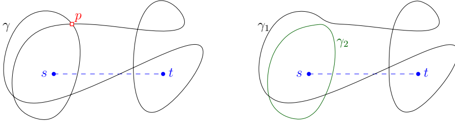
Fig. 7 Uncrossing argument in the proof of Lemma 6.
