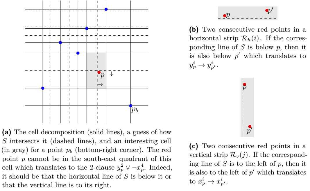
■ Figure 6 Illustration of the algorithm and the two kinds of clauses of the 2-SAT instance.
