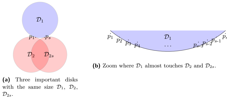
Figure 5 The disks \mathcal{D}_1 , \mathcal{D}_2 , \mathcal{D}_{2s} and the convex chain p_1, p_2, \dots, p_s . The curvature of the boundary of \mathcal{D}_1 is exaggerated in the zoom for the sake of clarity.
