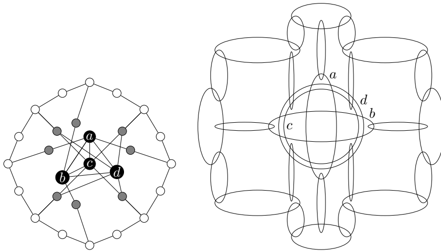
■ Figure 12 A graph (left), which has a representation with empty ellipses (right) but no representation with convex sets.
