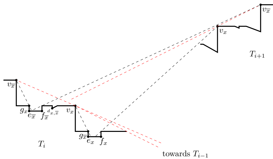
■ Figure 9 The inverter gadget. We omit the superscripts i and i + 1 . If a guard should be placed on at least one vertex among v_{x,x}^i and v_x^i (for \ell \in \{i, i + 1\} ), then the two ways of seeing the four vertices e_{x,x}^i, f_{x,x}^i, e_x^i, f_x^i with three guards are \{v_{x,x}^i, g_{x,x}^i, v_x^i\} and \{v_x^i, g_x^i, v_{x,x}^{i+1}\} .
