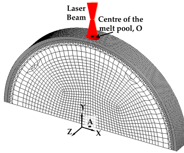
Figure 1. Meshed model of the half solid cylindrical specimen with 10\ \text{mm} diameter and 1\ \text{mm} length, where laser beam irradiating on the surface created melt pool; point O is the centre of the melt pool and A is the centre of the half cylindrical specimen.
