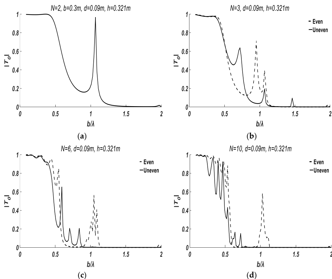
Figure 8. The influence of plate arrangement on the transmission coefficient of progressive waves. (a) Plate number N = 2 . (b) Plate number N = 3 . (c) Plate number N = 6 . (d) Plate number N = 10 .
