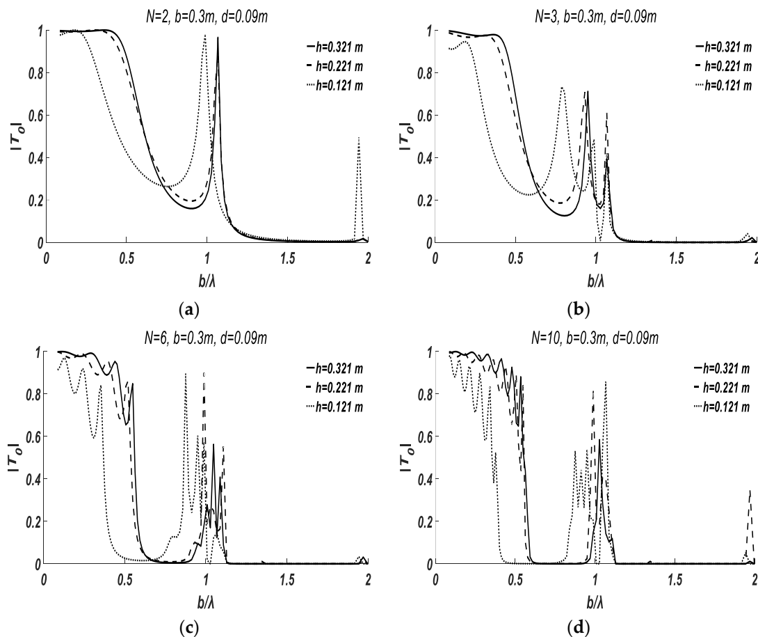
Figure 7. The influence of plate draft to water depth ratio on the transmission coefficient of progressive waves. (a) Plate number N = 2 . (b) Plate number N = 3 . (c) Plate number N = 6 . (d) Plate number N = 10 .
