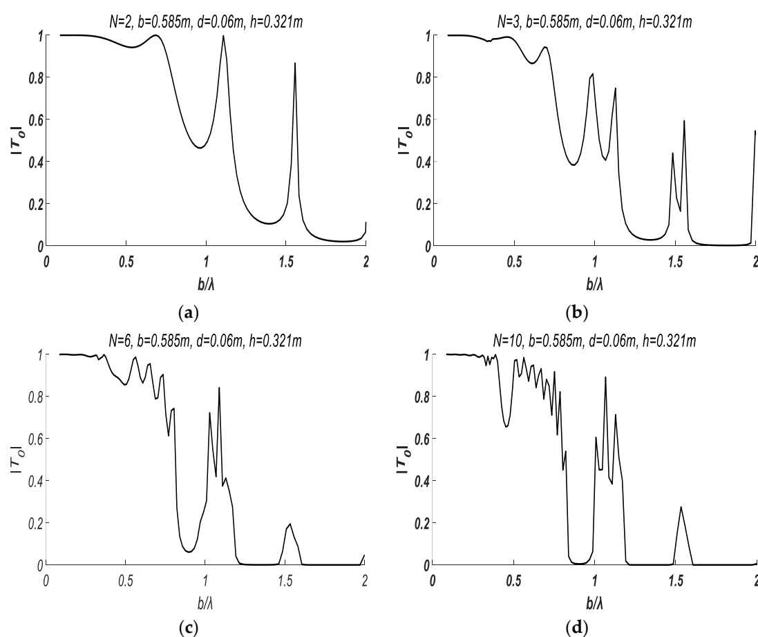
Figure 6. The transmission coefficient of progressive waves under different number of plates. (a) Plate number N = 2 . (b) Plate number N = 3 . (c) Plate number N = 6 . (d) Plate number N = 10 .
