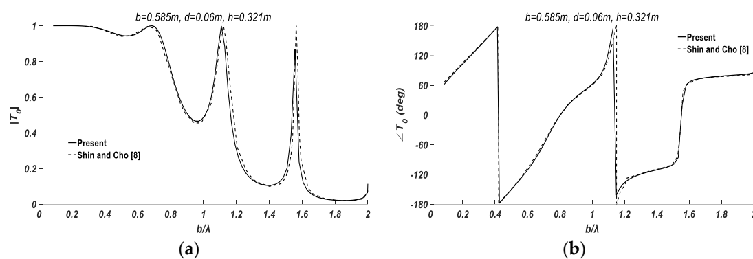
Figure 2. Comparison of the transmission coefficient of progressive waves obtained using the present numerical model with the numerical results from Shin and Cho [8]. (a) The amplitude of the coefficient |T_0| ; and (b) the phase of the coefficient \angle T_0 .
