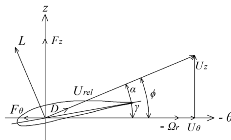
Figure 2. Cross-sectional airfoil element.
