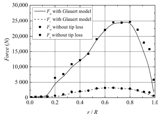
Figure 12. Comparison of radial force distributions with Glauert model and without the tip loss model.
