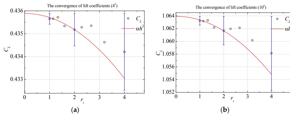
Figure 5. Convergence of the lift coefficient with the grid refinement (Fits obtained from the data with 1 \leq r_i \leq 2 ) by different attack angles: (a) 4^\circ ; (b) 10^\circ . Blue line: Error bar.
