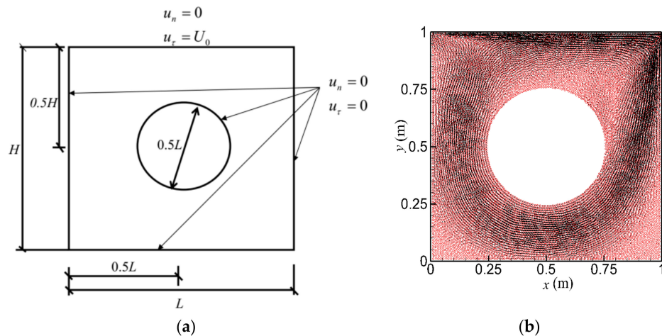
Figure 11. (a) Schematic setup of the lid-driven flow model with a cylinder inside; and (b) Velocity vector plot of the cavity flow at time t = 40 s. Red, location of fluid particle; Black, velocity of flow field.
