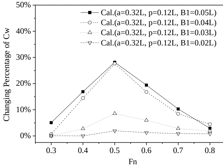
Fig. 33. Relative differences between computed results with and without considering SOZ for Tri A with different side hull breadths. (a) Sinkage, (b) Trim, (c) Wave making resistance.
