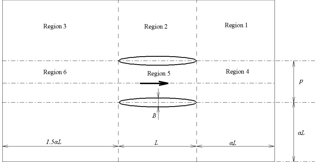
Fig. 34. Domain size of catamaran
