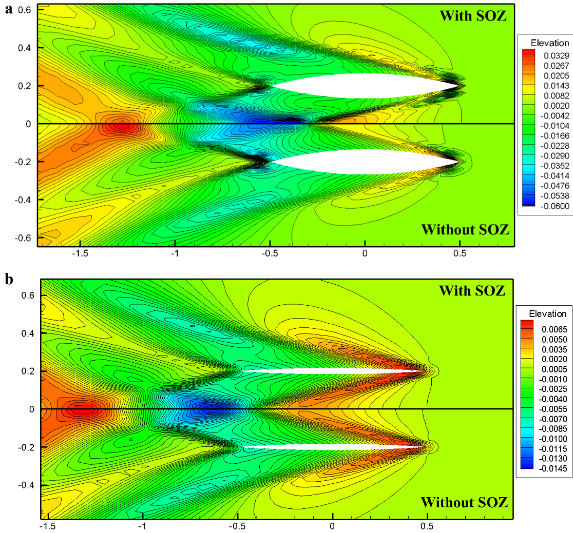
Fig. 40. Wave pattern of the catamaran with p = 0.4L at F_n = 0.7 . (a) B/L = 0.133 , (b) B/L = 0.067 .
