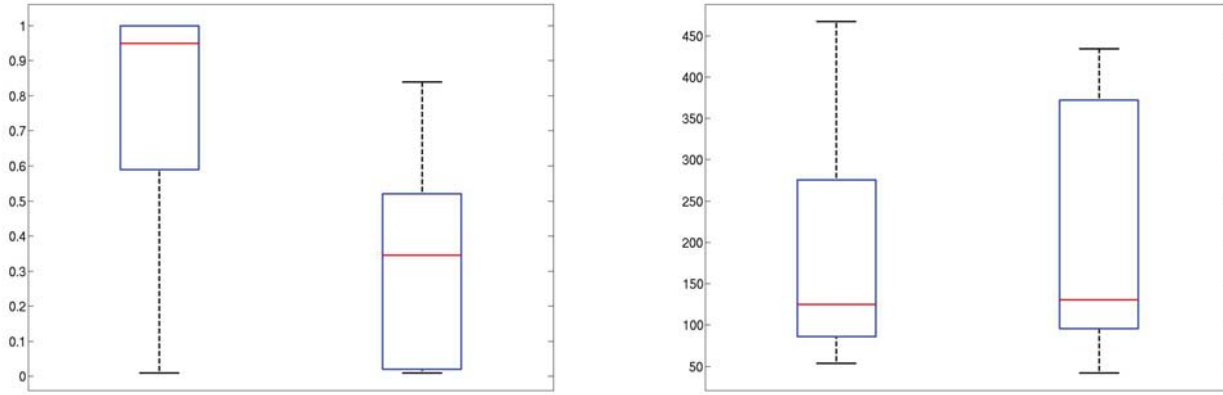
Figure A.2: Conditional probability of success and runtime of (\mu + \lambda)\text{EA}_{KBS} vs (\mu + \lambda)\text{EA}_{KBS} on the Rastrigin test function
