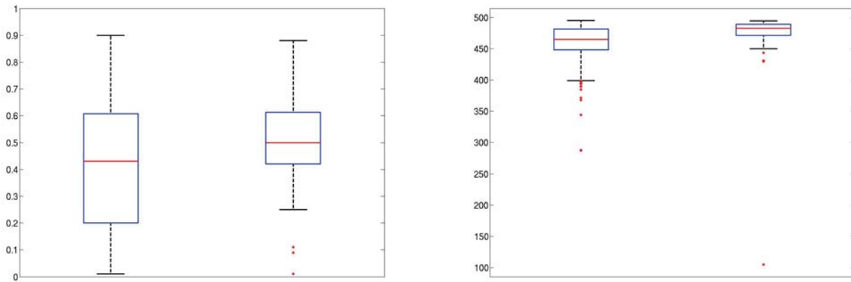
Figure A.9: Probability of success (\mu + \lambda)EA_{KBS} vs (\mu + \lambda)EA_{\sim KBS} on the random k-means clustering problem
