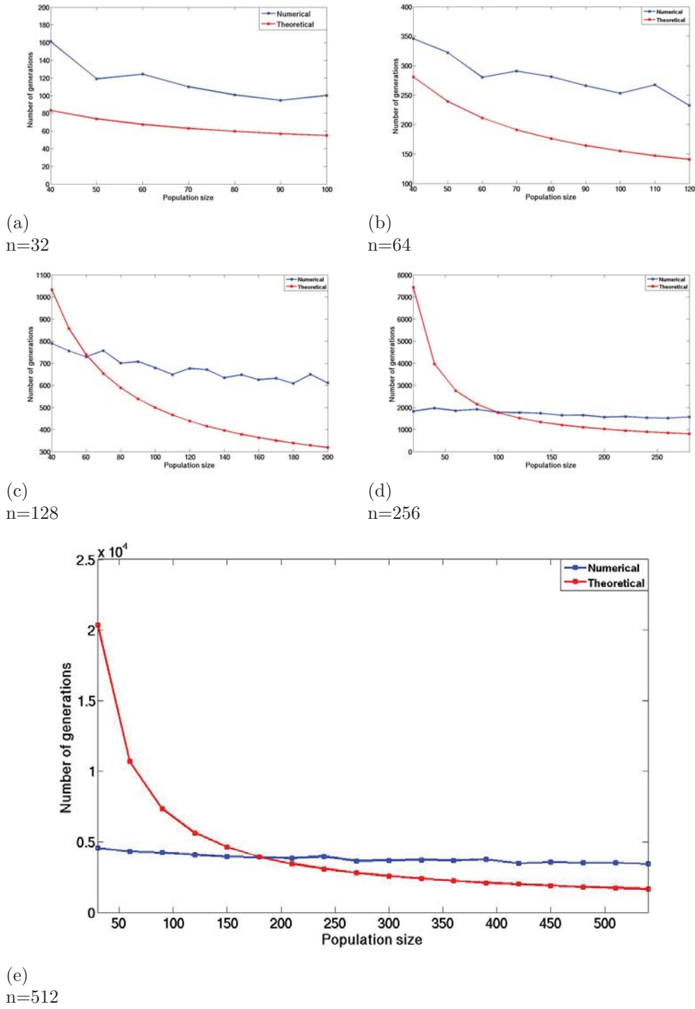
Figure 4.14: Theoretical and numerical bounds for (\mu + \lambda)EA_{IBS} solving Royal Roads Test Function
