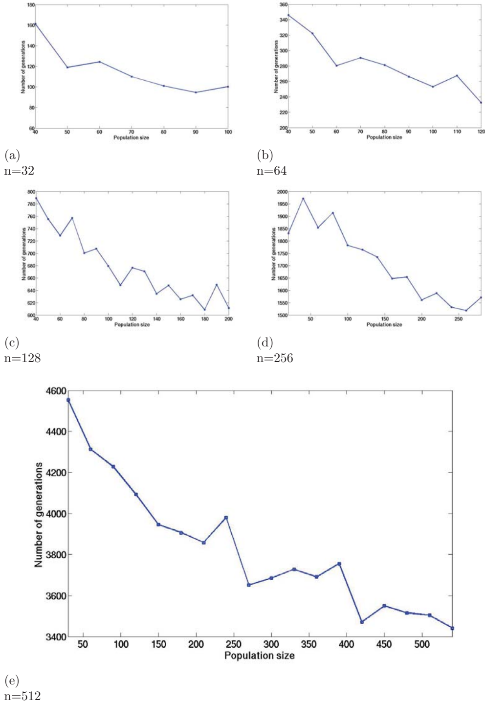
Figure 4.12: Numerical runtime estimate for (\mu + \lambda)\text{EA}_{1BS} solving Royal Roads Test Function for different population sizes. The positive effect of the population size measured in the number of generations is obvious.
