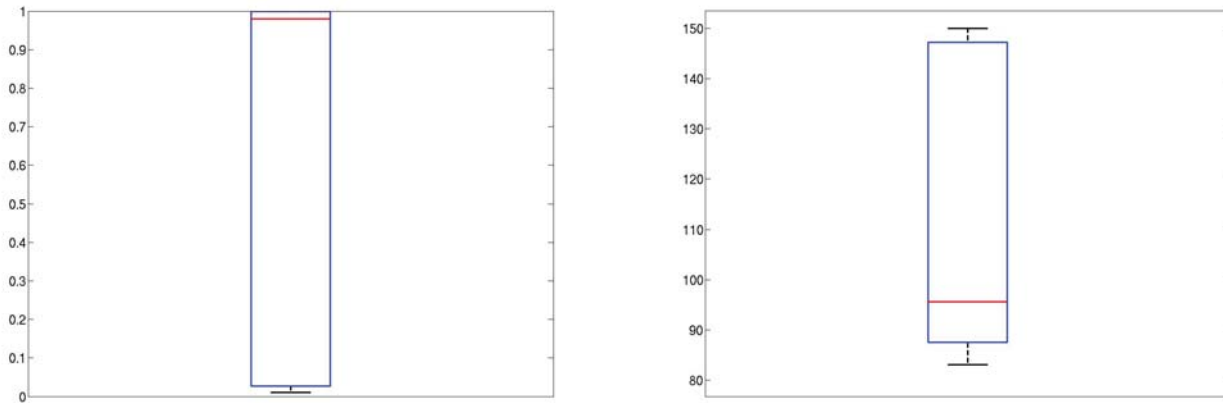
Figure A.4: Conditional probability of success and runtime (\mu + \lambda)\text{EA}_{KBS} on the Royal Roads test function. Algorithms with other parameter settings do not solve the problem in the set number of generations.
