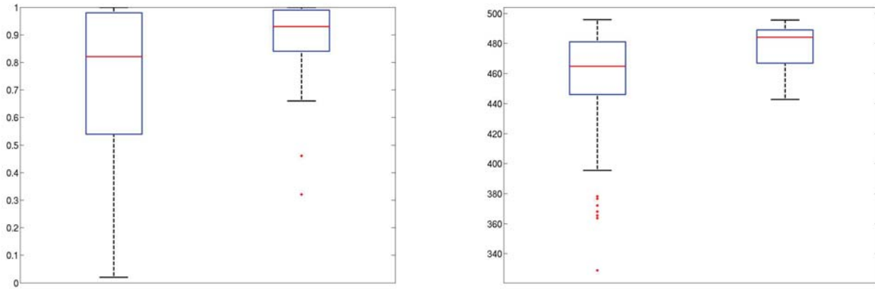
Figure A.8: Probability of success (\mu + \lambda)EA_{KBS} vs (\mu + \lambda)EA_{\sim KBS} on the trivial k-means clustering problem
