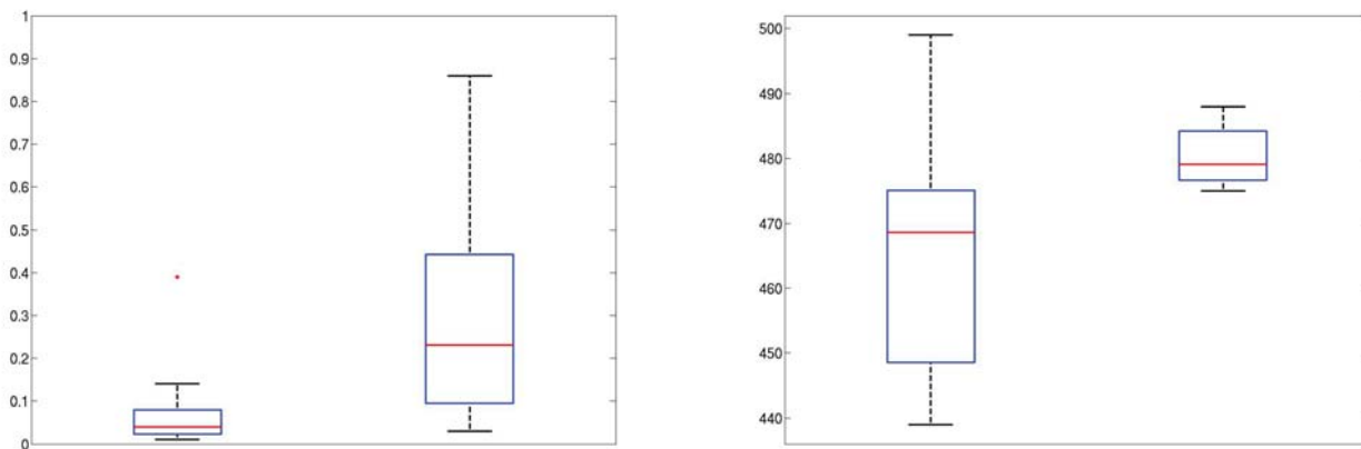
Figure A.5: Conditional probability of success and runtime of (\mu + \lambda)\text{EA}_{KBS} vs (\mu + \lambda)\text{EA}_{KBS} on the Four Peaks test function
