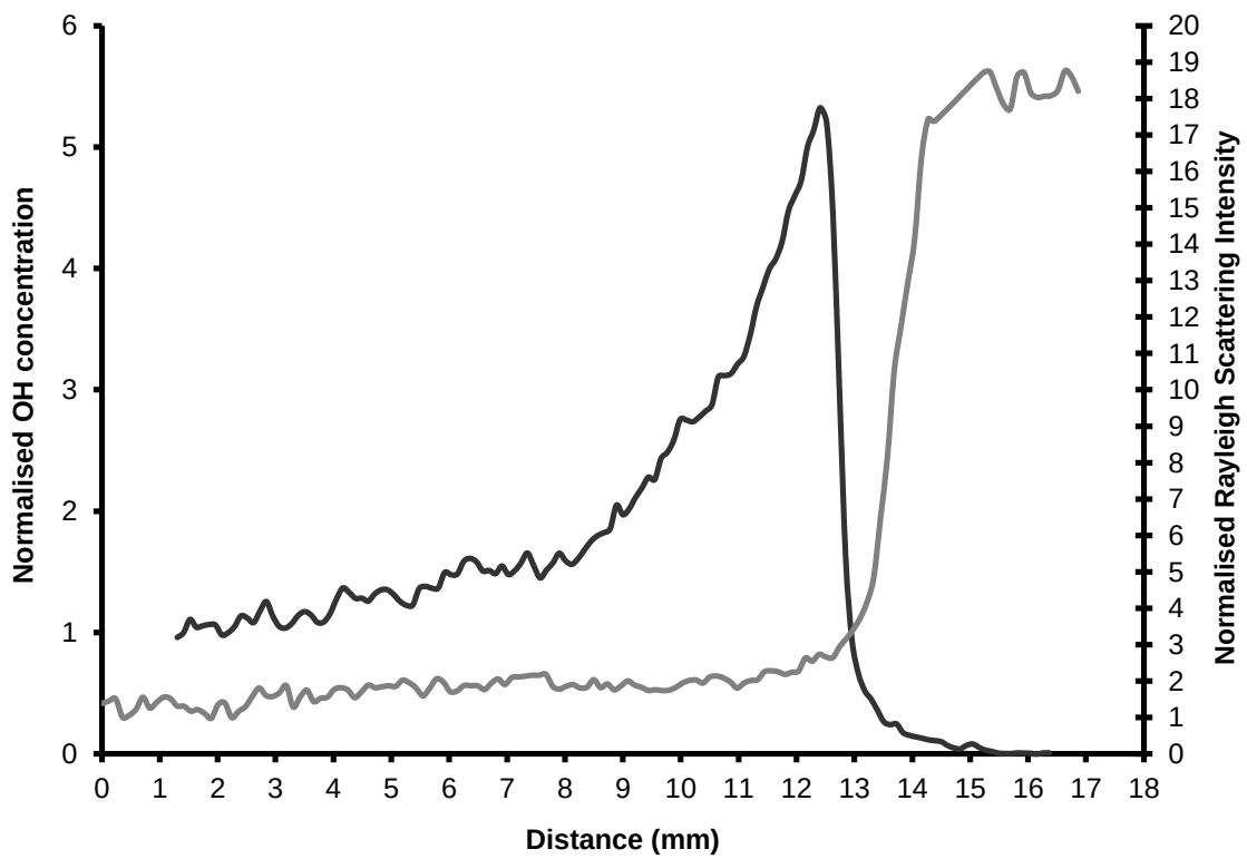
Figure 5: (a) Graph of normalised OH concentration and Rayleigh scattering intensity across a convex flame cell as a function of position.
