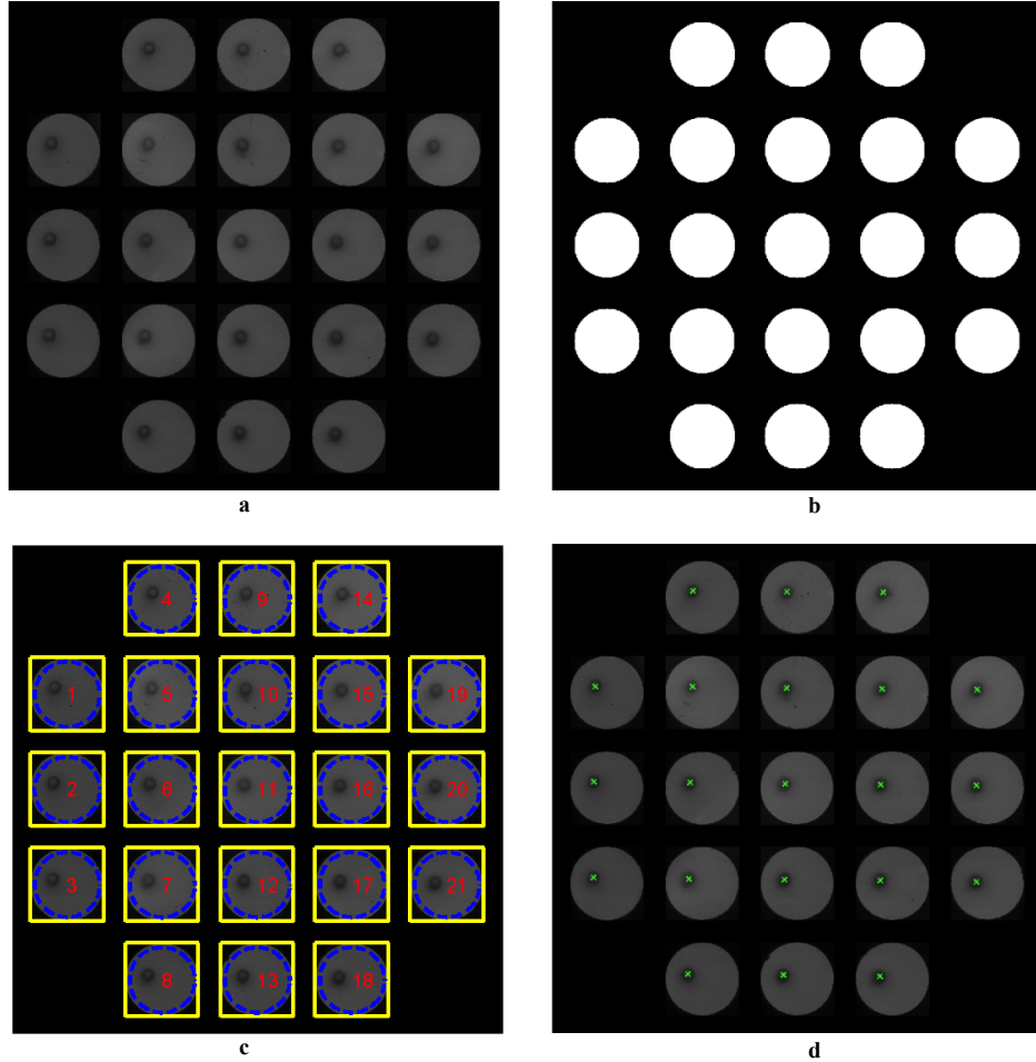
Figure 2: Image processing steps for calibration, (a) captured image (grey scaled), (b) mask of detected lens array (black-white), (c) lenses registration 1-21, visualization of their edges (yellow) and perimeters (dotted blue) highlighting the area of investigation for cross-correlation, (d) detected pillar centroids of zero deflection (green cross)
